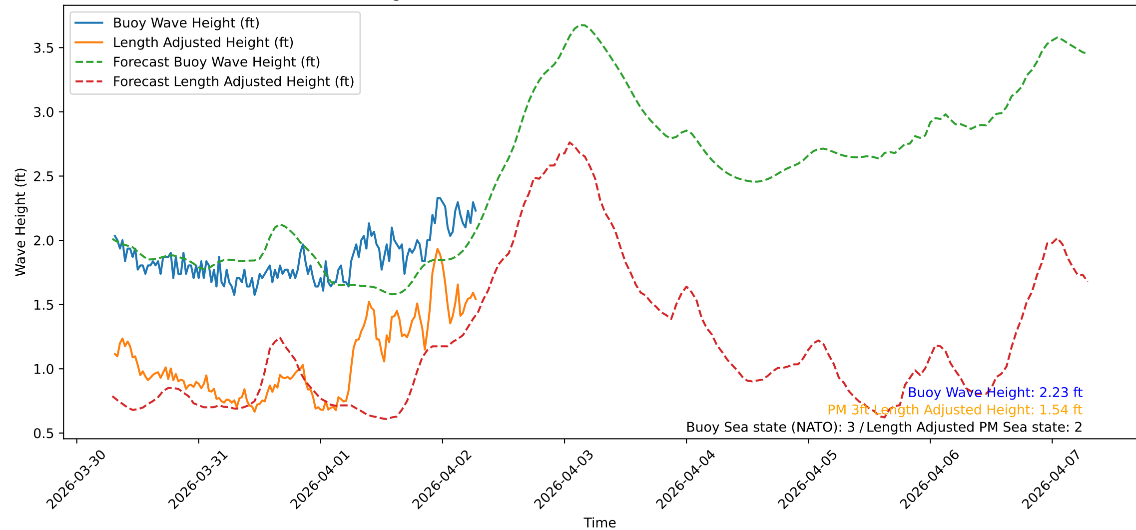
Wave Heights over Time for Oceanside Harbor at 2026-04-02 07:20:31
