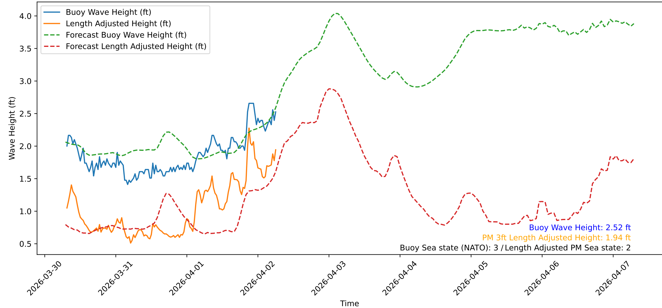
Wave Heights over Time for Green Beach at 2026-04-02 07:21:10
