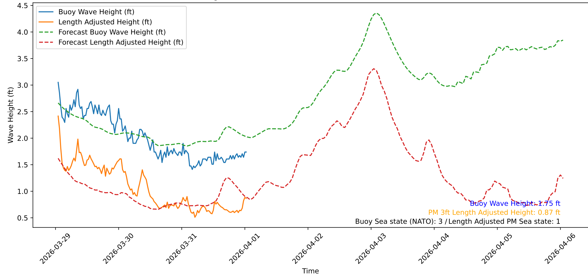
Wave Heights over Time for Green Beach at 2026-04-01 01:11:10
