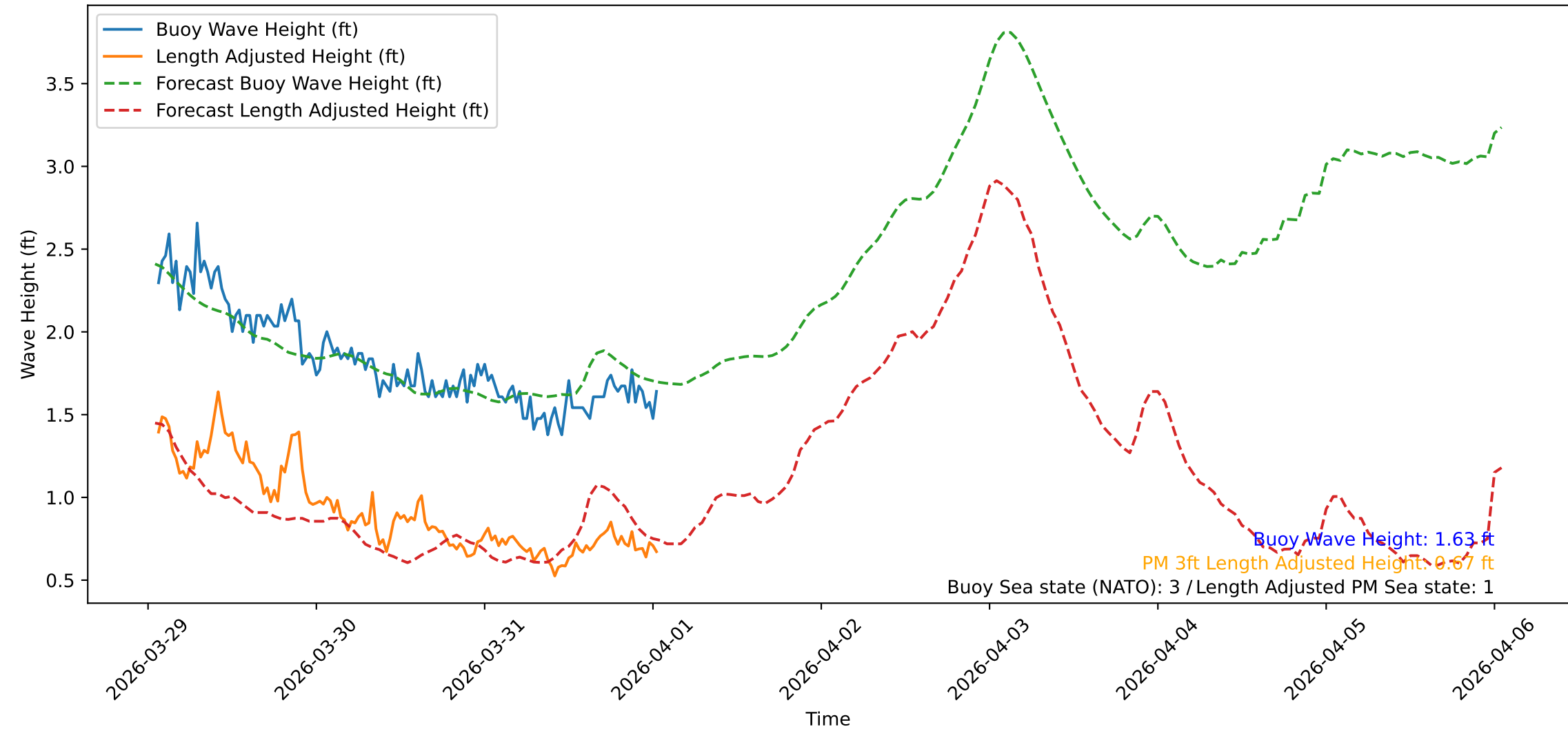
Wave Heights over Time for Red Beach at 2026-04-01 01:10:48
