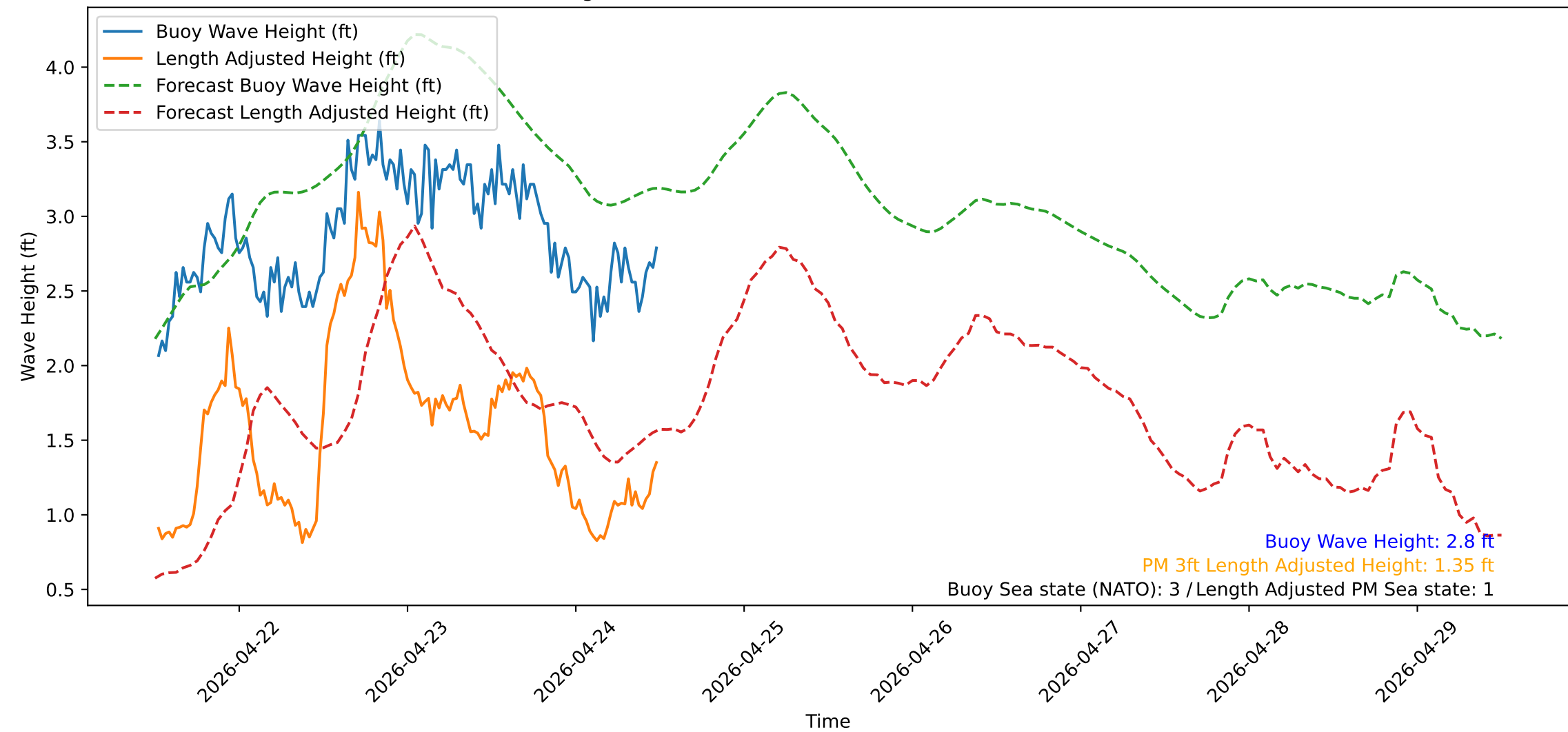
Wave Heights over Time for Red Beach at 2026-04-24 12:20:52
