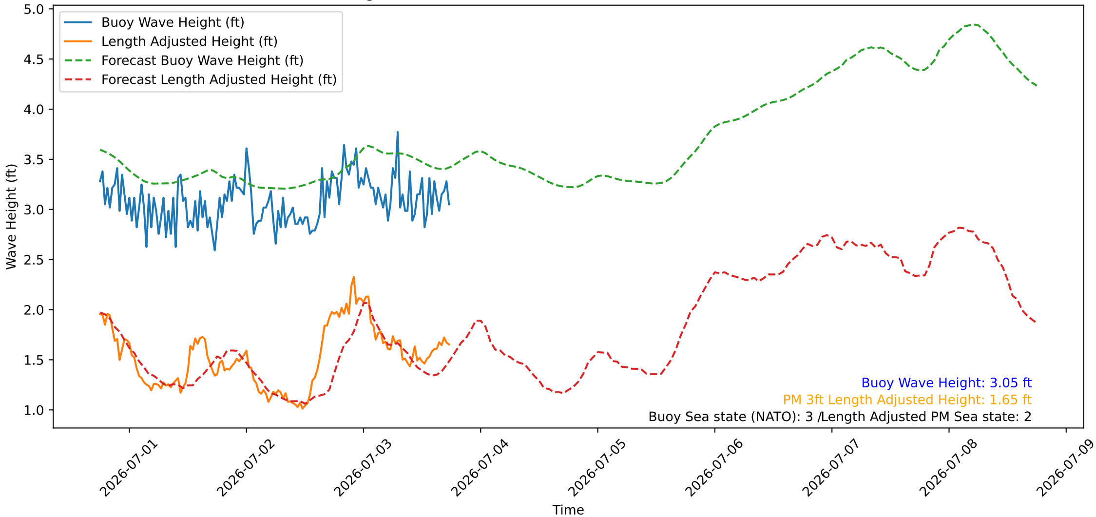
Wave Heights over Time for Oceanside Harbor at 2026-07-03 18:00:27
