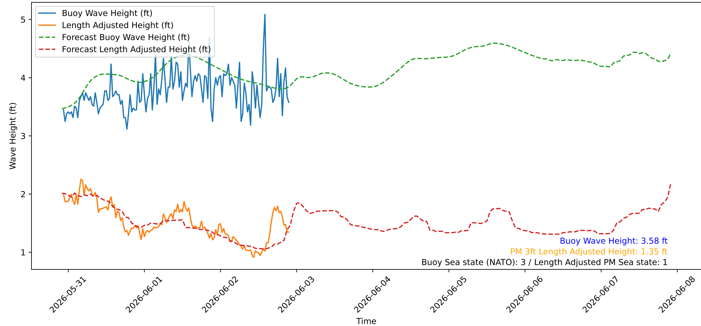
Wave Heights over Time for Oceanside Harbor at 2026-06-02 22:20:26
