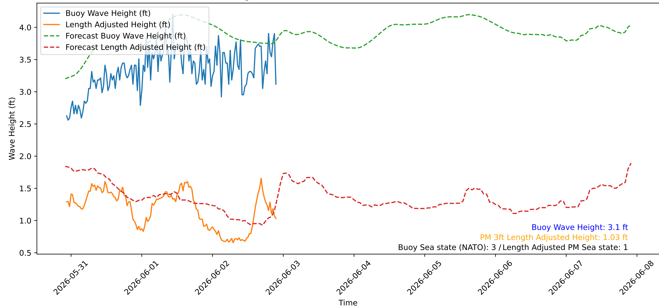
Wave Heights over Time for Red Beach at 2026-06-02 22:20:46
