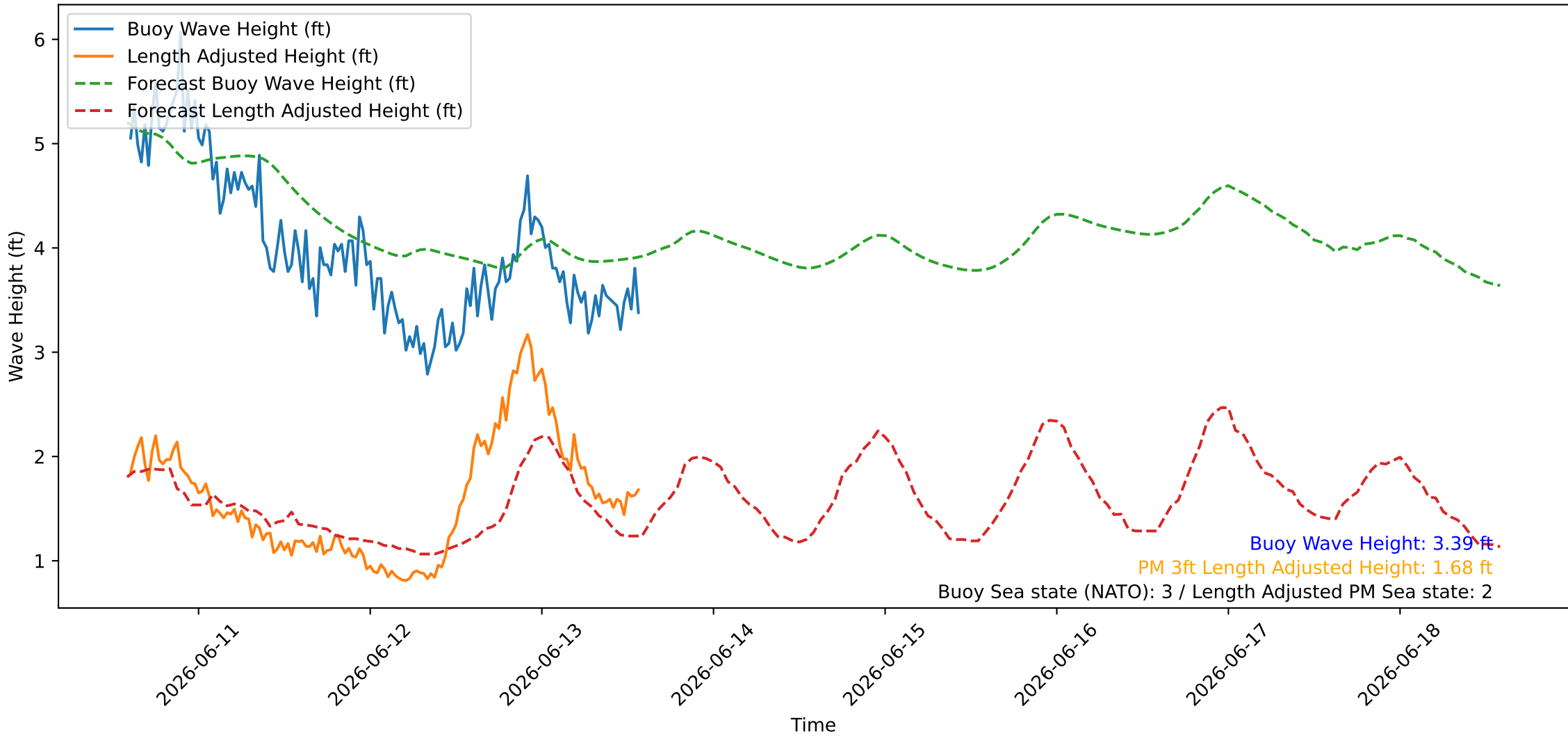
Wave Heights over Time for Oceanside Harbor at 2026-06-13 14:20:26
