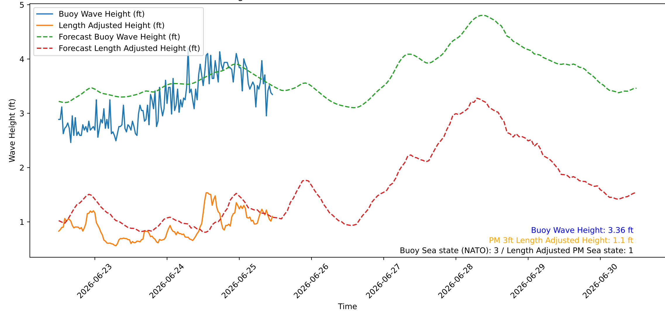
Wave Heights over Time for Green Beach at 2026-06-25 12:01:07
