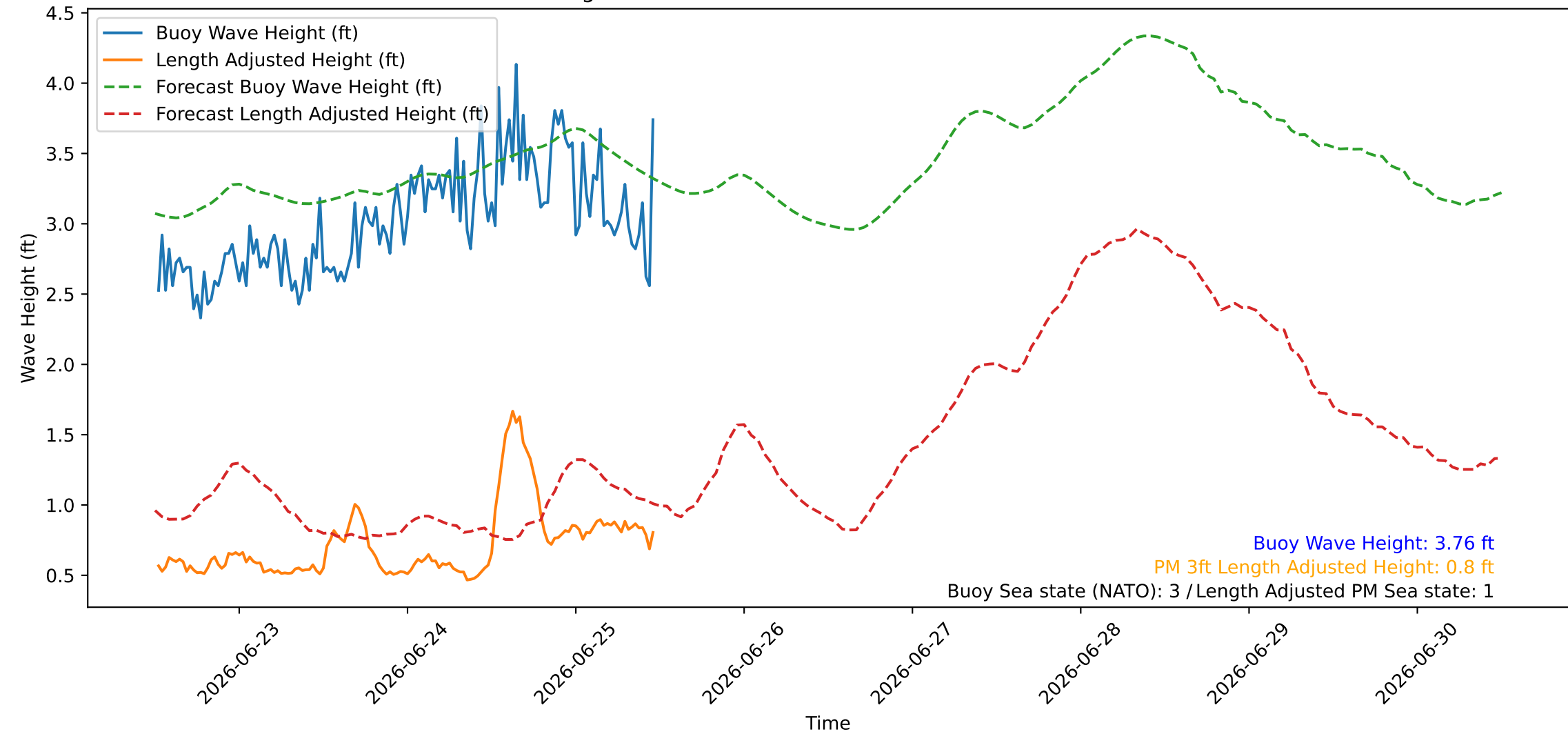
Wave Heights over Time for Red Beach at 2026-06-25 12:00:44
