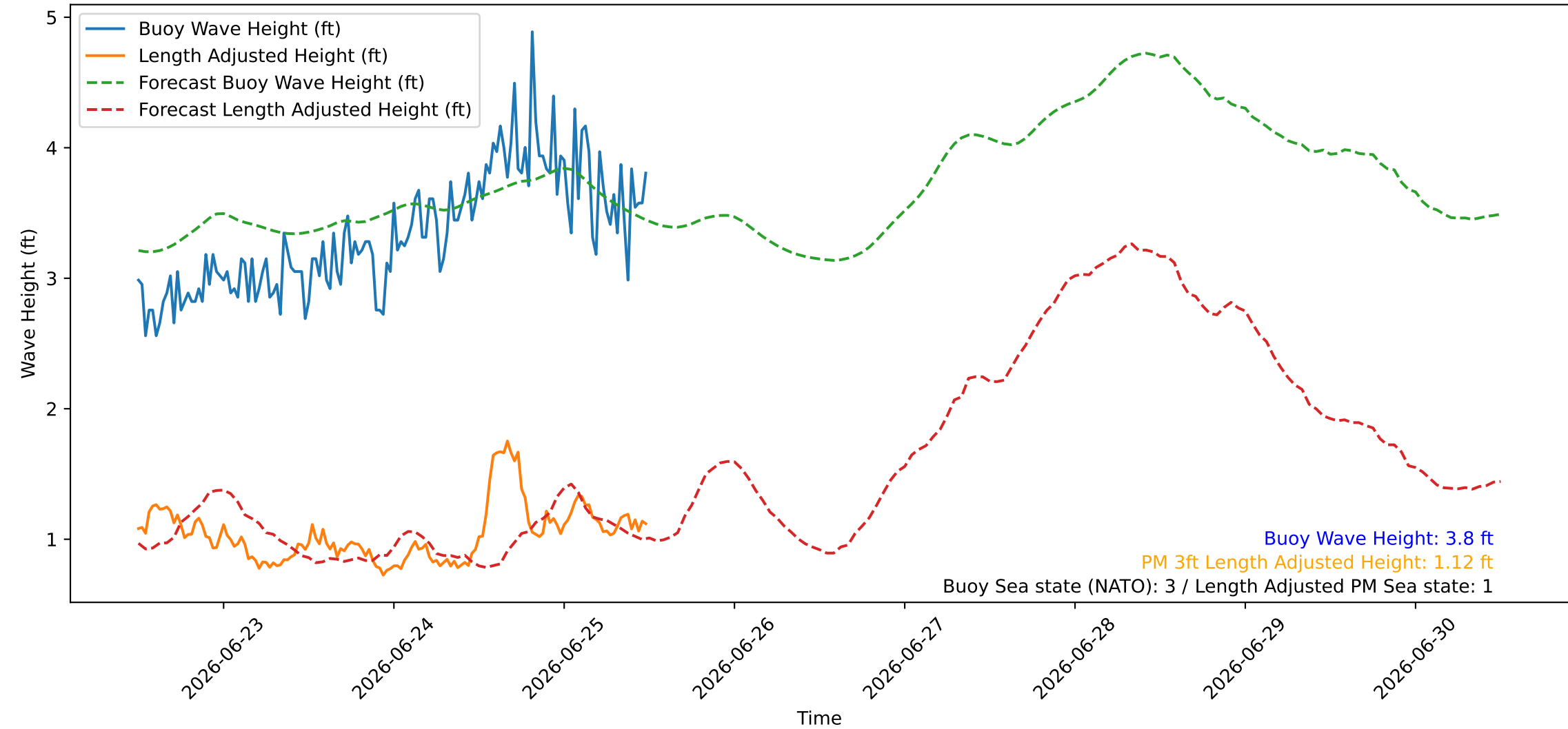
Wave Heights over Time for Oceanside Harbor at 2026-06-25 12:00:26
