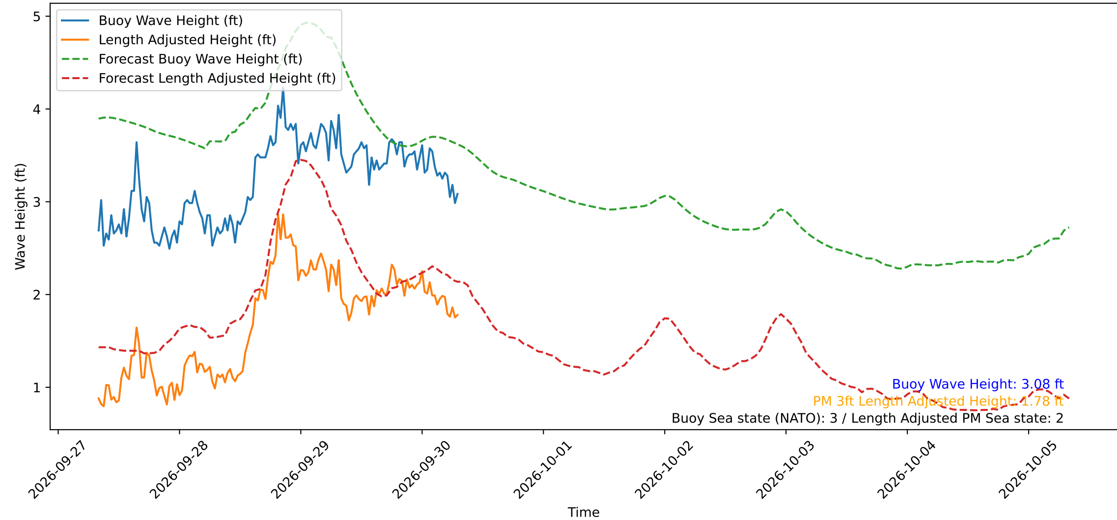
Wave Heights over Time for Oceanside Harbor at 2026-09-30 07:50:30
