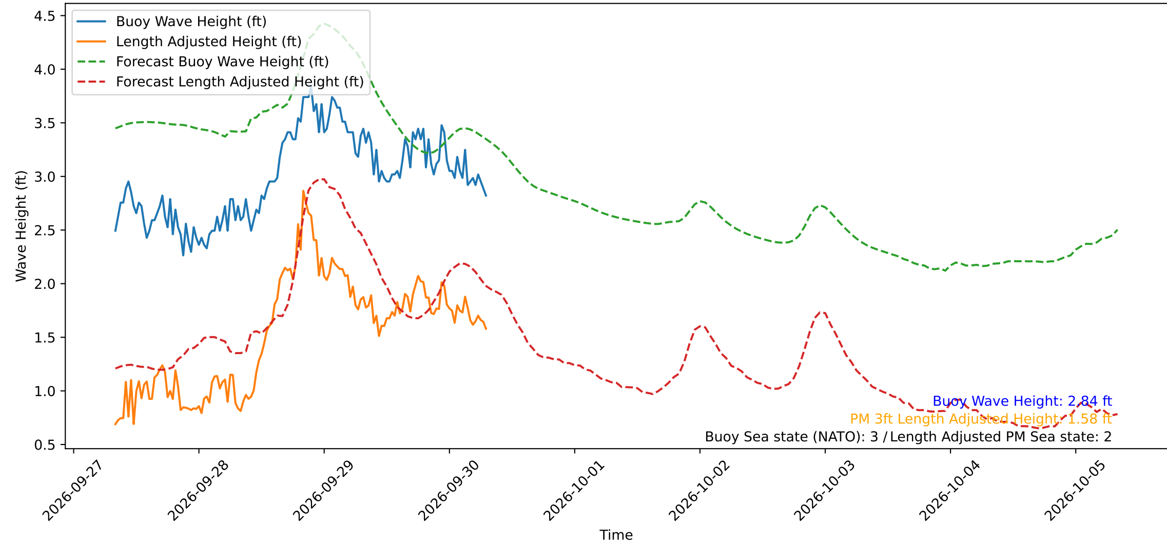
Wave Heights over Time for Red Beach at 2026-09-30 07:50:51
