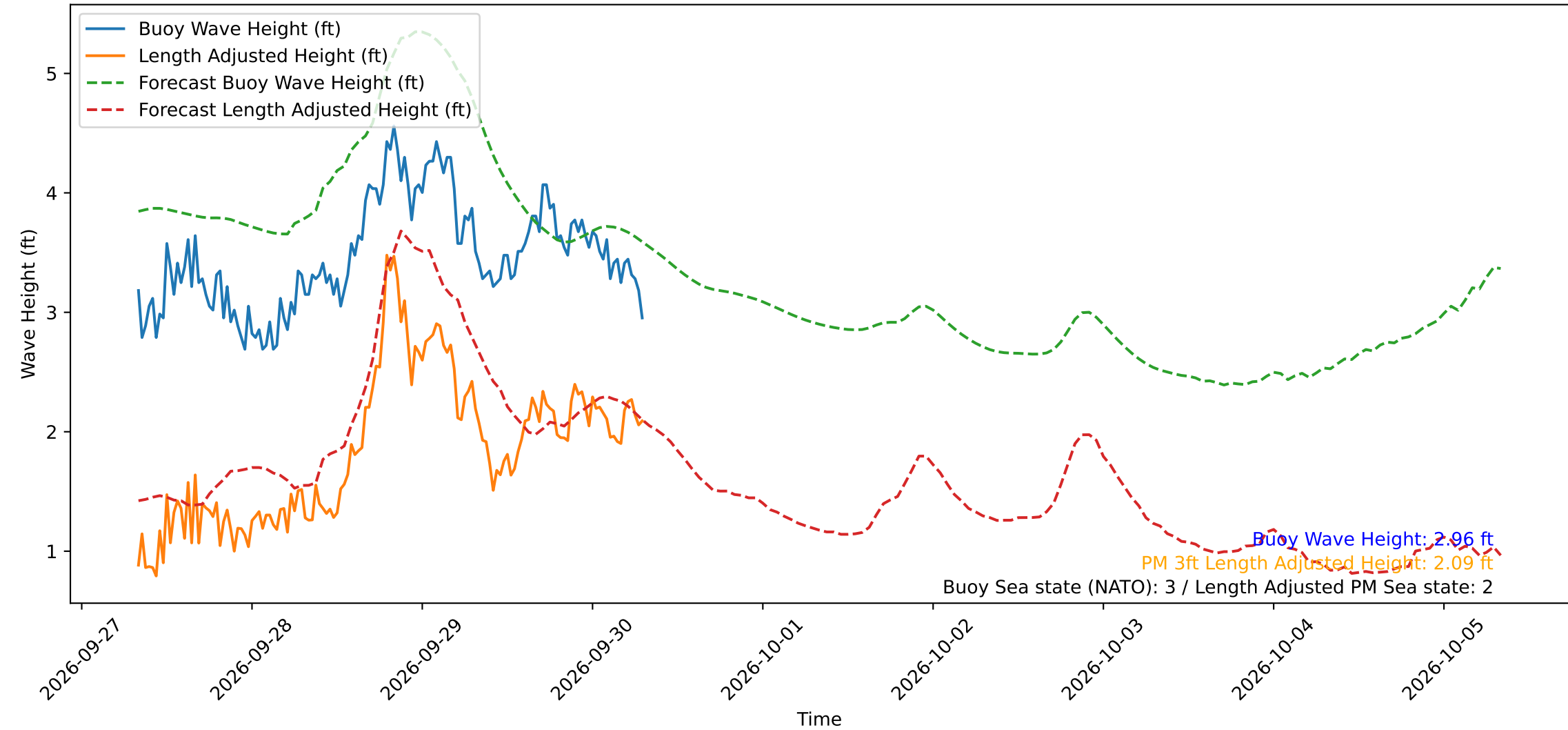
Wave Heights over Time for Green Beach at 2026-09-30 07:51:15
