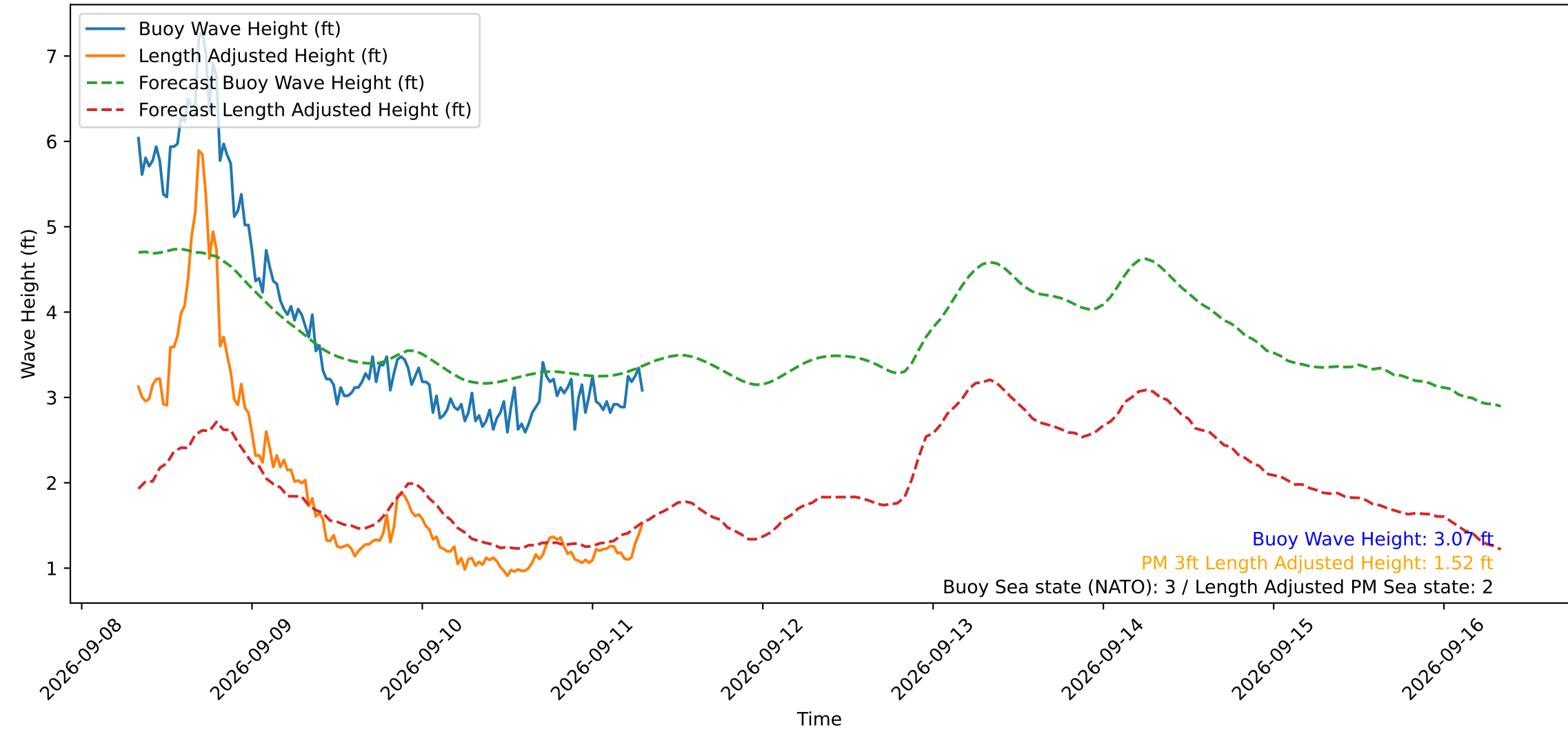
Wave Heights over Time for Green Beach at 2026-09-11 07:51:15
