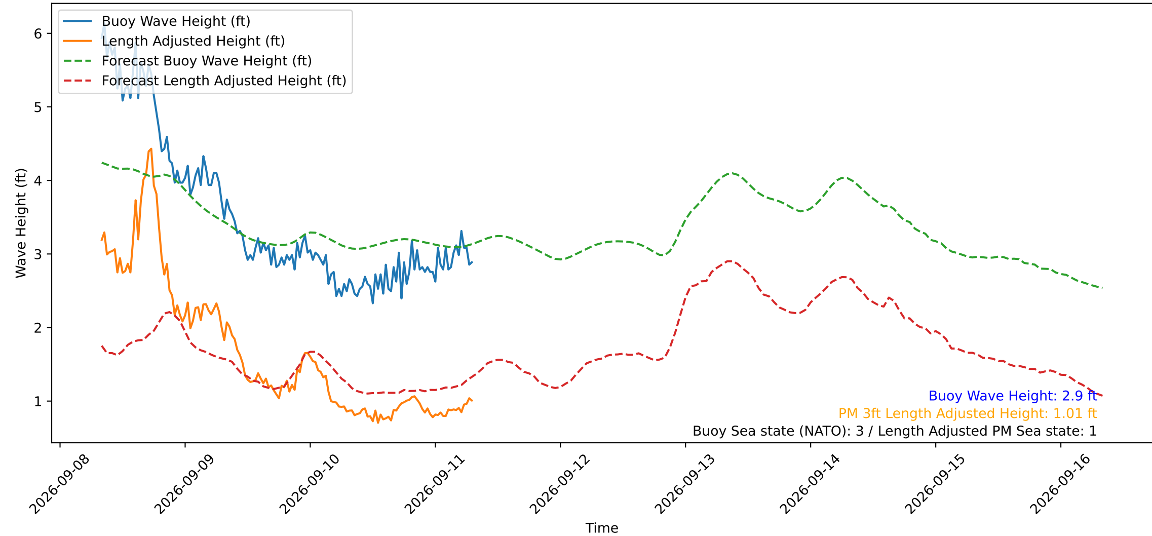
Wave Heights over Time for Red Beach at 2026-09-11 07:50:51
