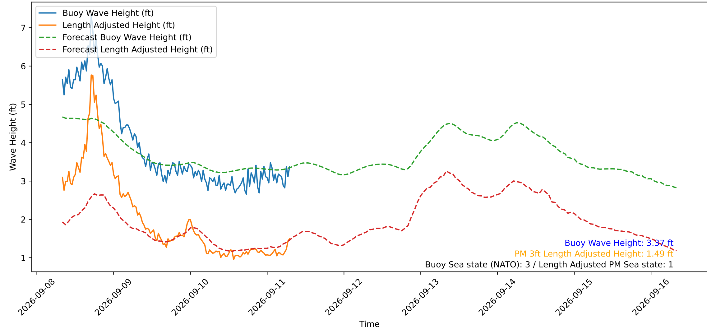
Wave Heights over Time for Oceanside Harbor at 2026-09-11 07:50:30
