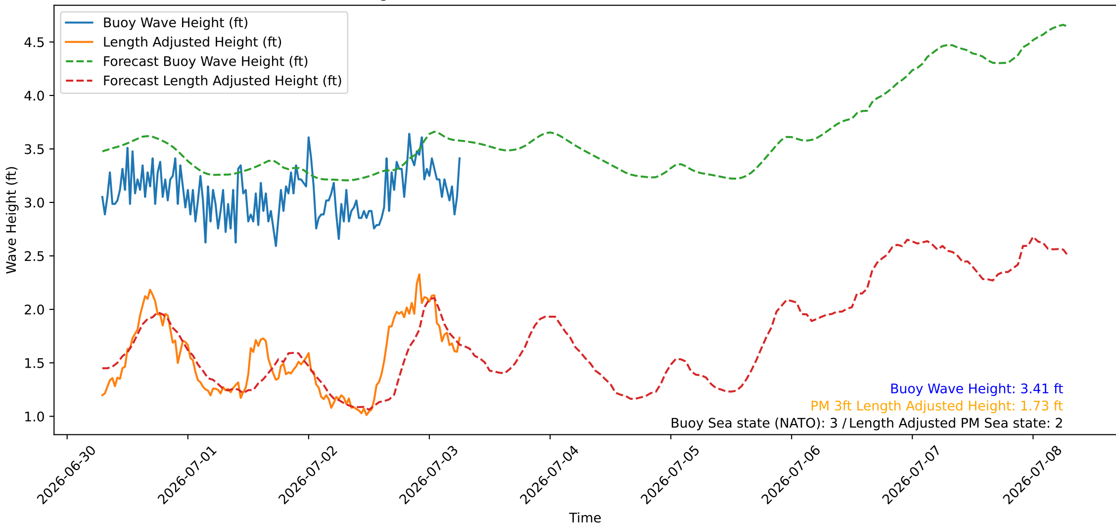
Wave Heights over Time for Oceanside Harbor at 2026-07-03 06:50:26
