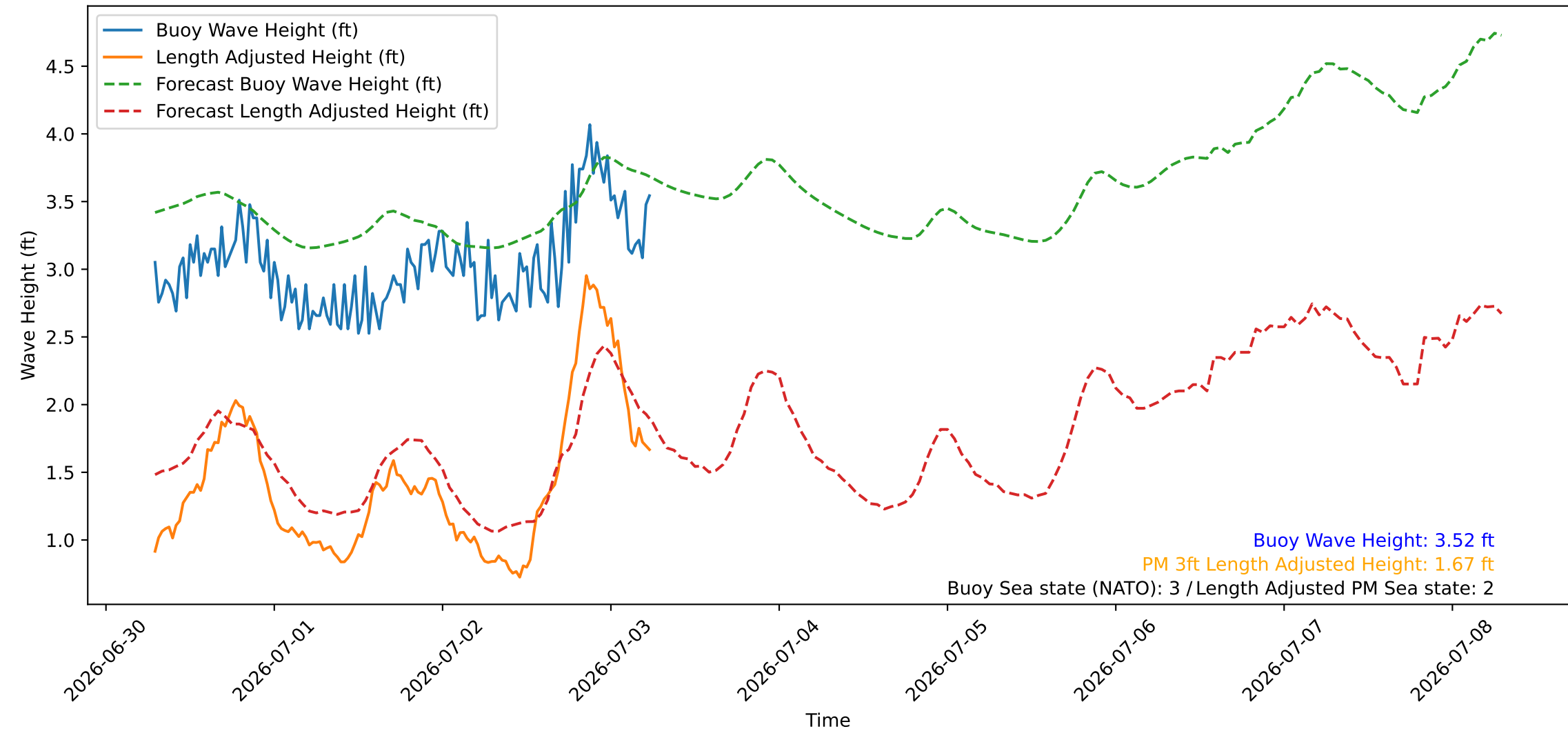
Wave Heights over Time for Green Beach at 2026-07-03 06:51:08
