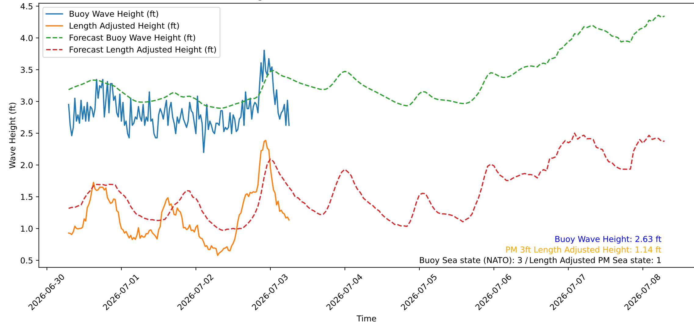
Wave Heights over Time for Red Beach at 2026-07-03 06:50:46
