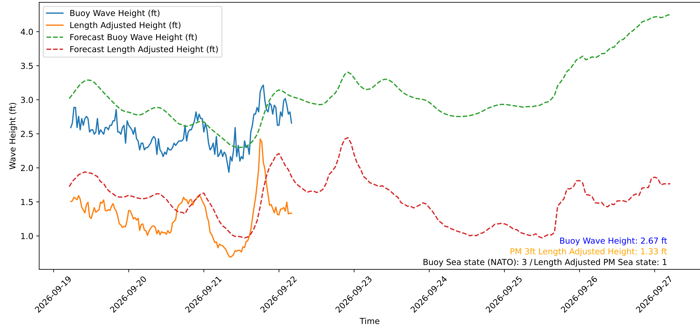
Wave Heights over Time for Green Beach at 2026-09-22 05:01:12
