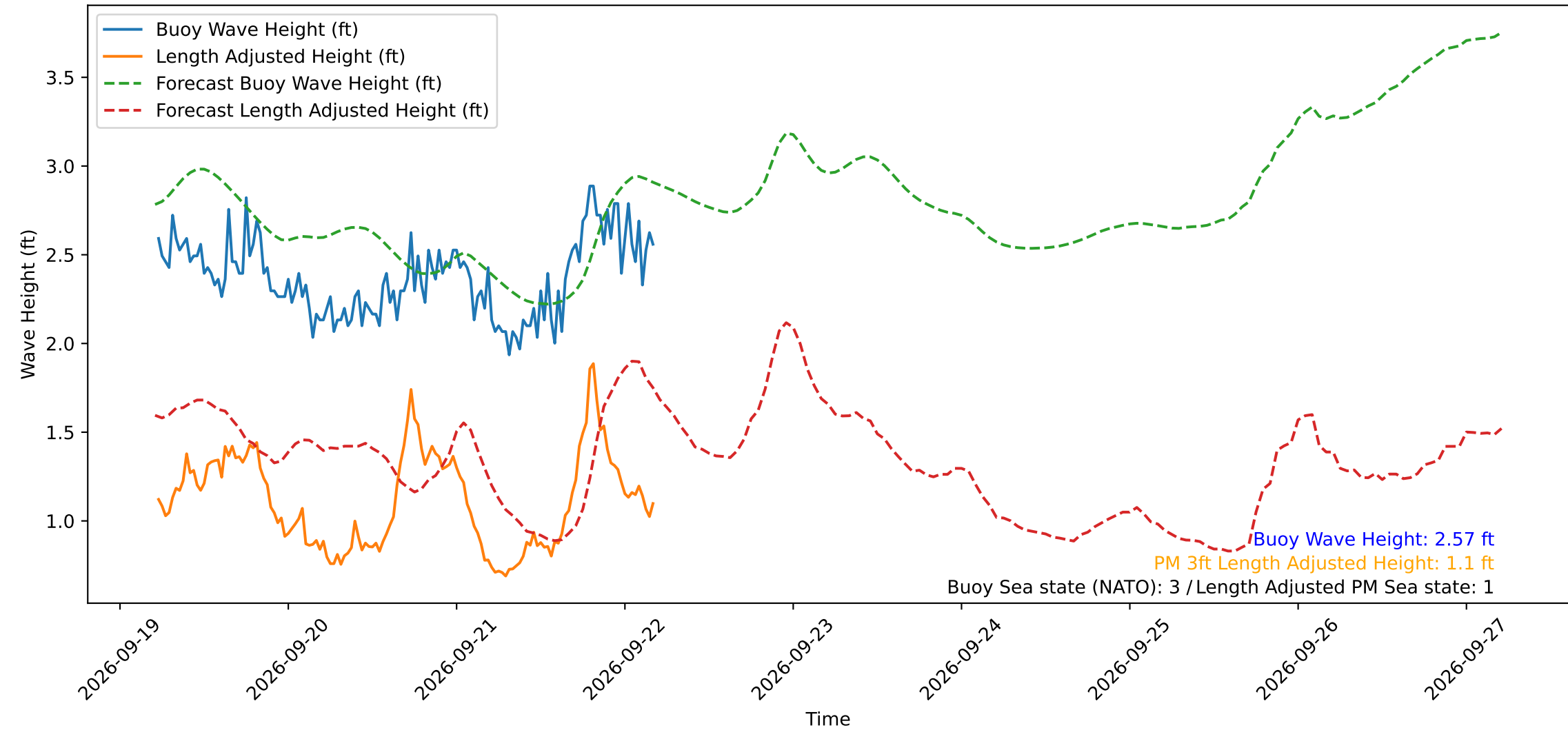
Wave Heights over Time for Red Beach at 2026-09-22 05:00:49
