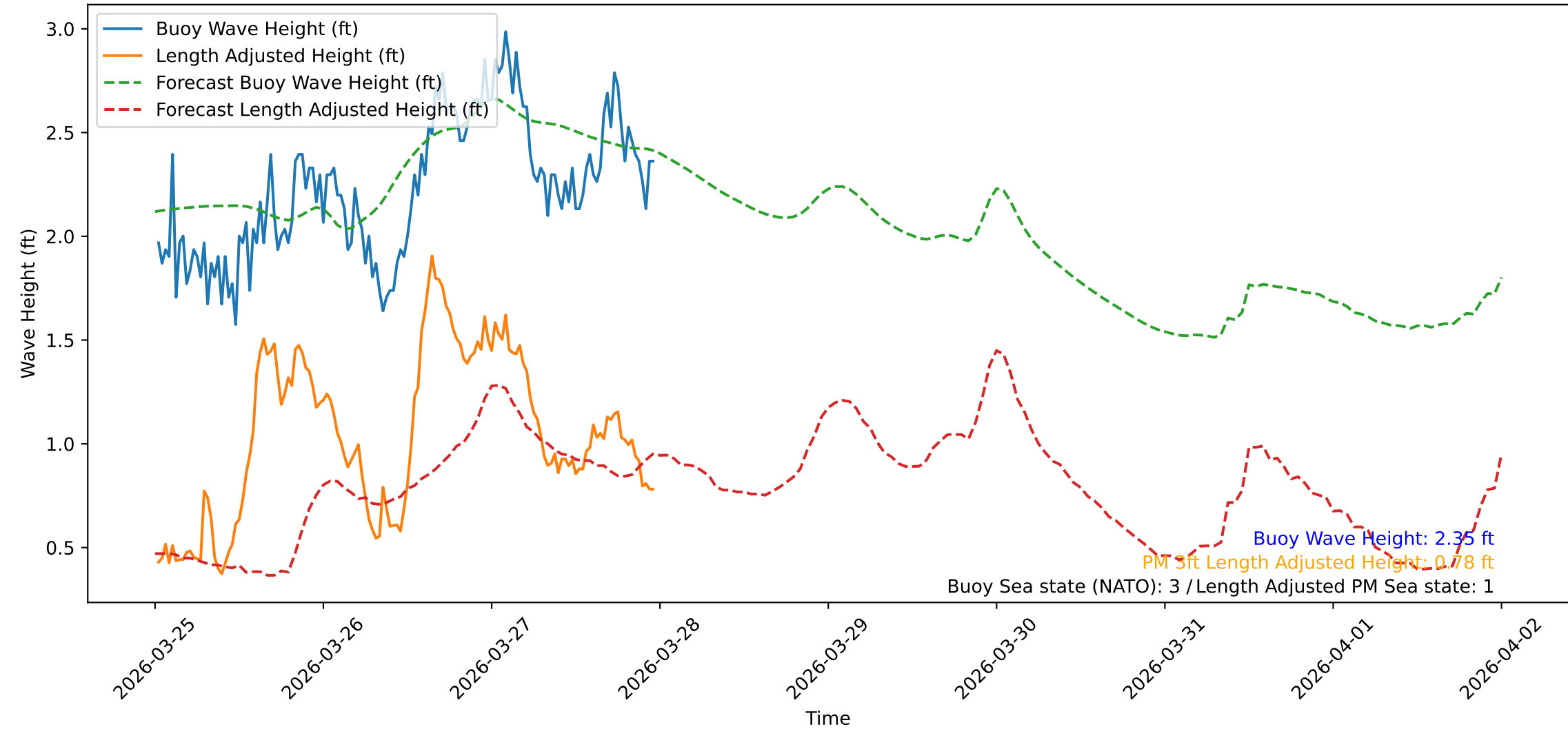
Wave Heights over Time for Red Beach at 2026-03-28 00:00:47
