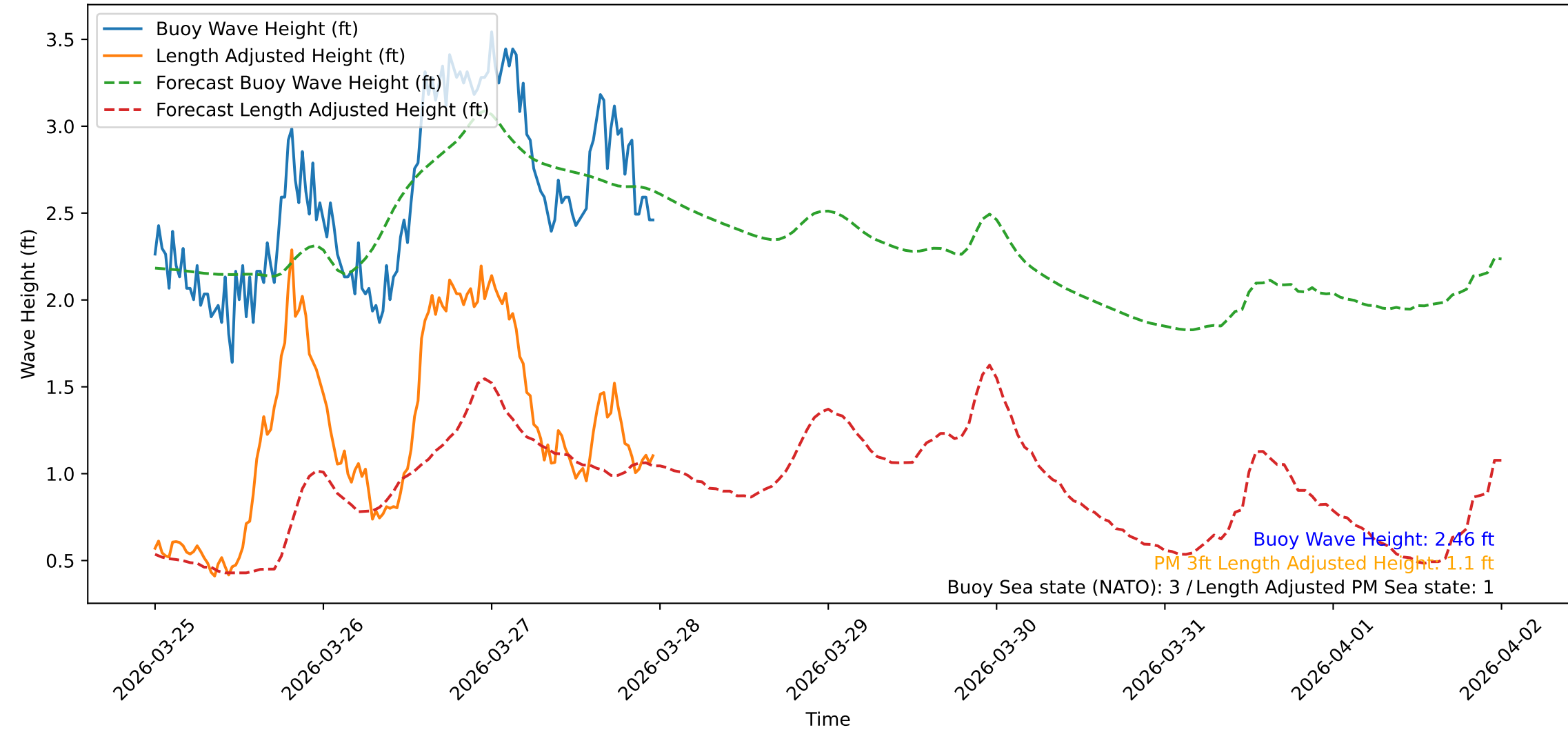
Wave Heights over Time for Green Beach at 2026-03-28 00:01:10
