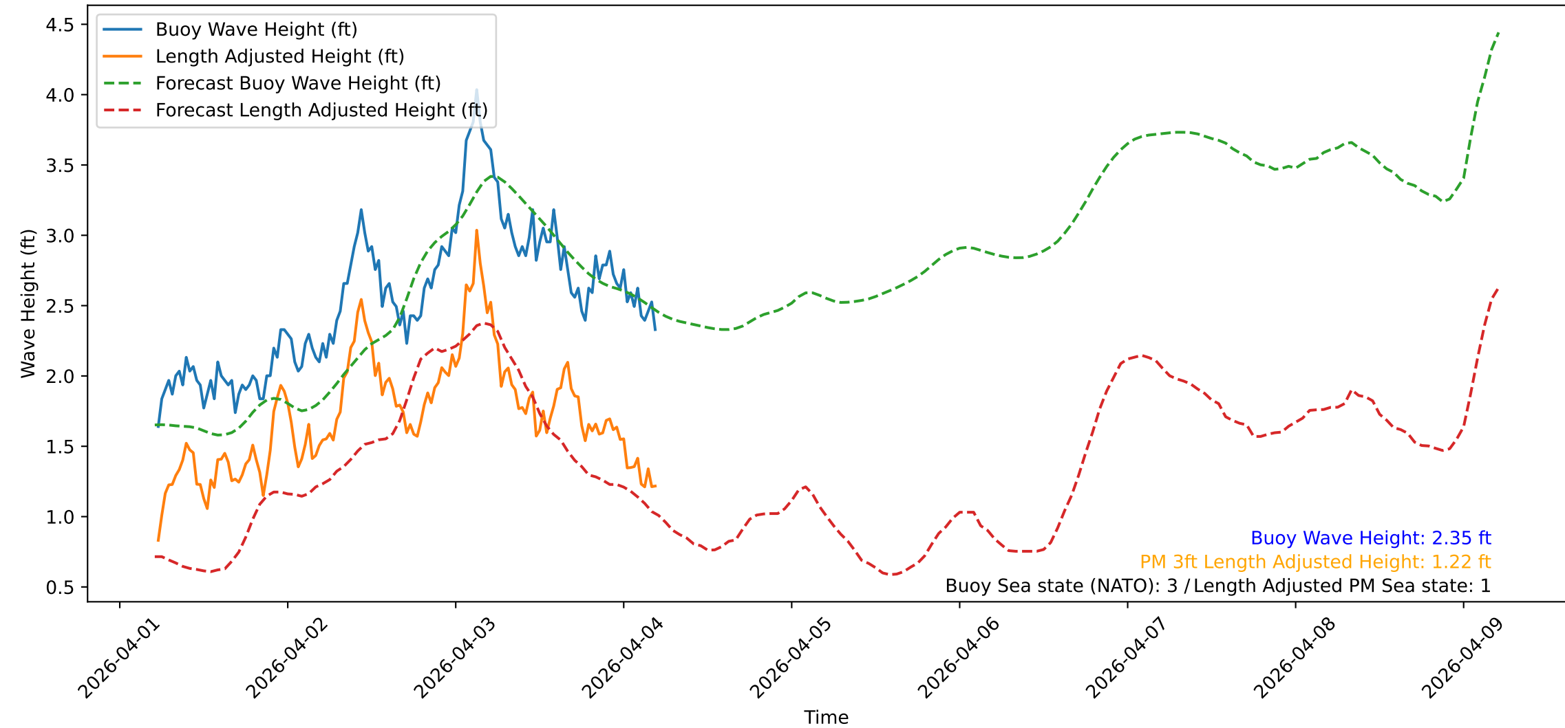
Wave Heights over Time for Oceanside Harbor at 2026-04-04 05:20:32
