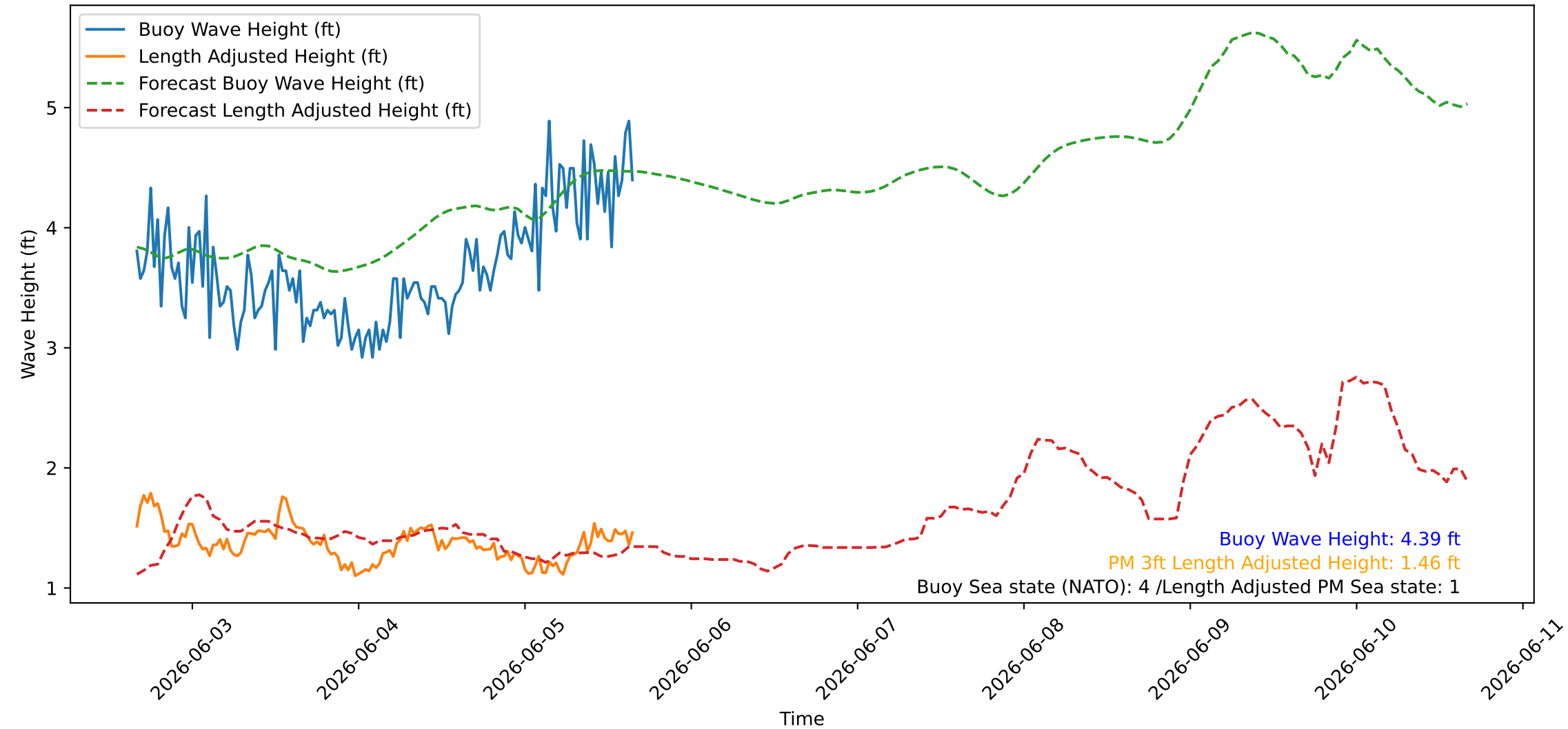
Wave Heights over Time for Oceanside Harbor at 2026-06-05 16:10:26
