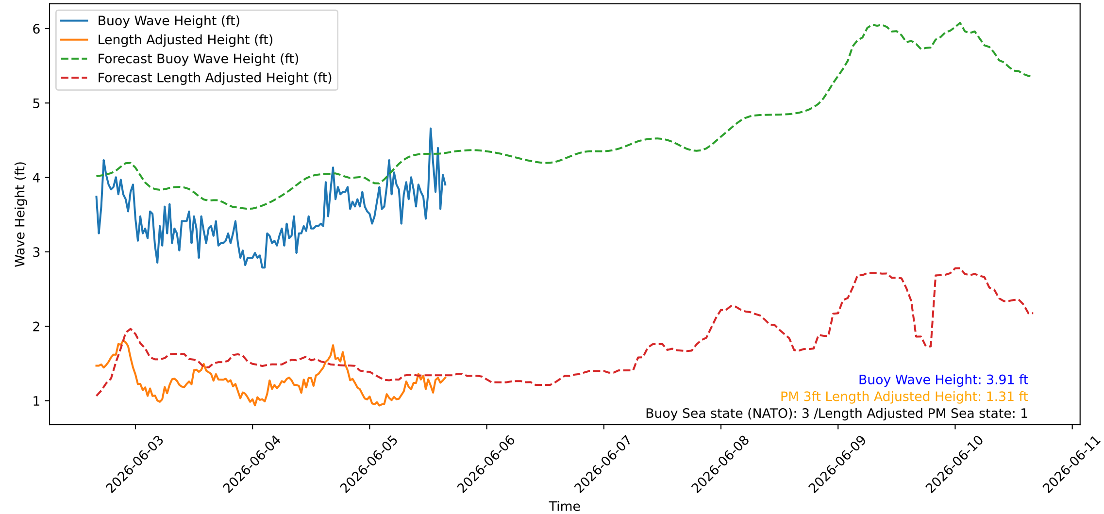
Wave Heights over Time for Green Beach at 2026-06-05 16:11:08
