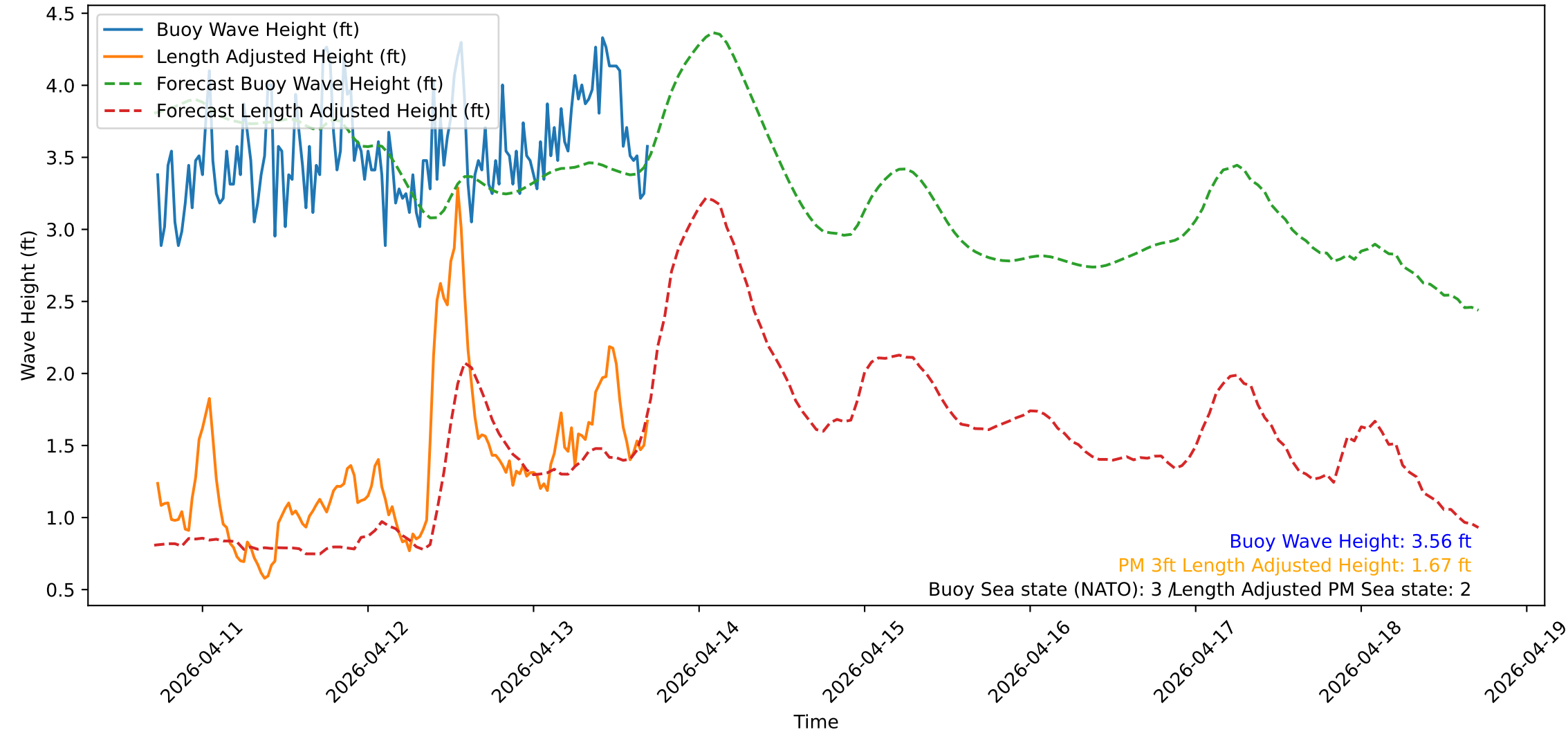
Wave Heights over Time for Red Beach at 2026-04-13 17:20:50
