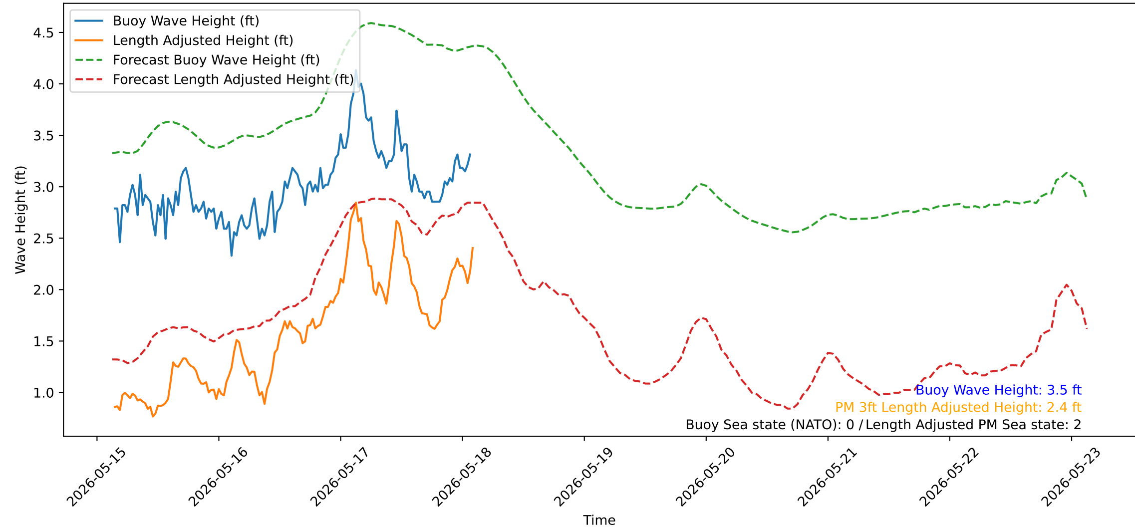
Wave Heights over Time for Red Beach at 2026-05-18 03:00:51
