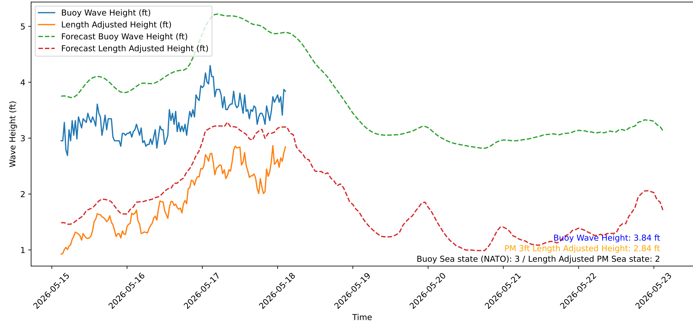
Wave Heights over Time for Oceanside Harbor at 2026-05-18 03:00:32
