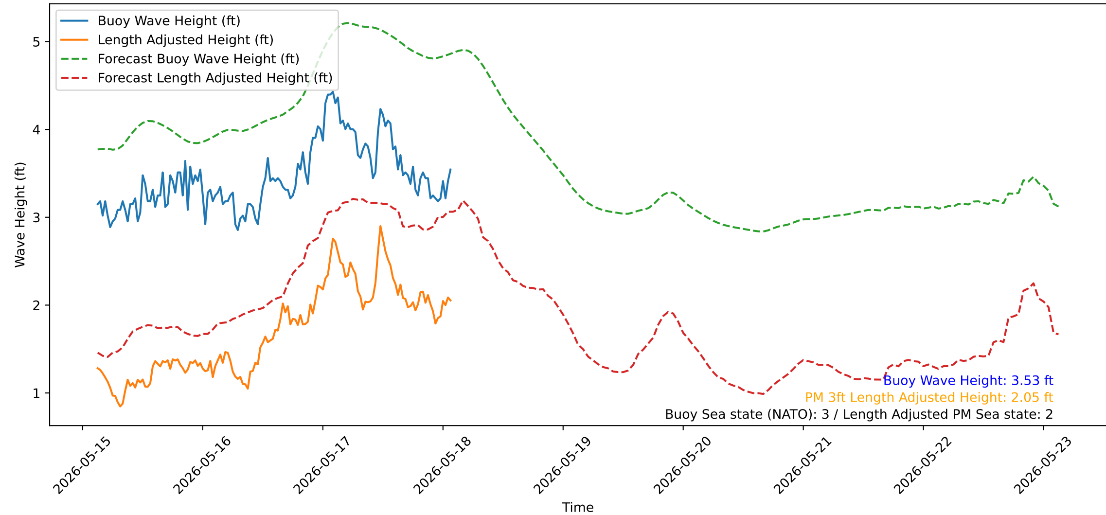
Wave Heights over Time for Green Beach at 2026-05-18 03:01:14
