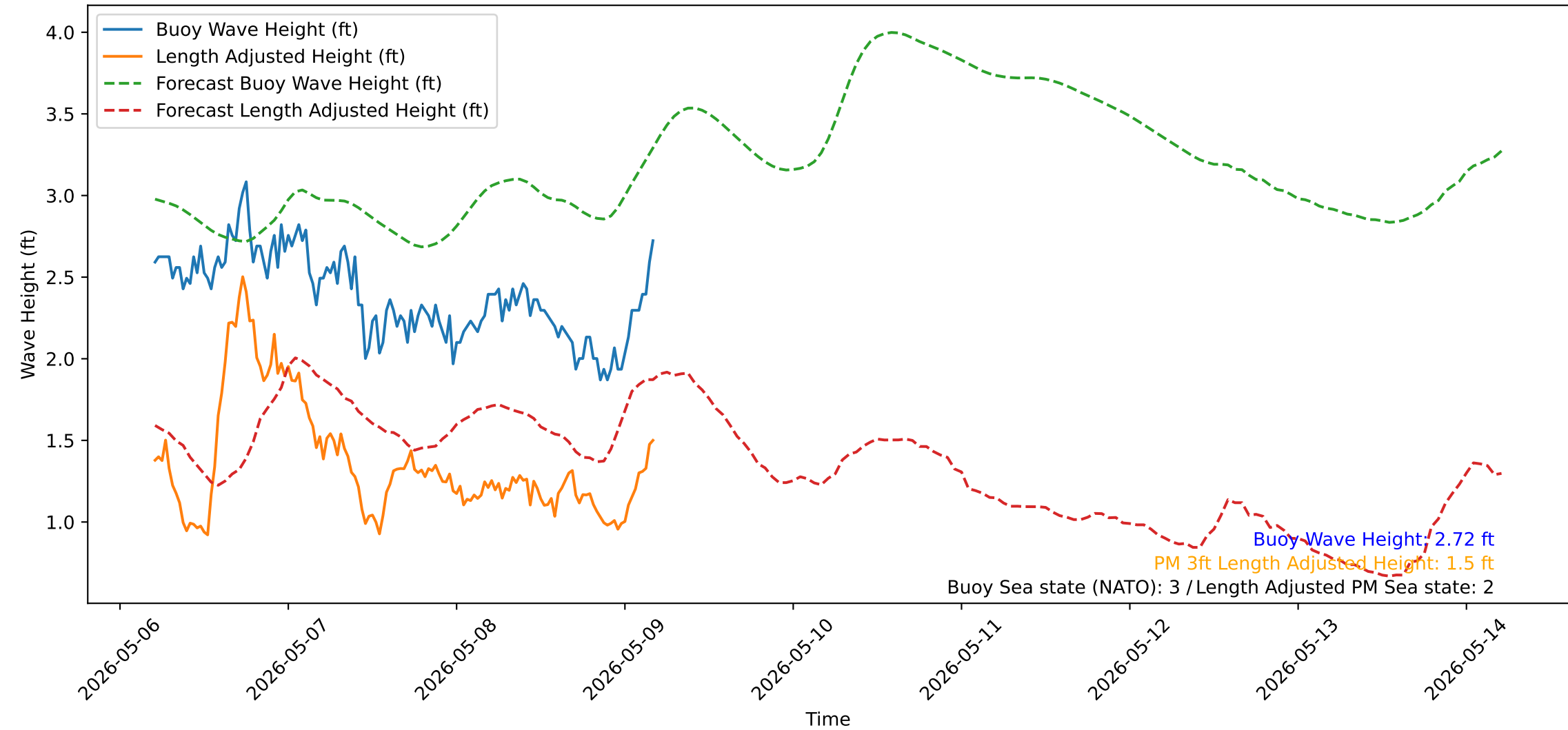
Wave Heights over Time for Oceanside Harbor at 2026-05-09 04:50:32
