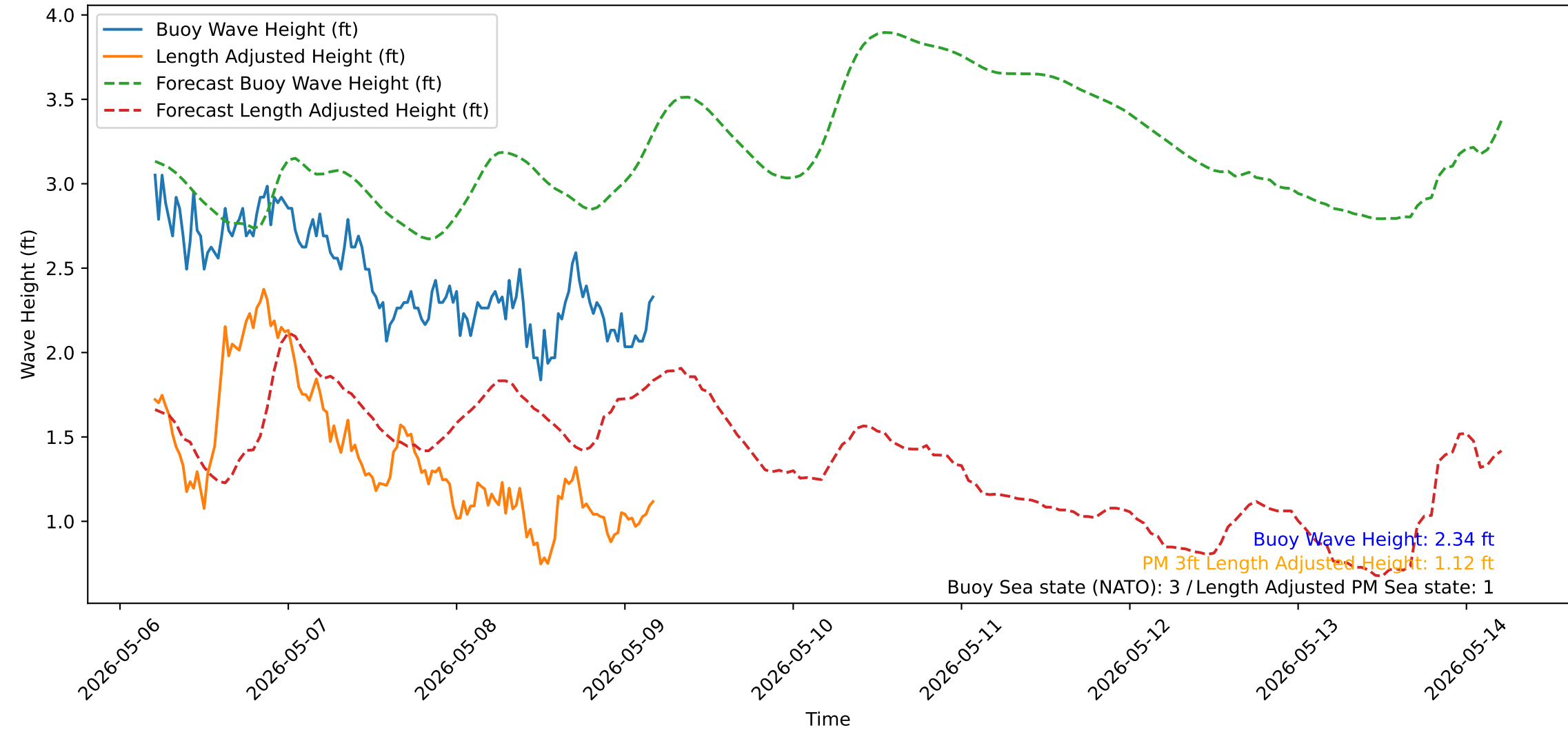
Wave Heights over Time for Green Beach at 2026-05-09 04:51:15
