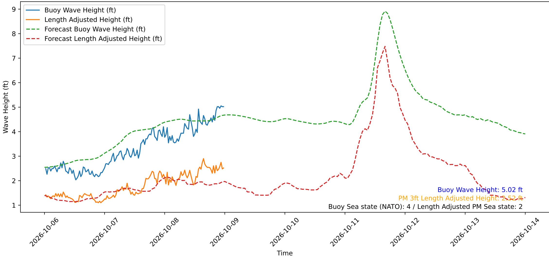
Wave Heights over Time for Oceanside Harbor at 2026-10-09 00:20:30
