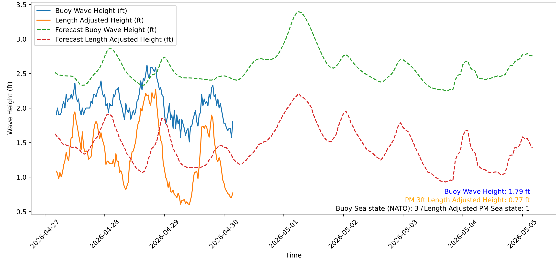
Wave Heights over Time for Red Beach at 2026-04-30 04:20:51
