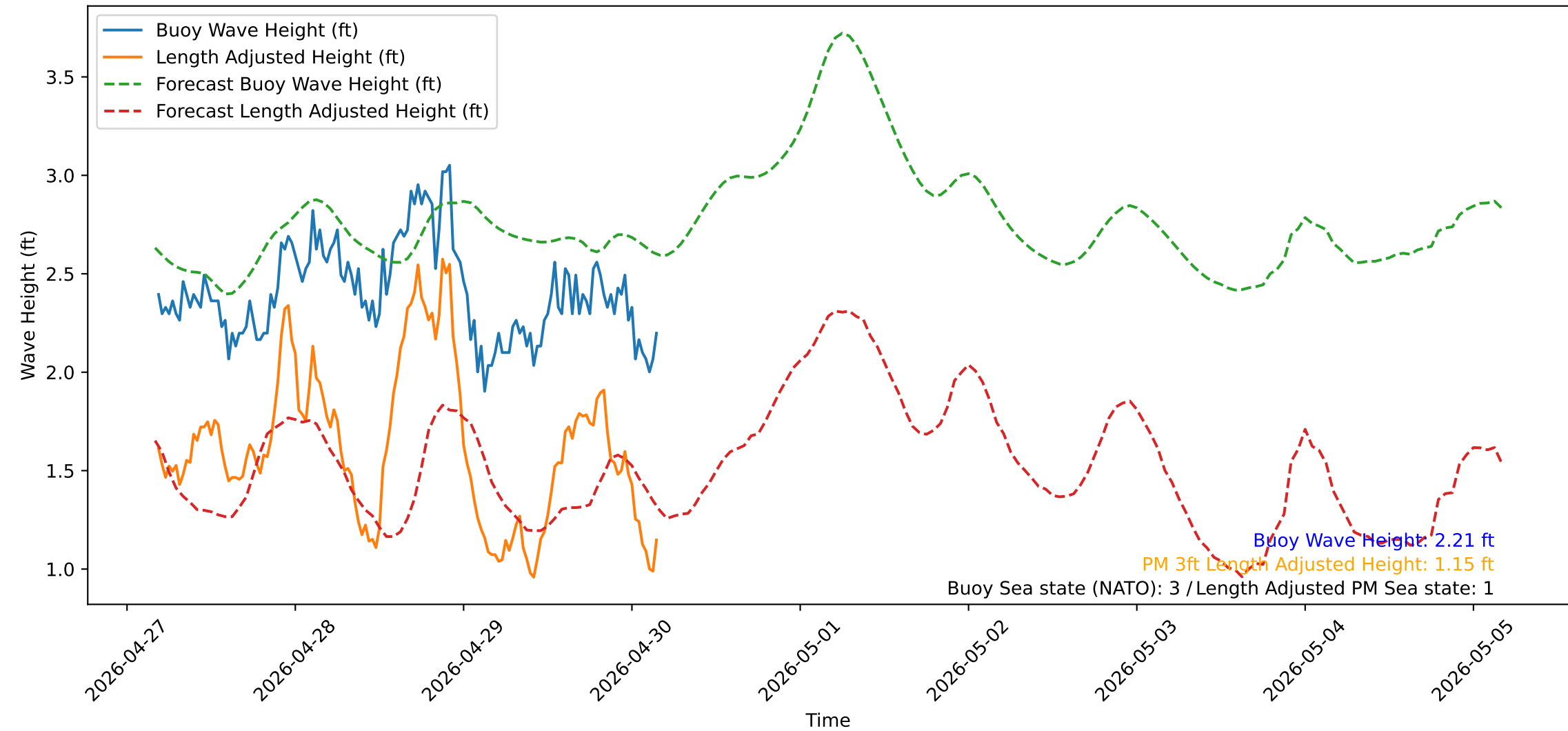
Wave Heights over Time for Oceanside Harbor at 2026-04-30 04:20:31
