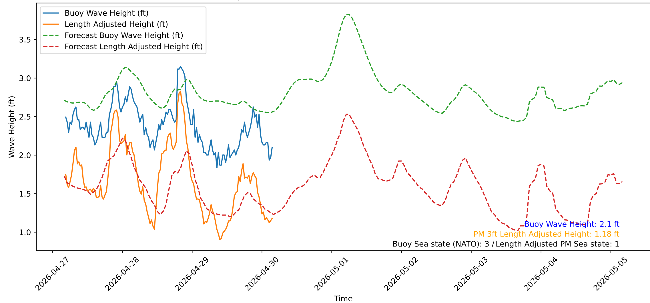
Wave Heights over Time for Green Beach at 2026-04-30 04:21:13
