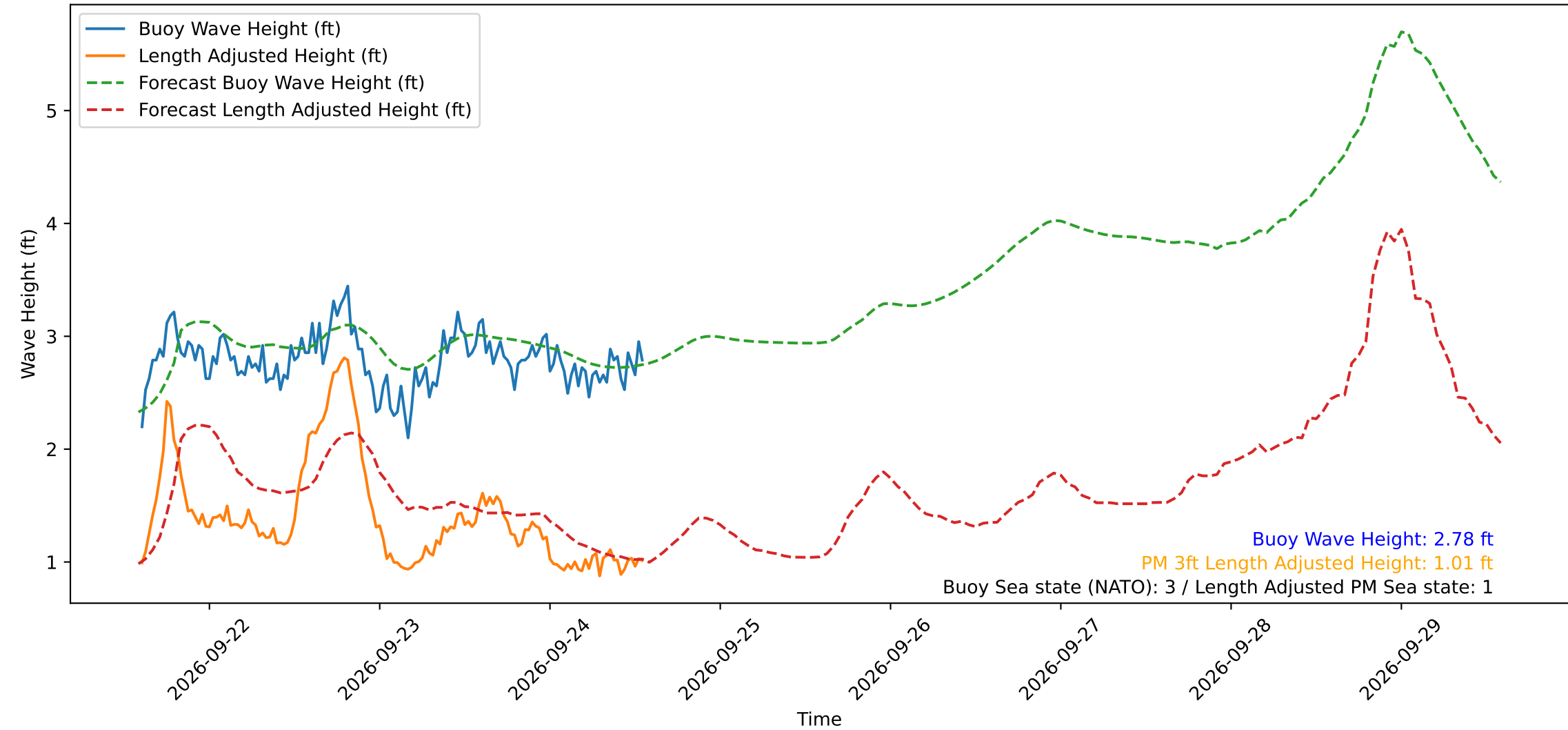
Wave Heights over Time for Green Beach at 2026-09-24 14:01:14
