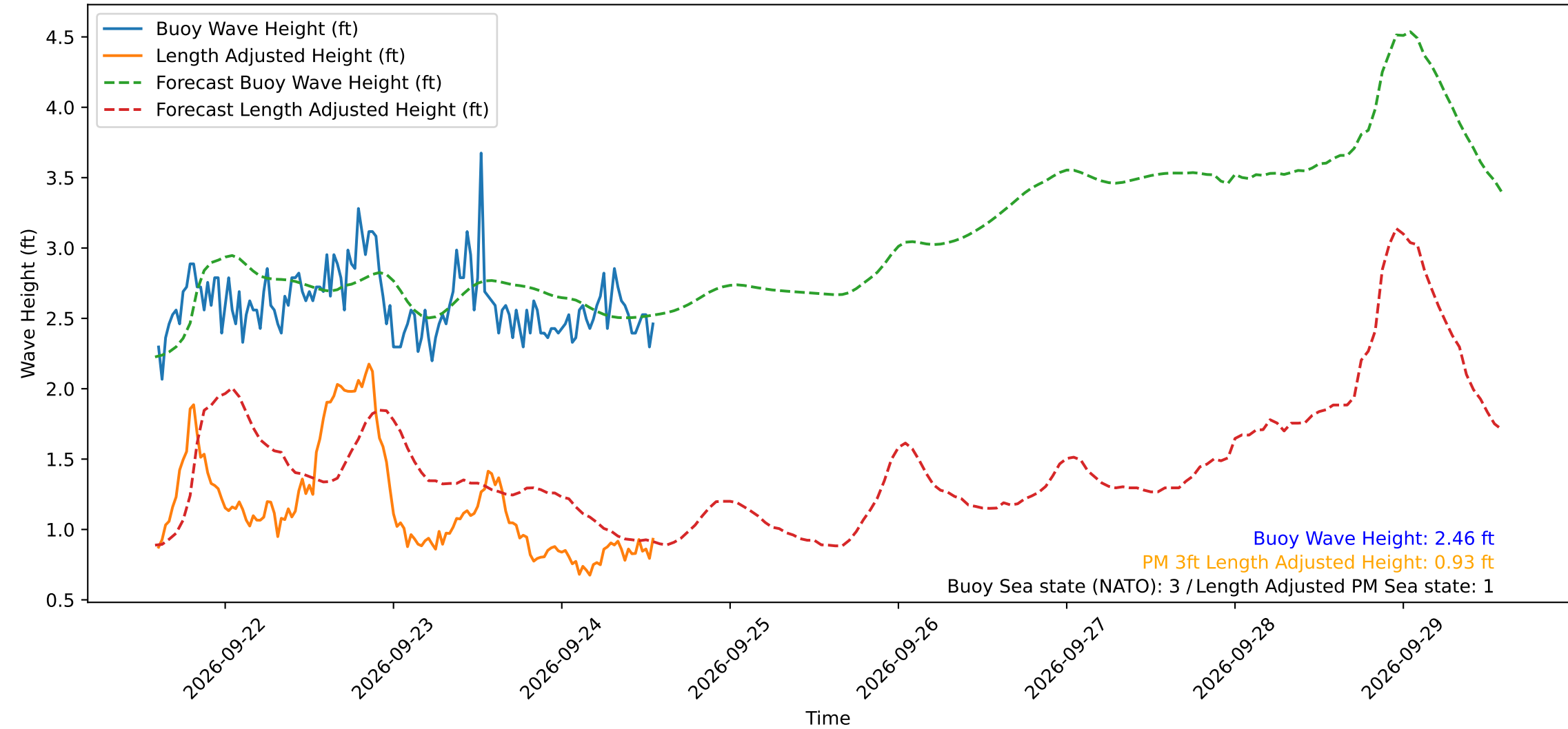
Wave Heights over Time for Red Beach at 2026-09-24 14:00:51
