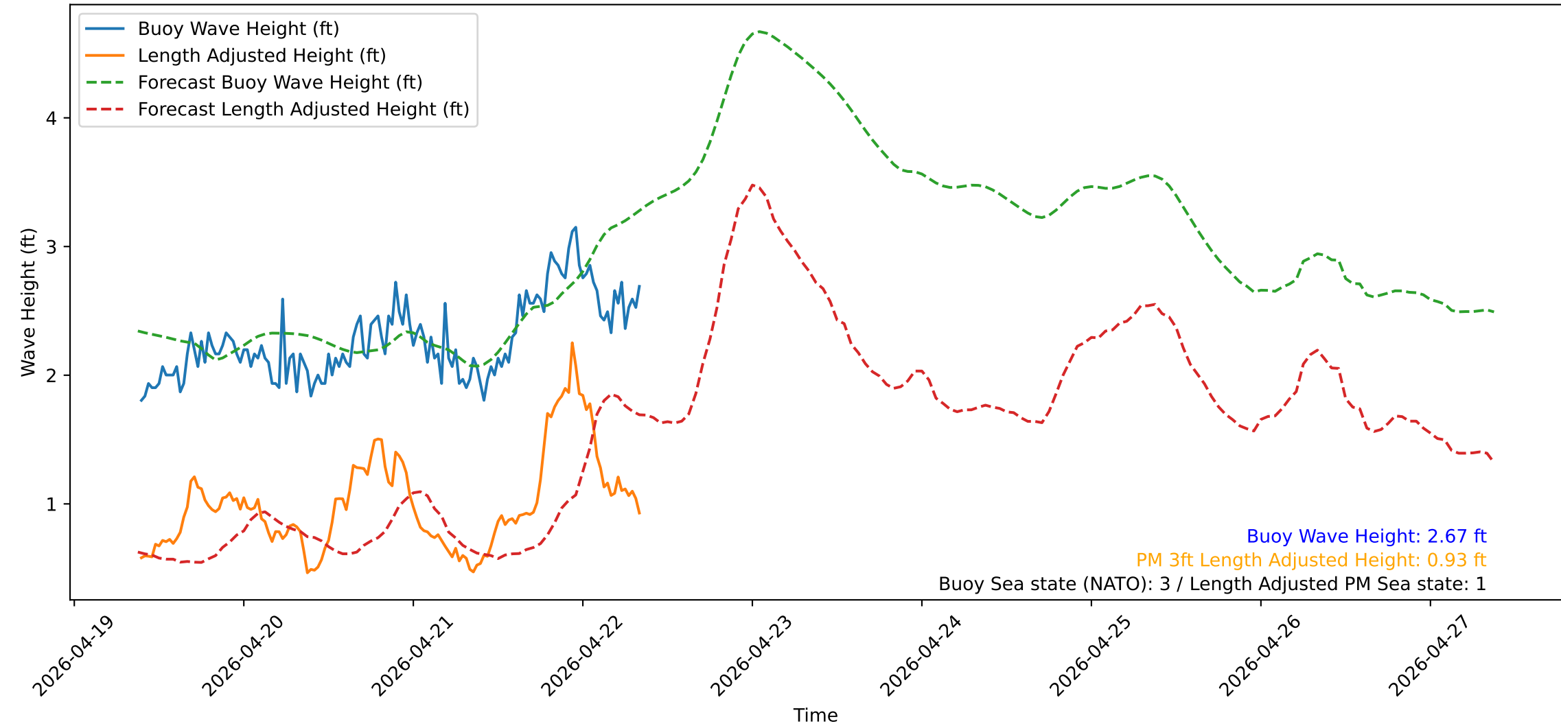
Wave Heights over Time for Red Beach at 2026-04-22 09:00:50
