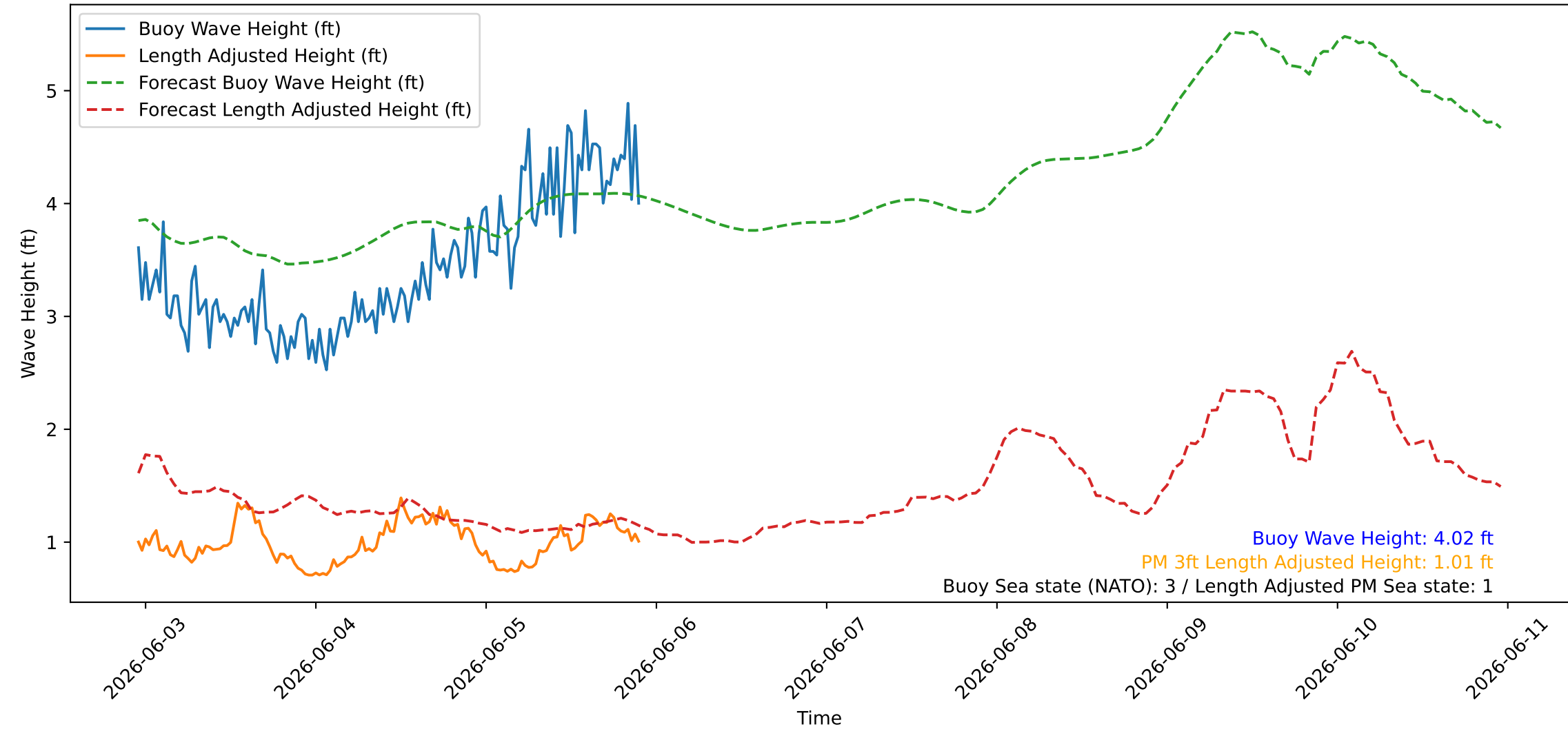
Wave Heights over Time for Red Beach at 2026-06-05 22:30:46
