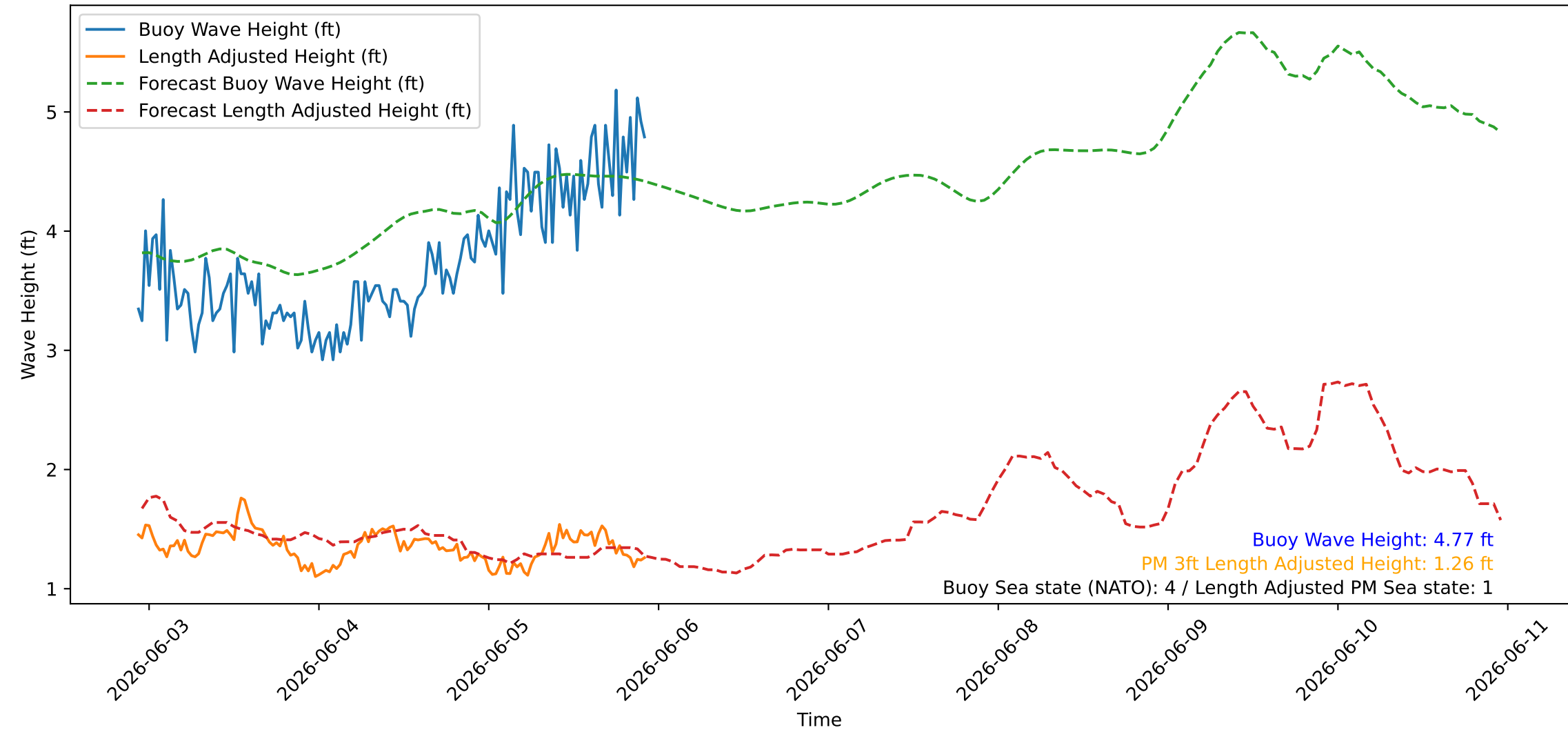
Wave Heights over Time for Oceanside Harbor at 2026-06-05 22:30:26
