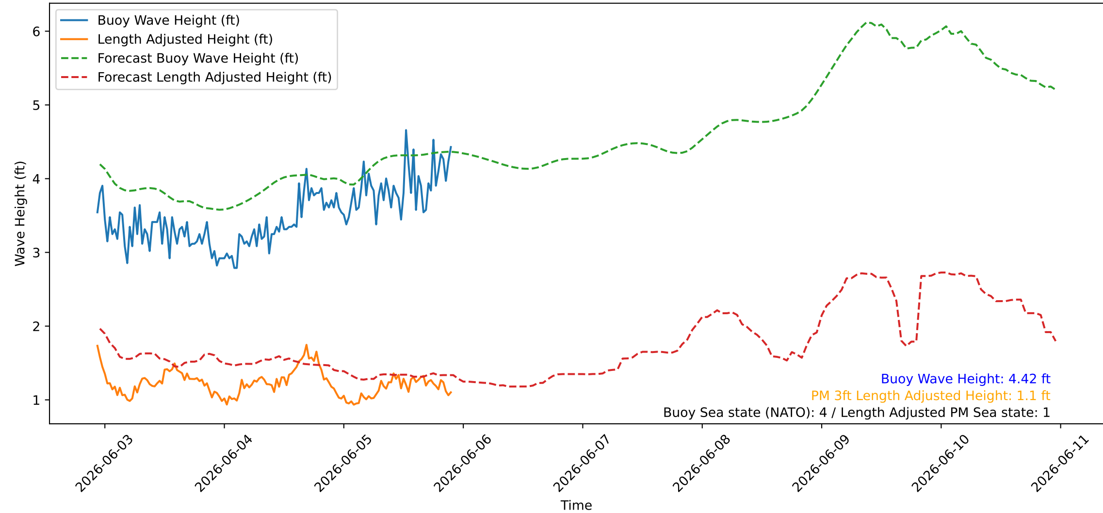
Wave Heights over Time for Green Beach at 2026-06-05 22:31:08
