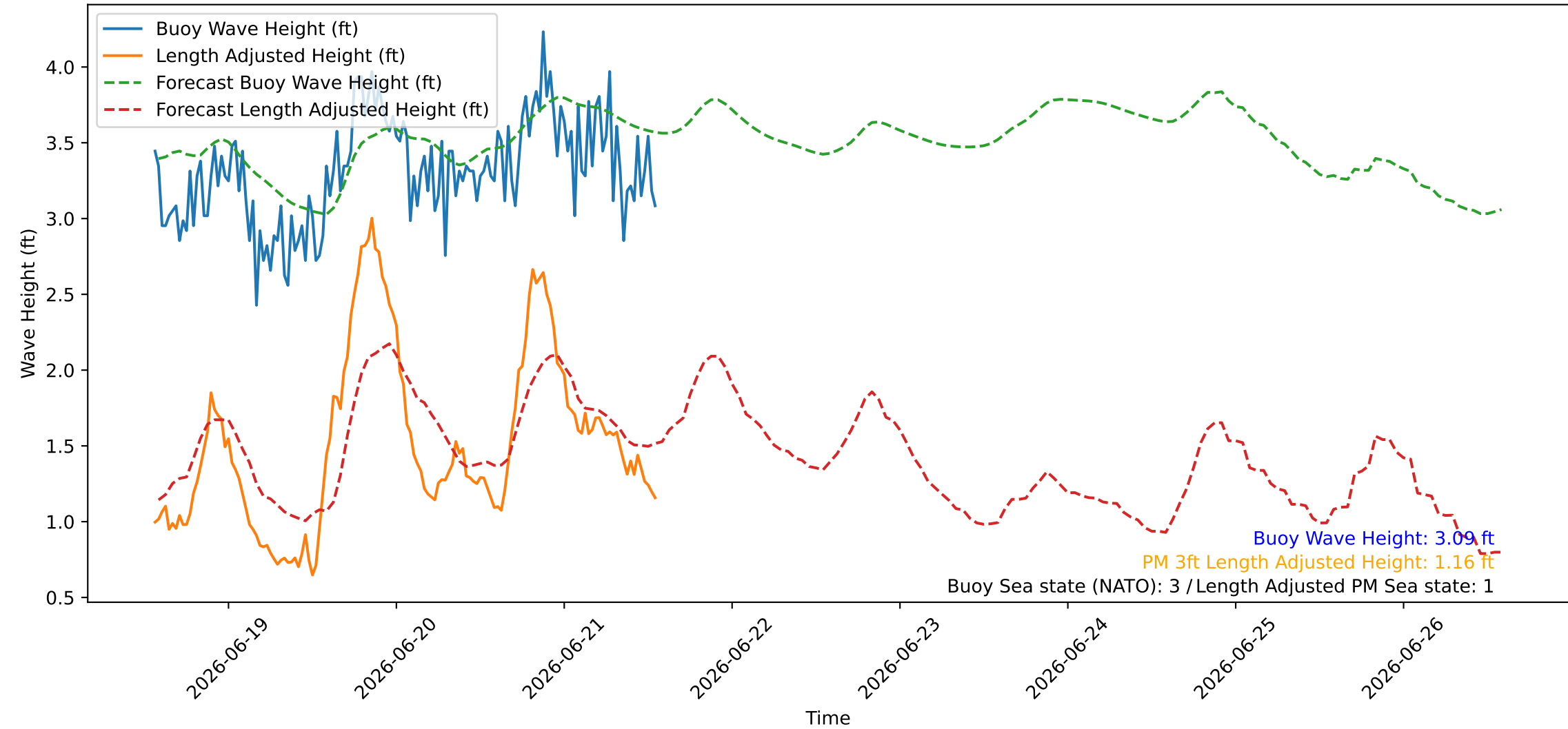
Wave Heights over Time for Green Beach at 2026-06-21 13:41:07
