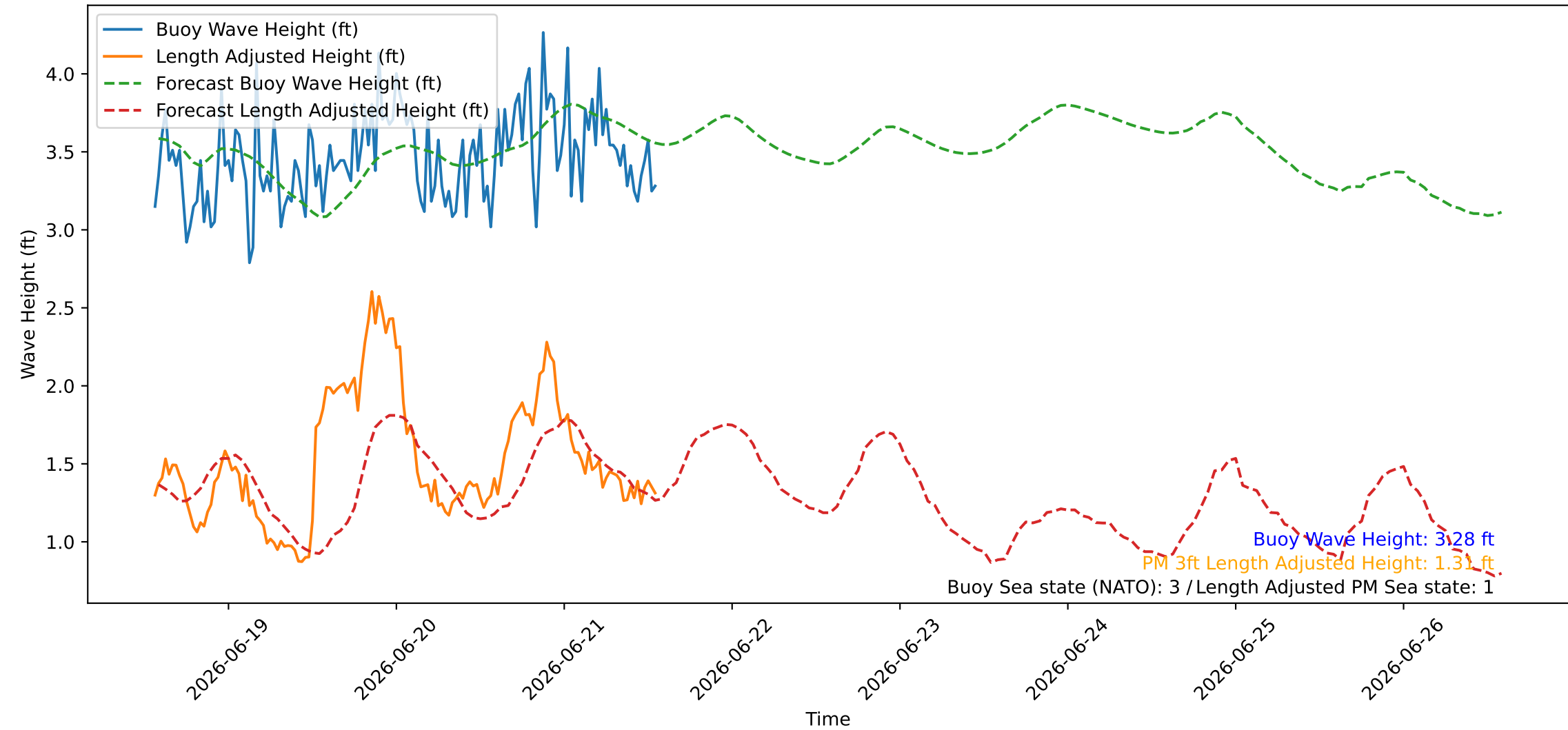
Wave Heights over Time for Oceanside Harbor at 2026-06-21 13:40:26
