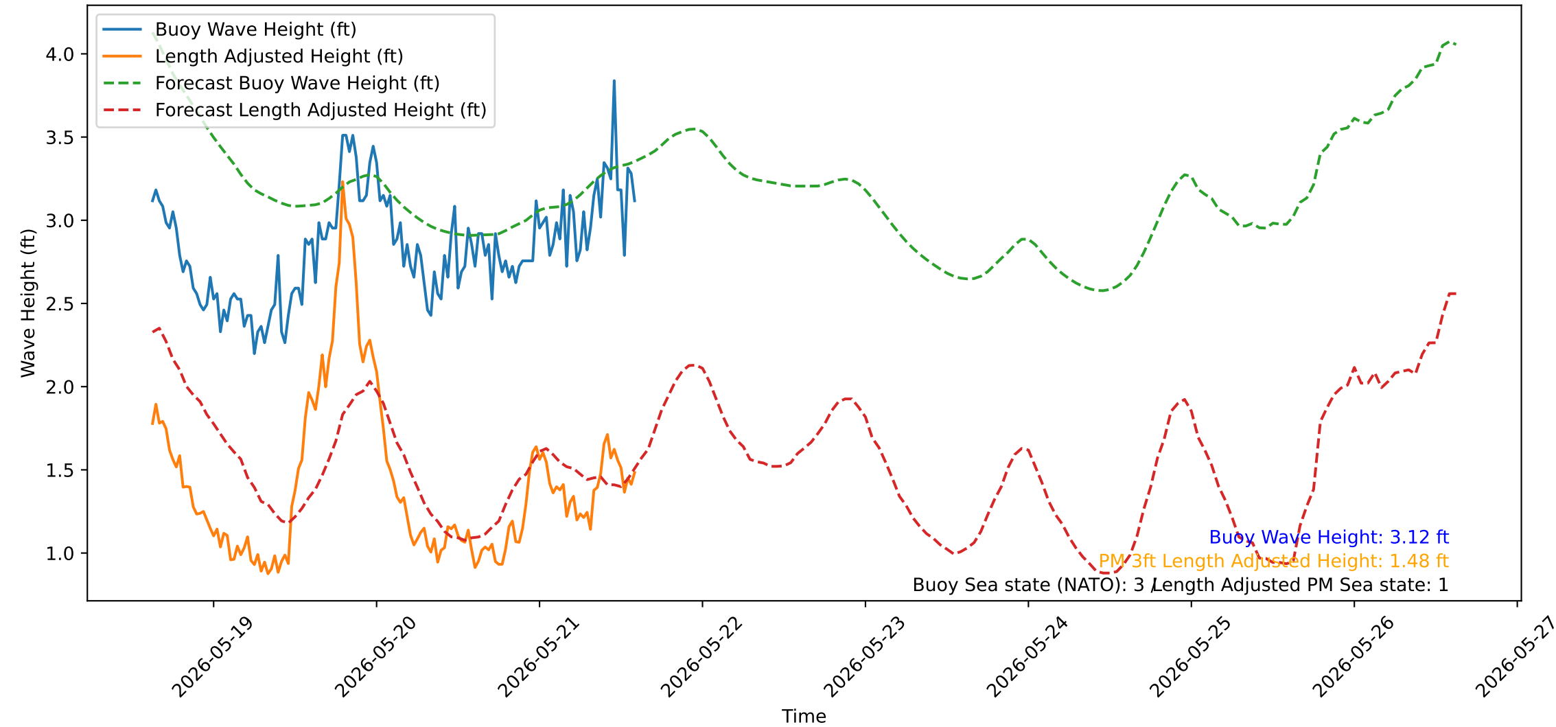
Wave Heights over Time for Oceanside Harbor at 2026-05-21 14:50:31
