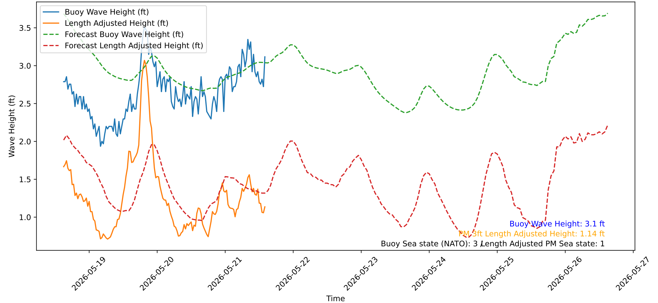
Wave Heights over Time for Red Beach at 2026-05-21 14:50:52
