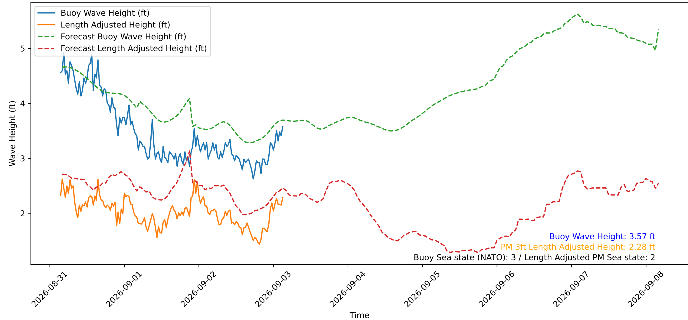
Wave Heights over Time for Oceanside Harbor at 2026-09-03 03:30:30
