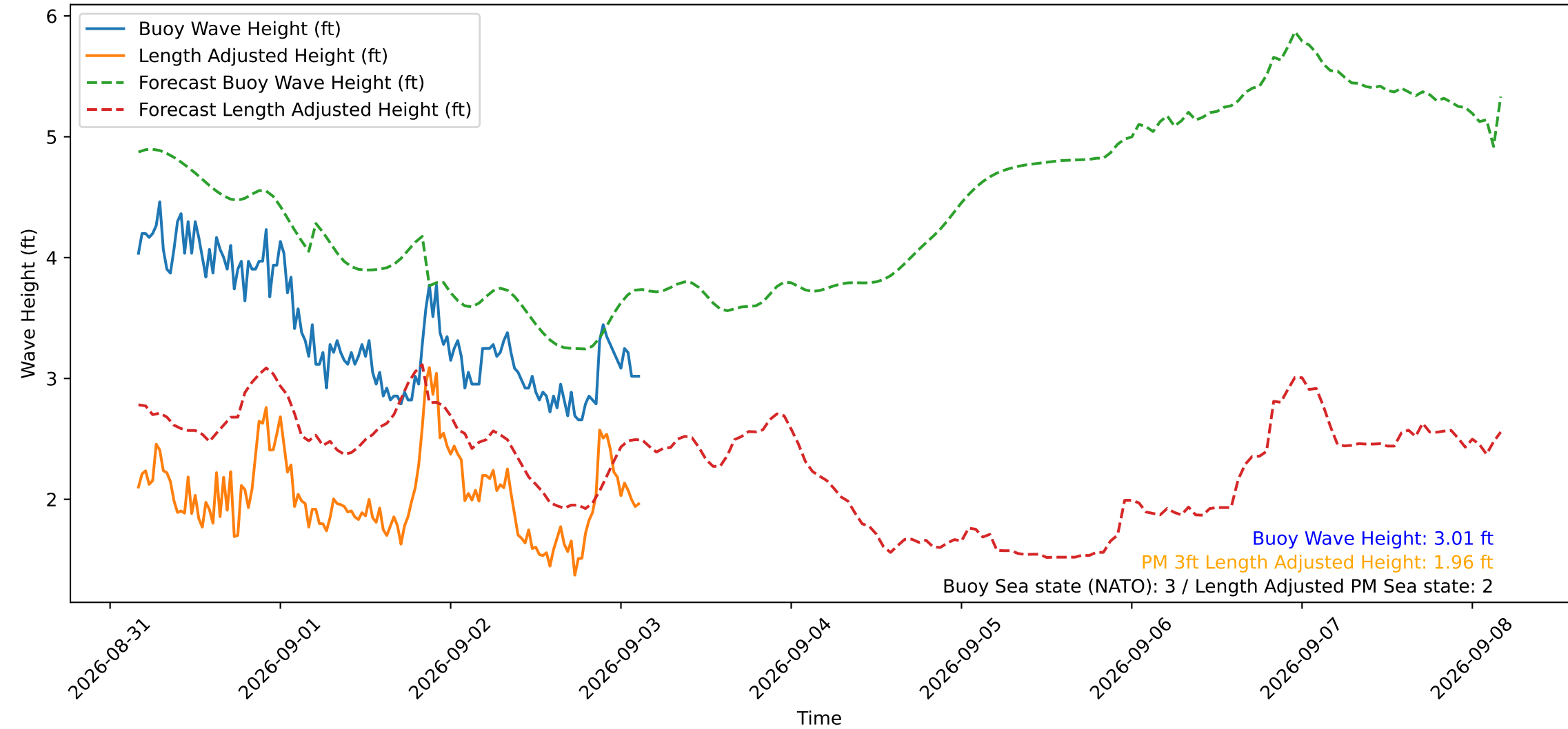
Wave Heights over Time for Green Beach at 2026-09-03 03:31:12
