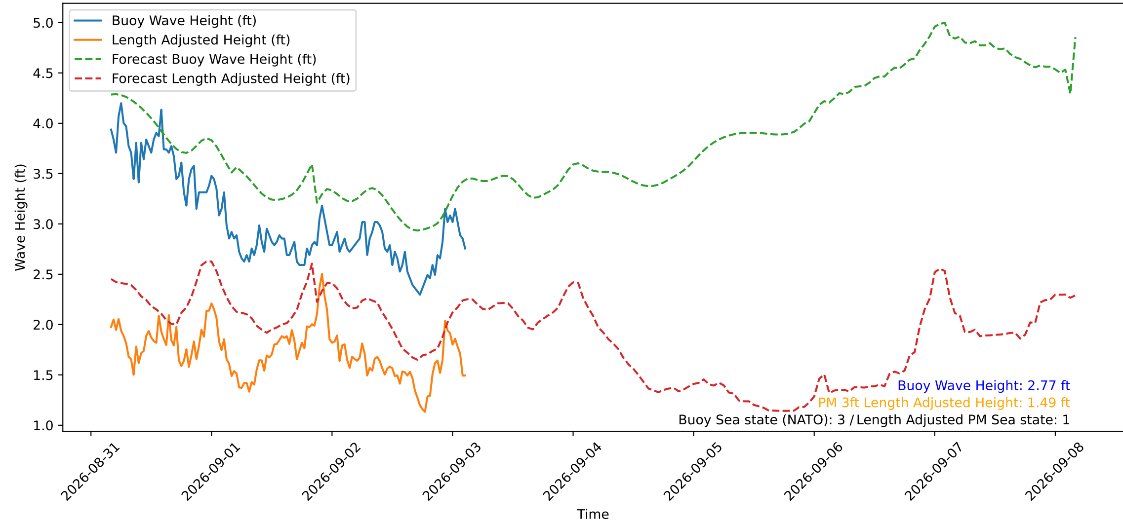
Wave Heights over Time for Red Beach at 2026-09-03 03:30:49
