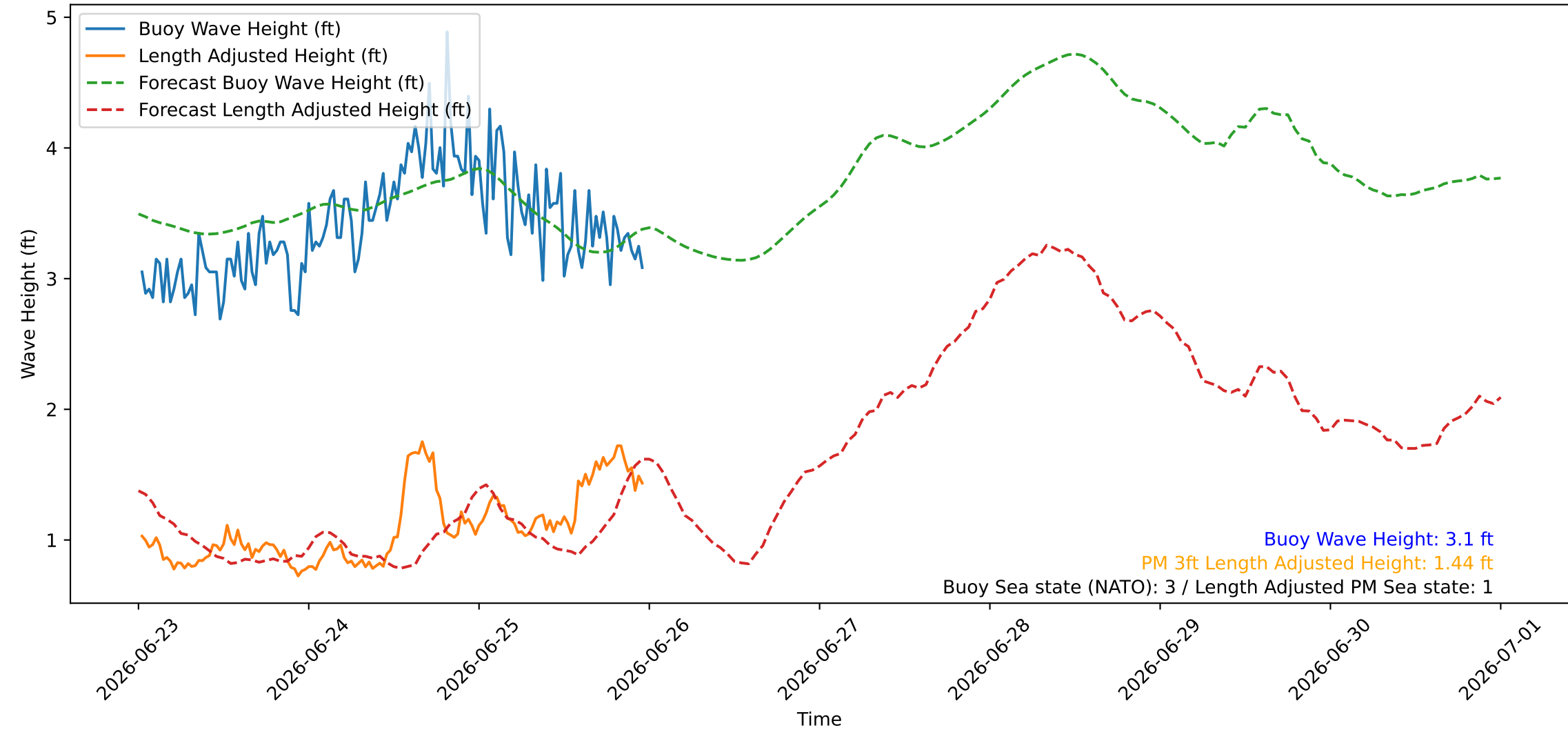
Wave Heights over Time for Oceanside Harbor at 2026-06-26 00:20:25
