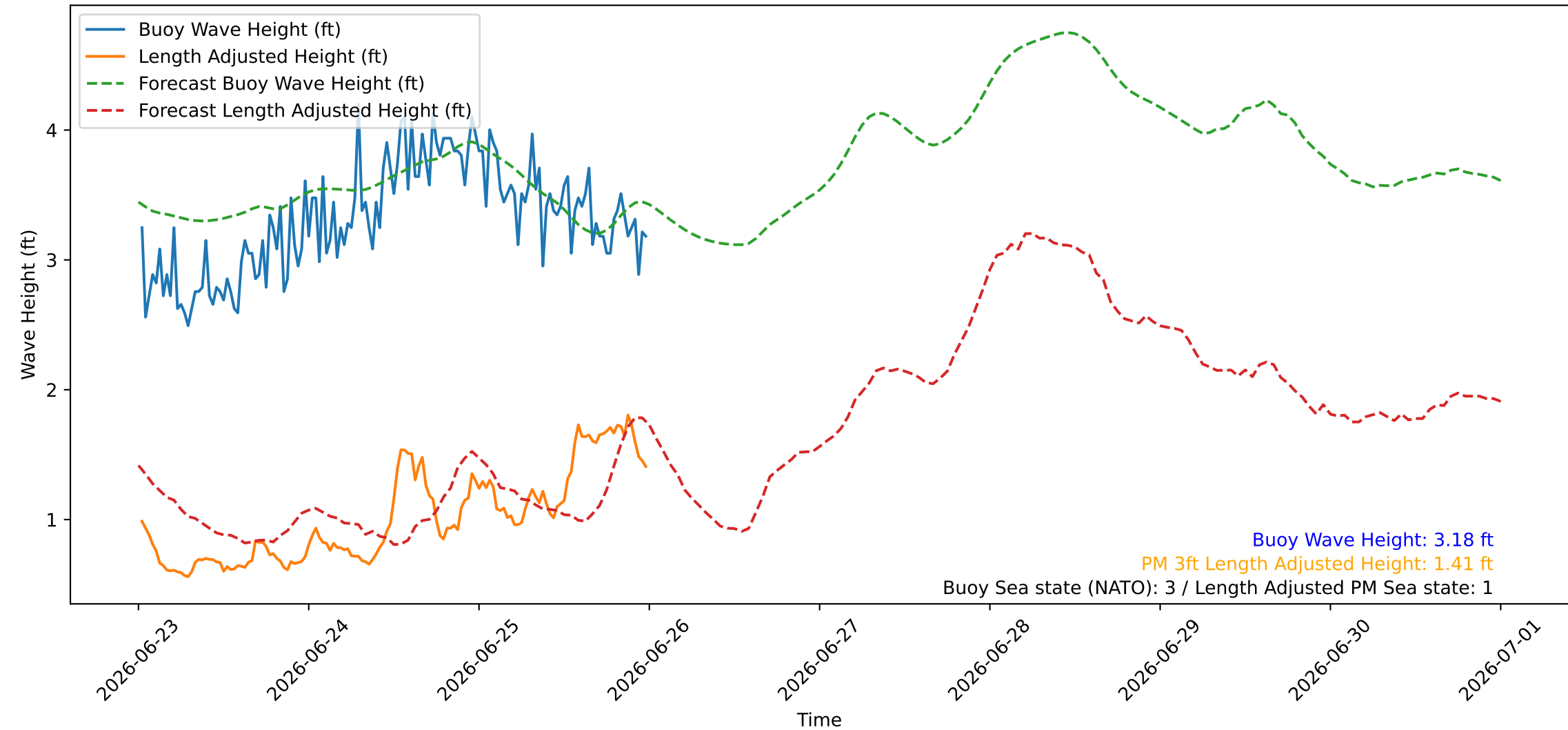
Wave Heights over Time for Green Beach at 2026-06-26 00:21:09
