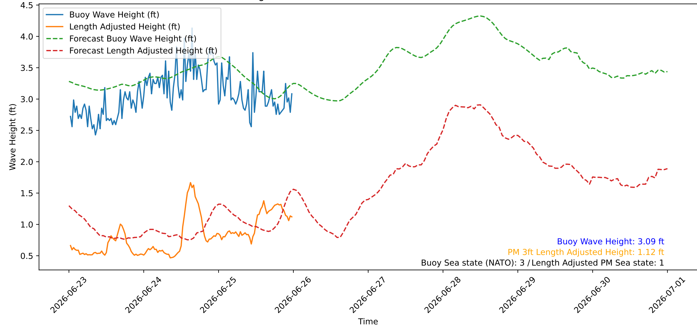
Wave Heights over Time for Red Beach at 2026-06-26 00:20:46
