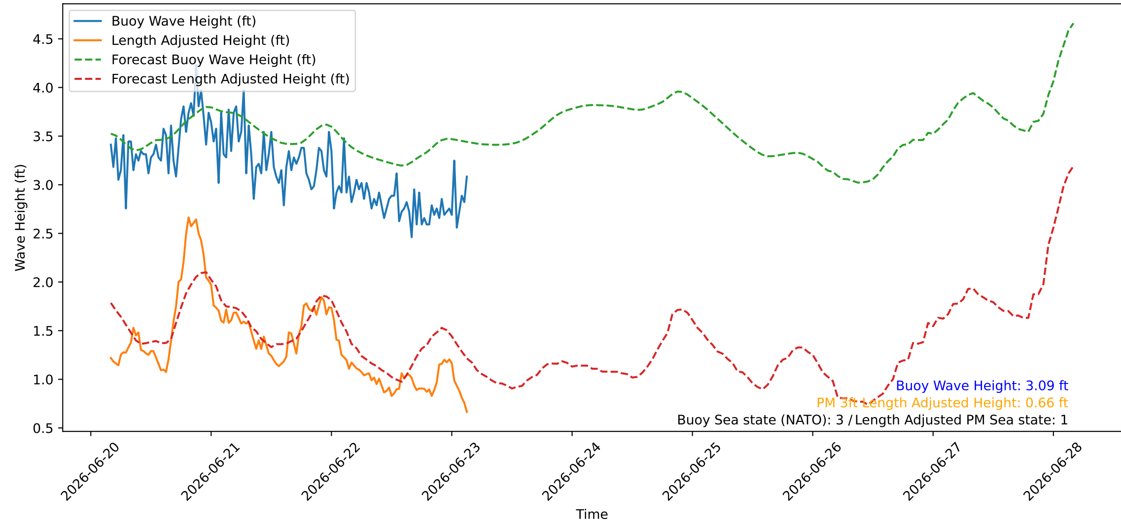
Wave Heights over Time for Green Beach at 2026-06-23 04:01:07
