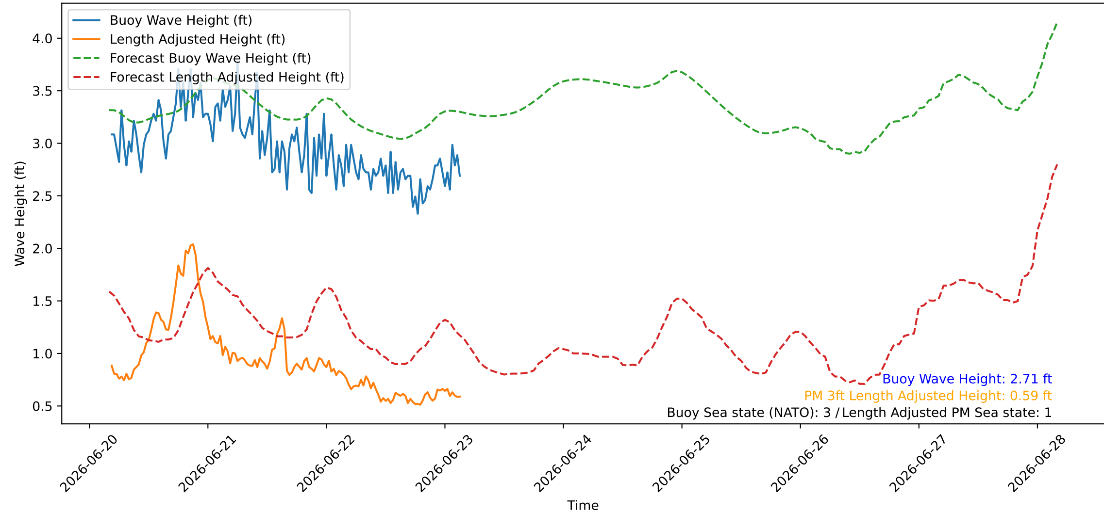
Wave Heights over Time for Red Beach at 2026-06-23 04:00:45
