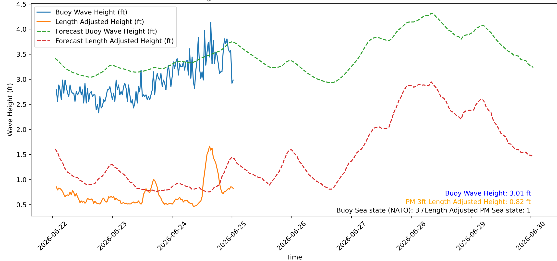
Wave Heights over Time for Red Beach at 2026-06-25 01:10:45
