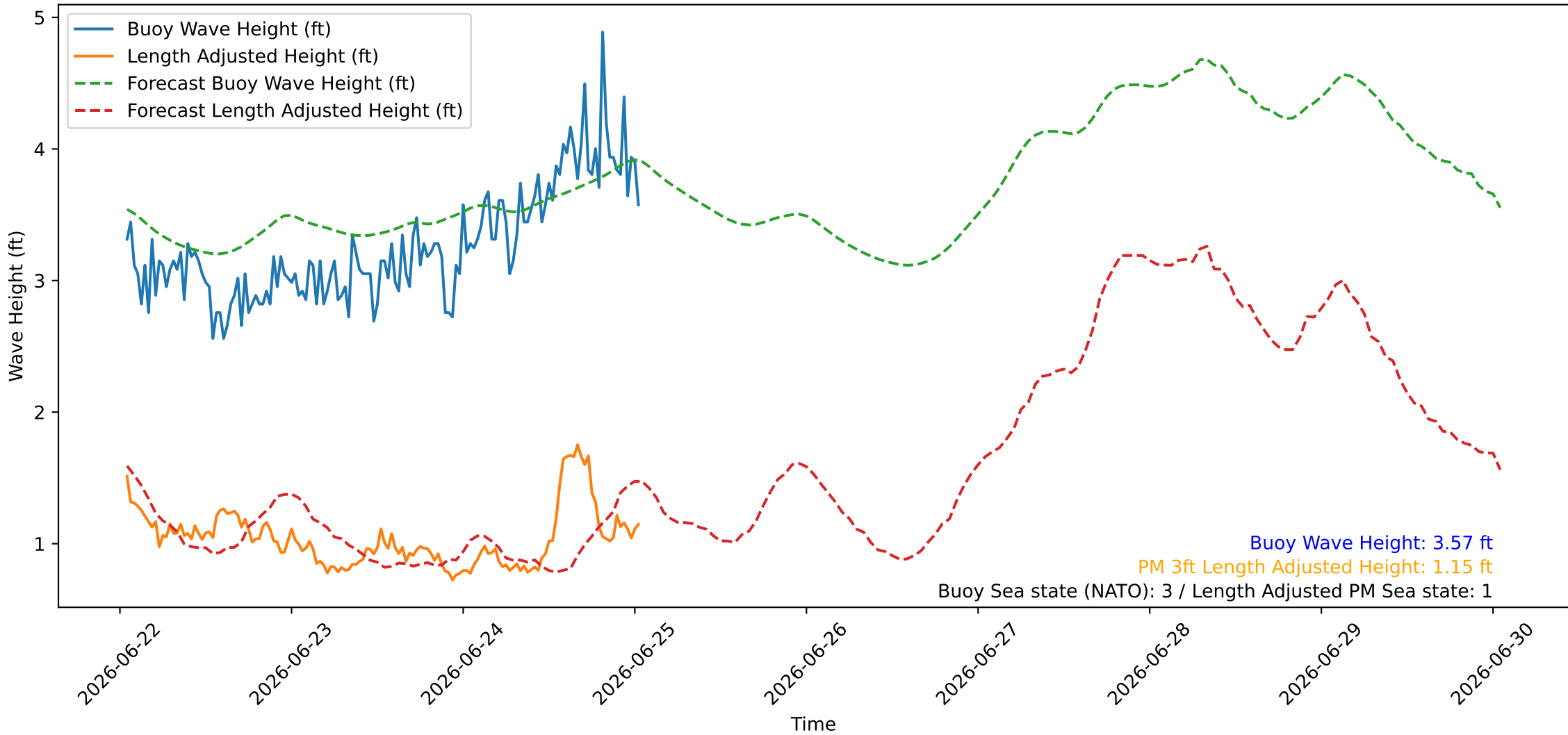
Wave Heights over Time for Oceanside Harbor at 2026-06-25 01:10:26
