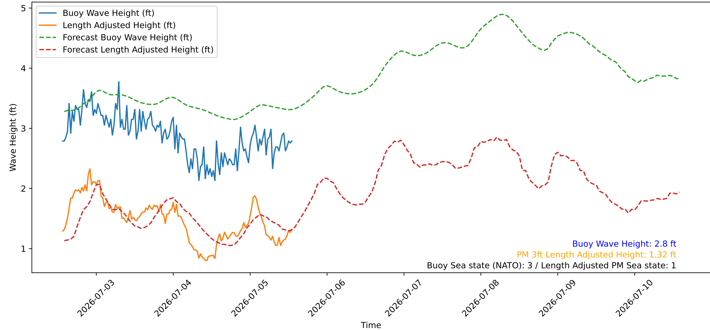
Wave Heights over Time for Oceanside Harbor at 2026-07-05 13:40:27
