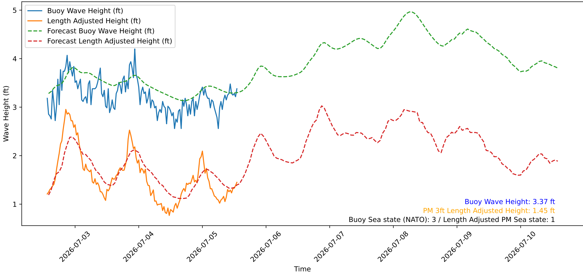
Wave Heights over Time for Green Beach at 2026-07-05 13:41:10
