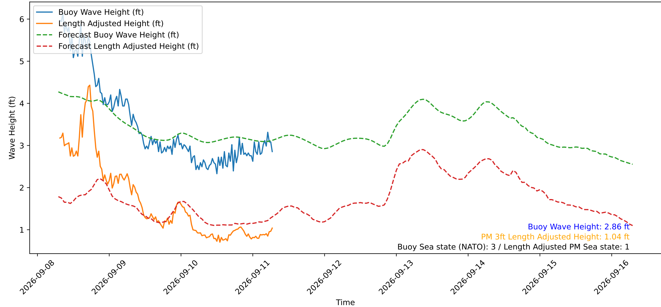
Wave Heights over Time for Red Beach at 2026-09-11 07:10:49
