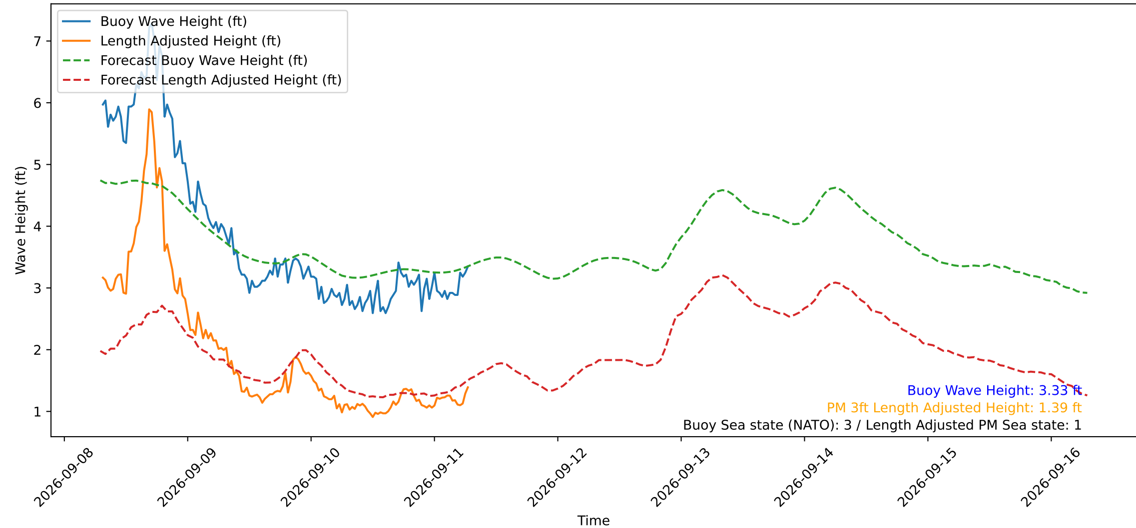
Wave Heights over Time for Green Beach at 2026-09-11 07:11:12
