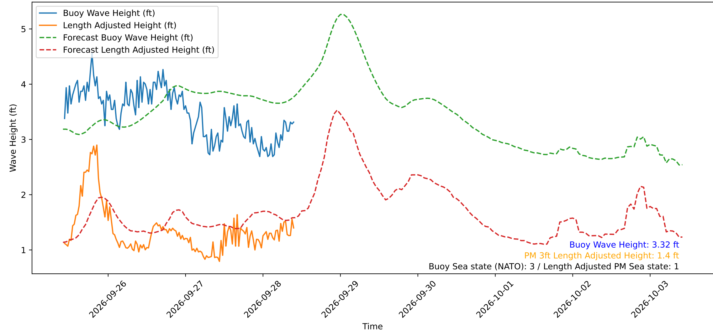
Wave Heights over Time for Green Beach at 2026-09-28 10:21:15
