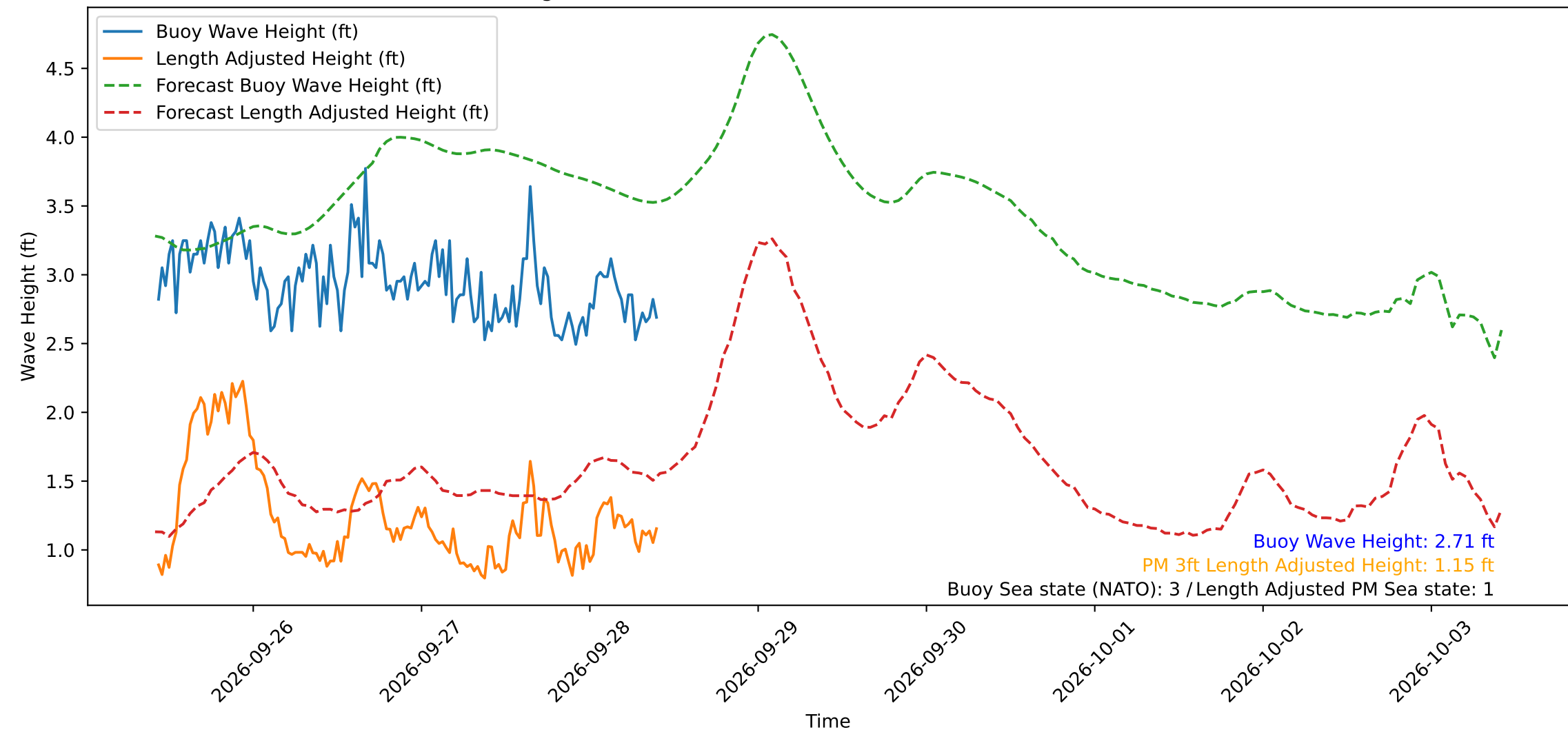
Wave Heights over Time for Oceanside Harbor at 2026-09-28 10:20:30
