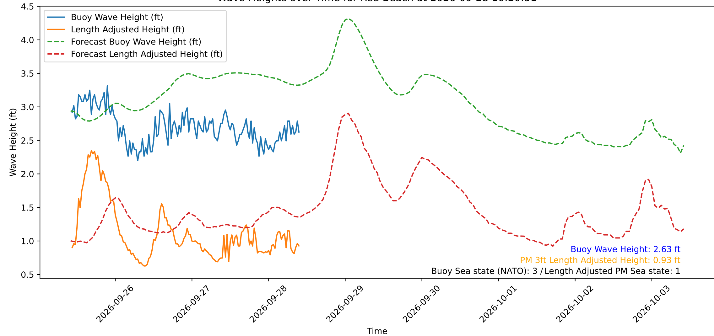
Wave Heights over Time for Red Beach at 2026-09-28 10:20:51
