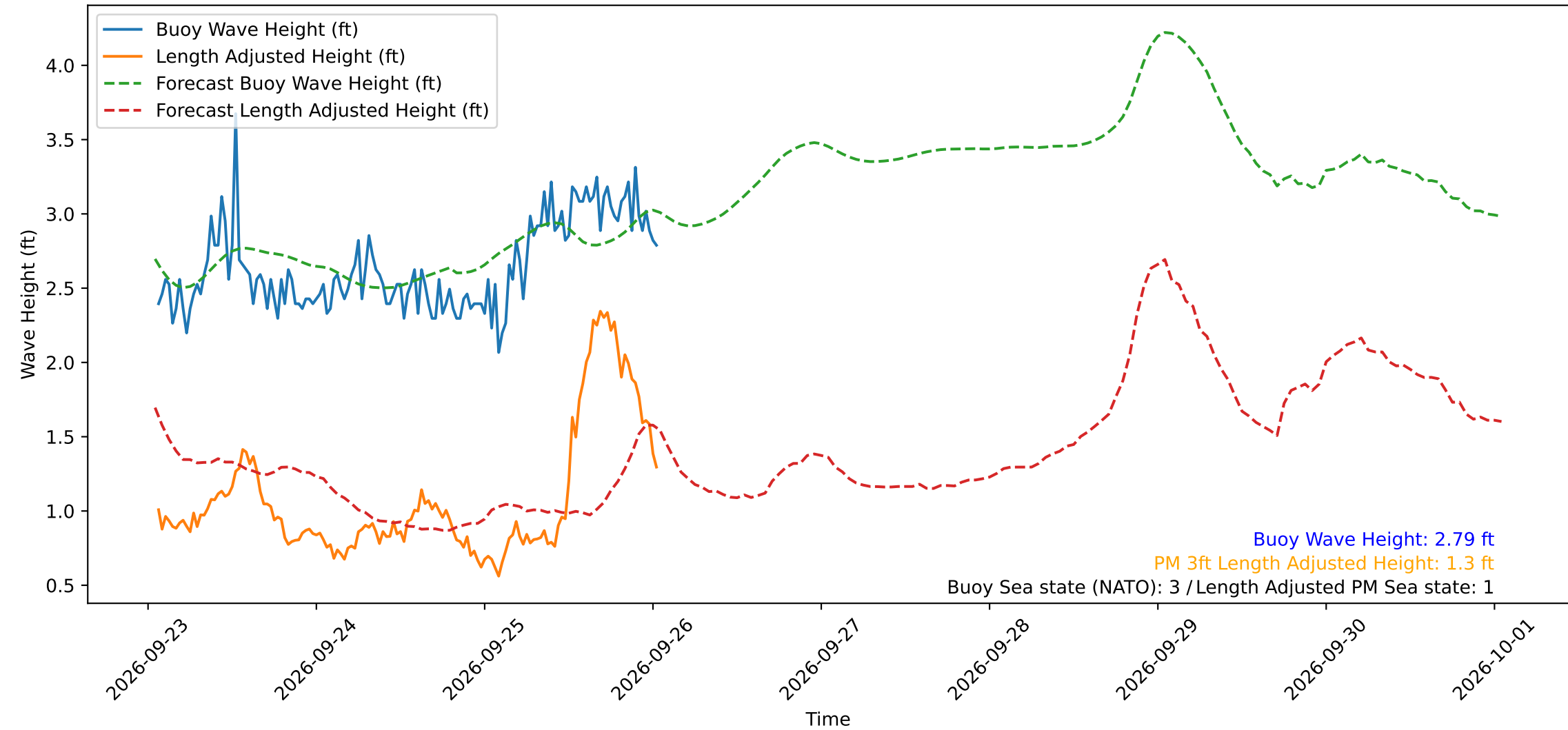
Wave Heights over Time for Red Beach at 2026-09-26 01:10:50
