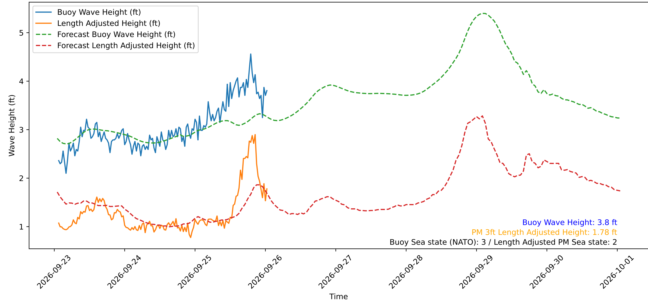
Wave Heights over Time for Green Beach at 2026-09-26 01:11:12
