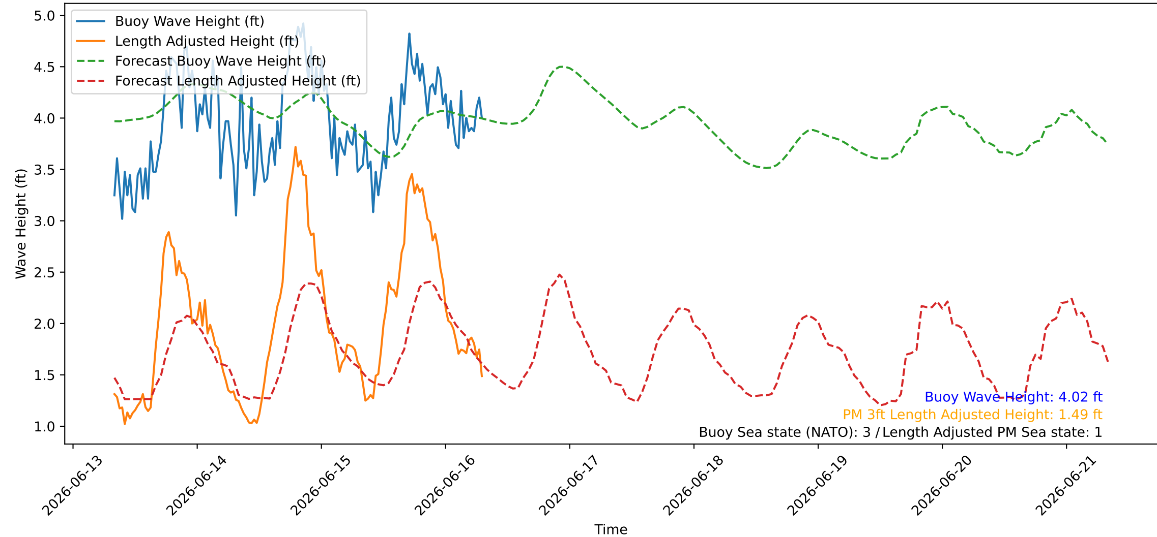
Wave Heights over Time for Green Beach at 2026-06-16 08:01:08
