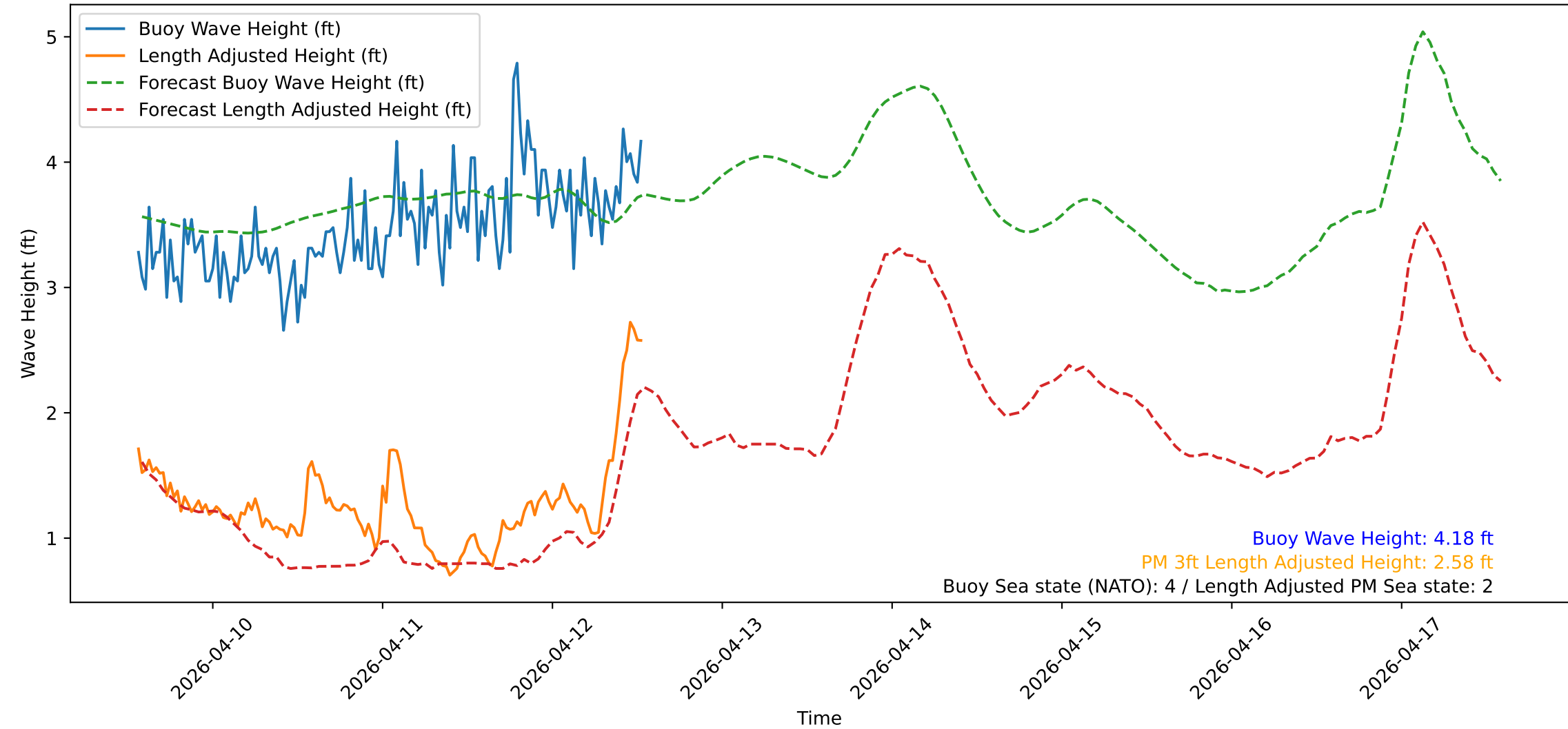
Wave Heights over Time for Oceanside Harbor at 2026-04-12 13:30:31
