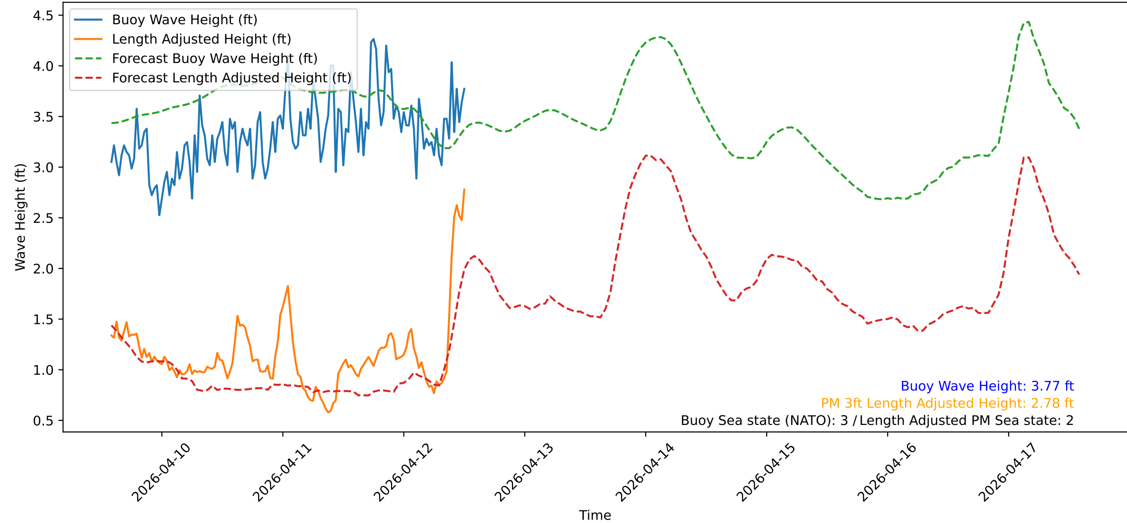
Wave Heights over Time for Red Beach at 2026-04-12 13:30:50
