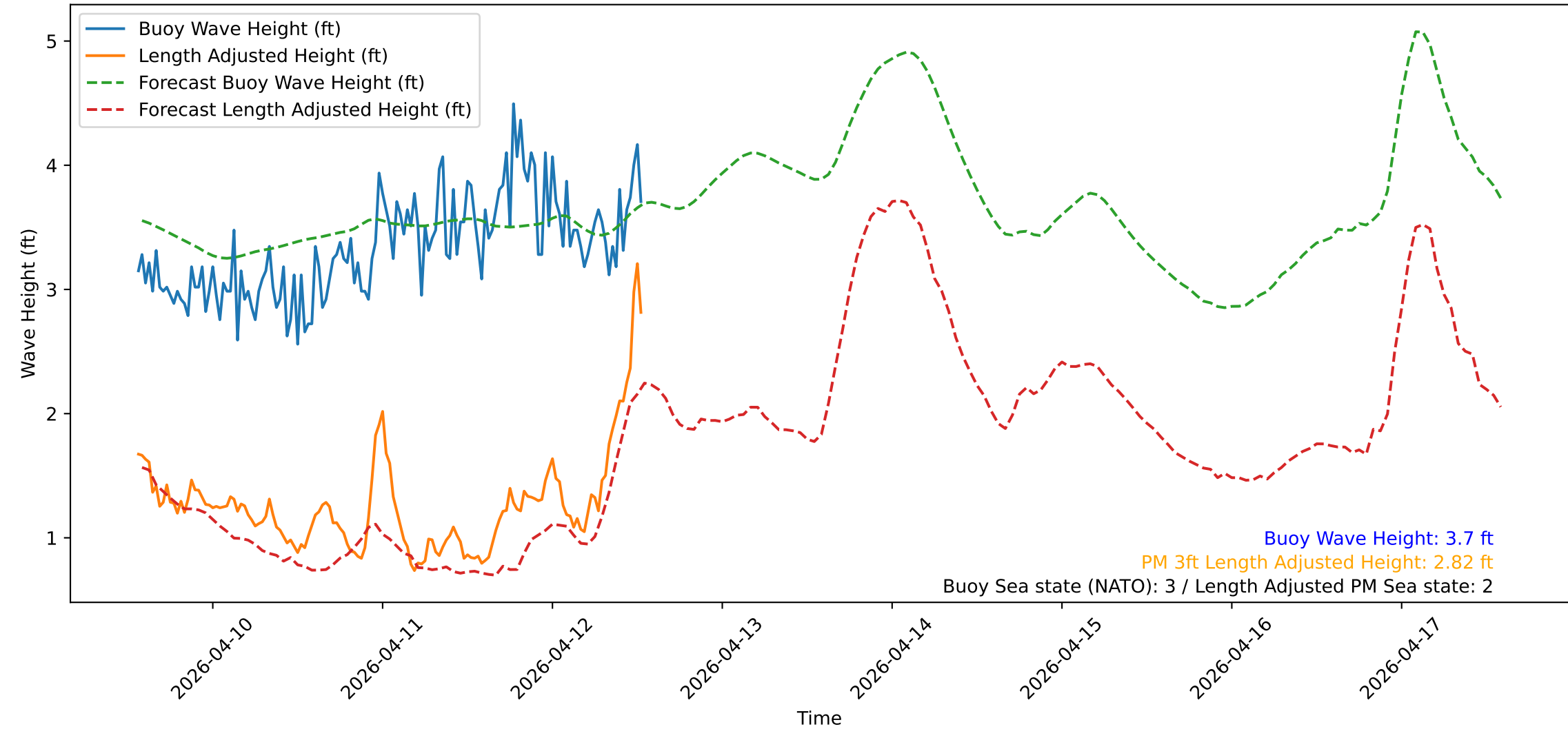
Wave Heights over Time for Green Beach at 2026-04-12 13:31:13
