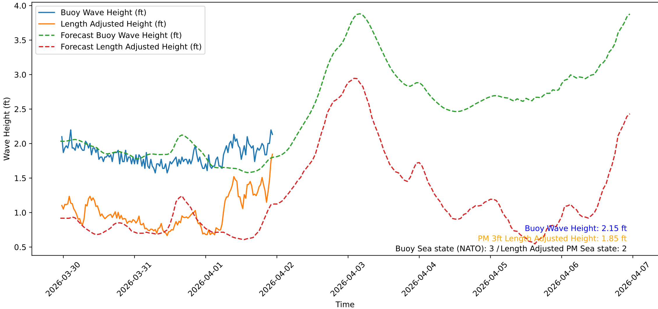
Wave Heights over Time for Oceanside Harbor at 2026-04-01 23:20:31
