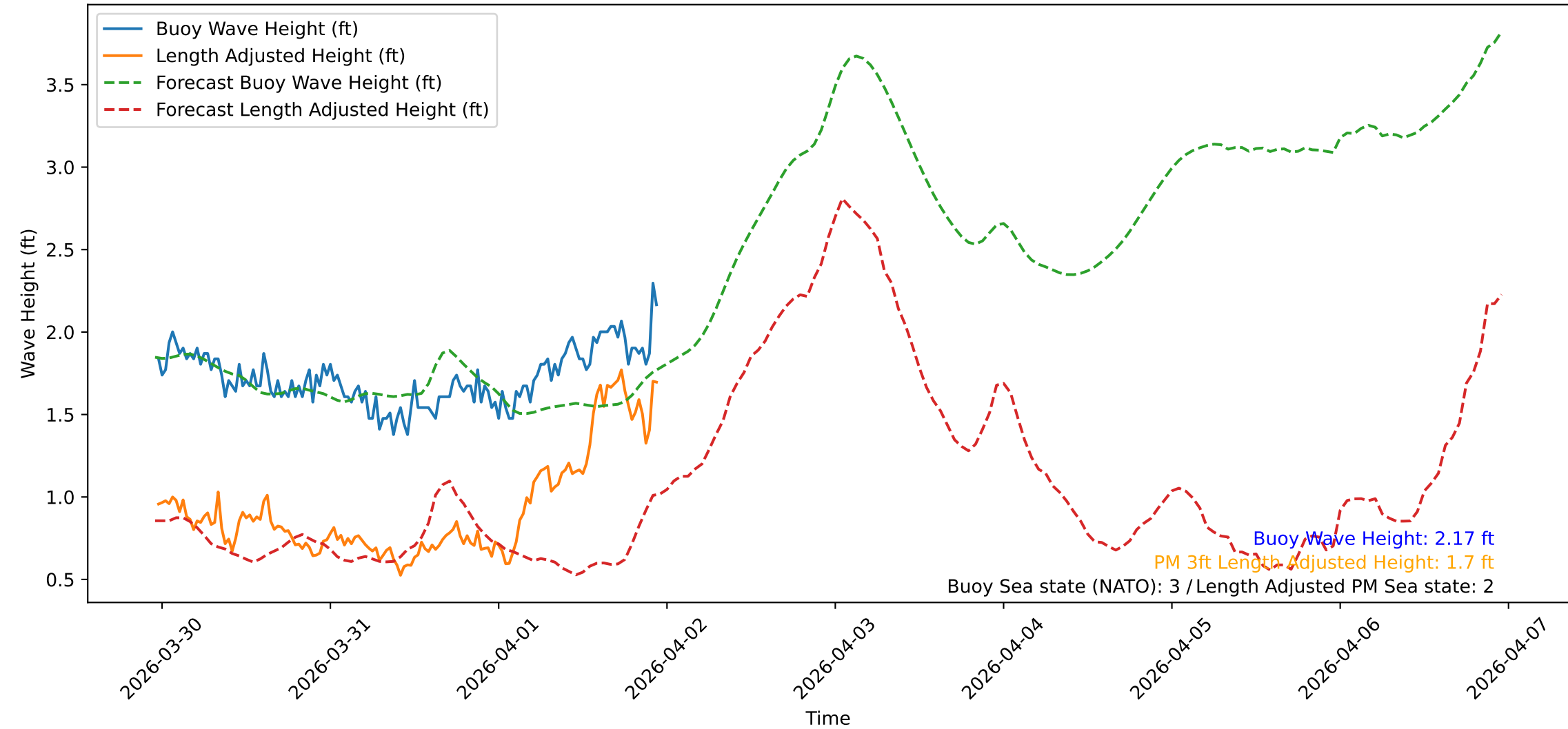
Wave Heights over Time for Red Beach at 2026-04-01 23:20:47
