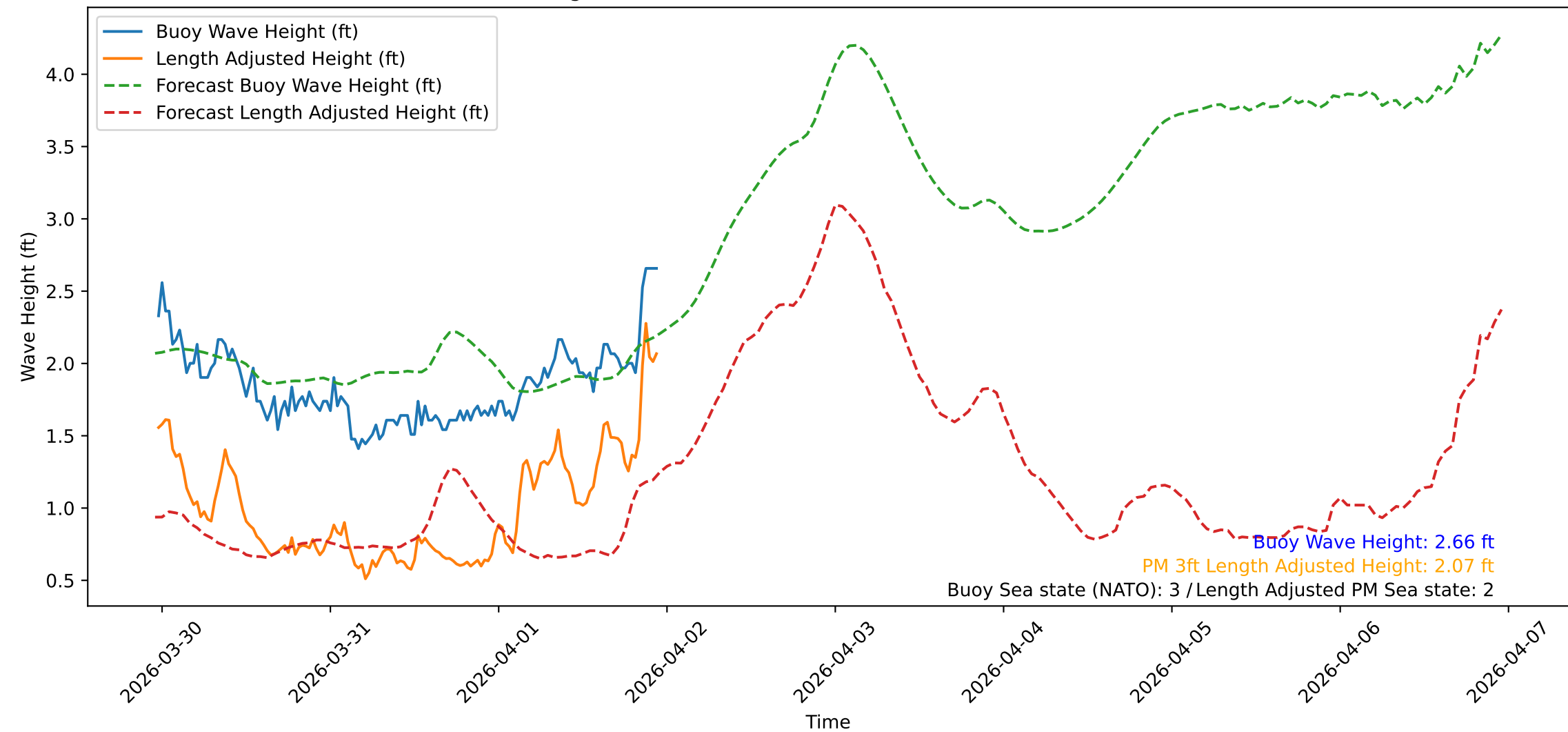
Wave Heights over Time for Green Beach at 2026-04-01 23:21:10
