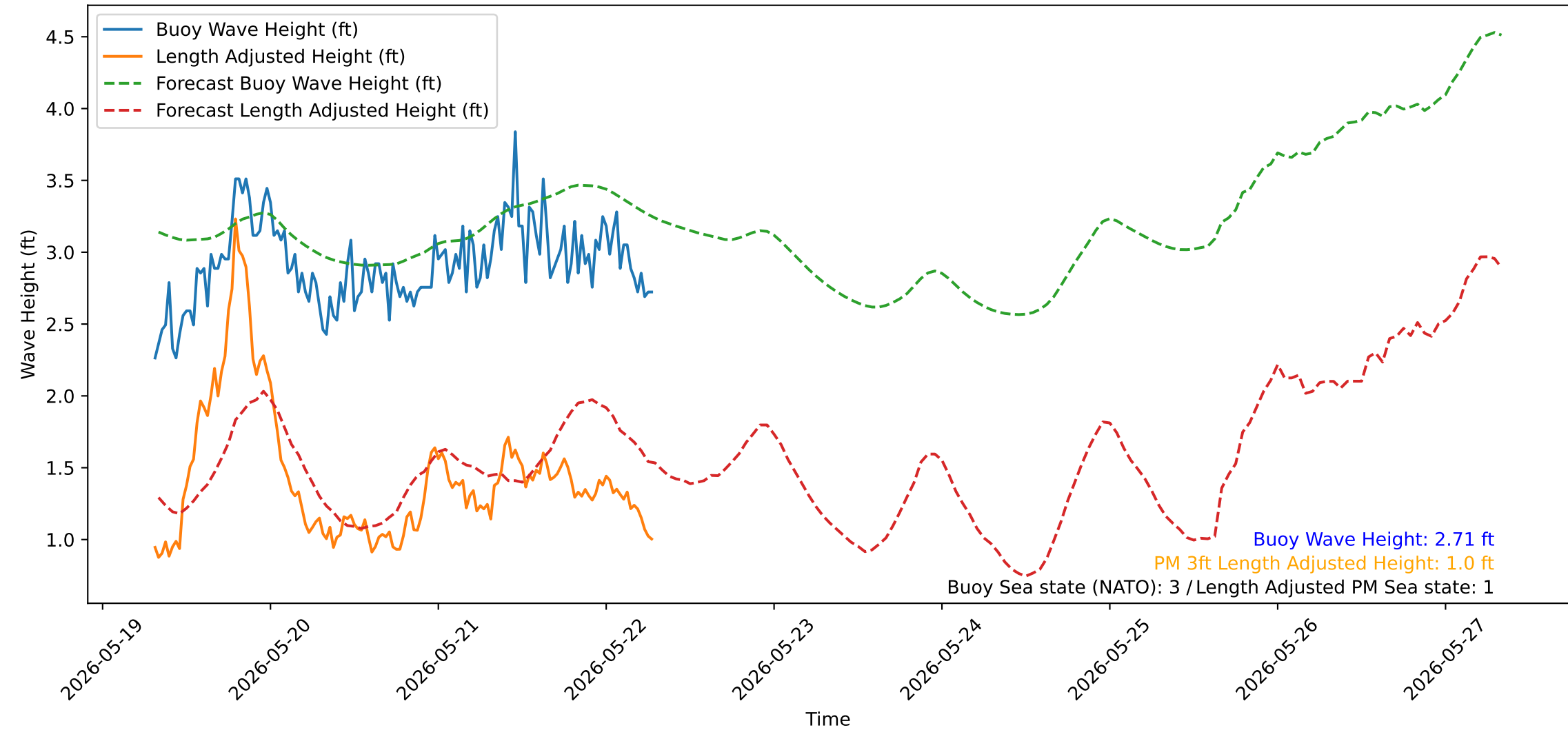
Wave Heights over Time for Oceanside Harbor at 2026-05-22 07:30:32
