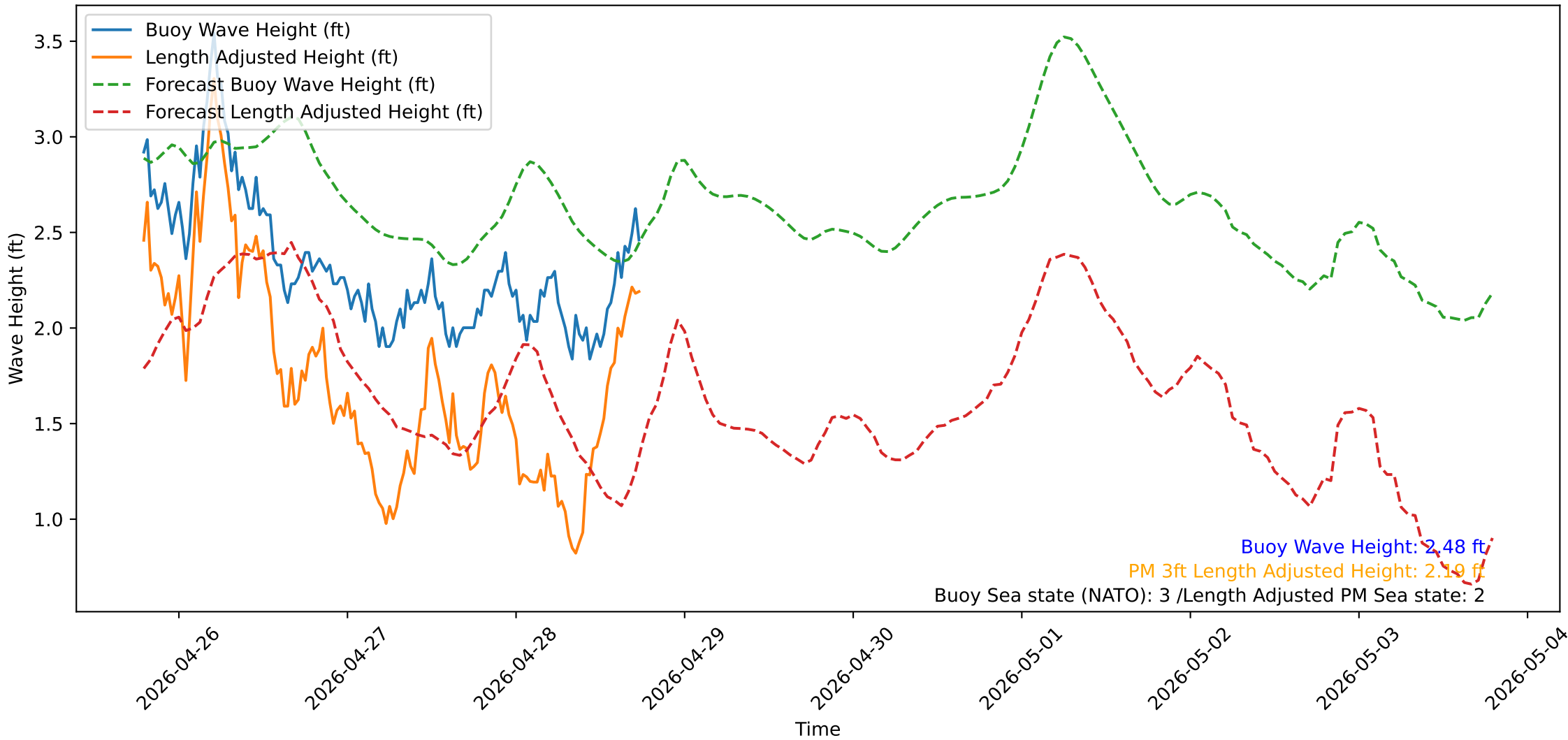
Wave Heights over Time for Red Beach at 2026-04-28 18:40:50
