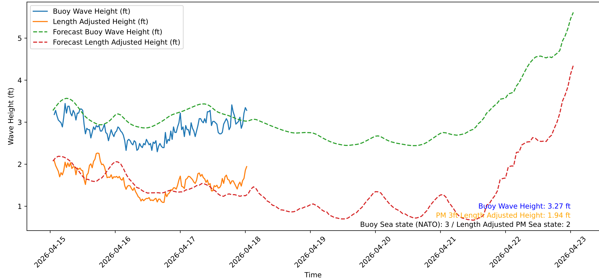
Wave Heights over Time for Oceanside Harbor at 2026-04-18 01:20:31
