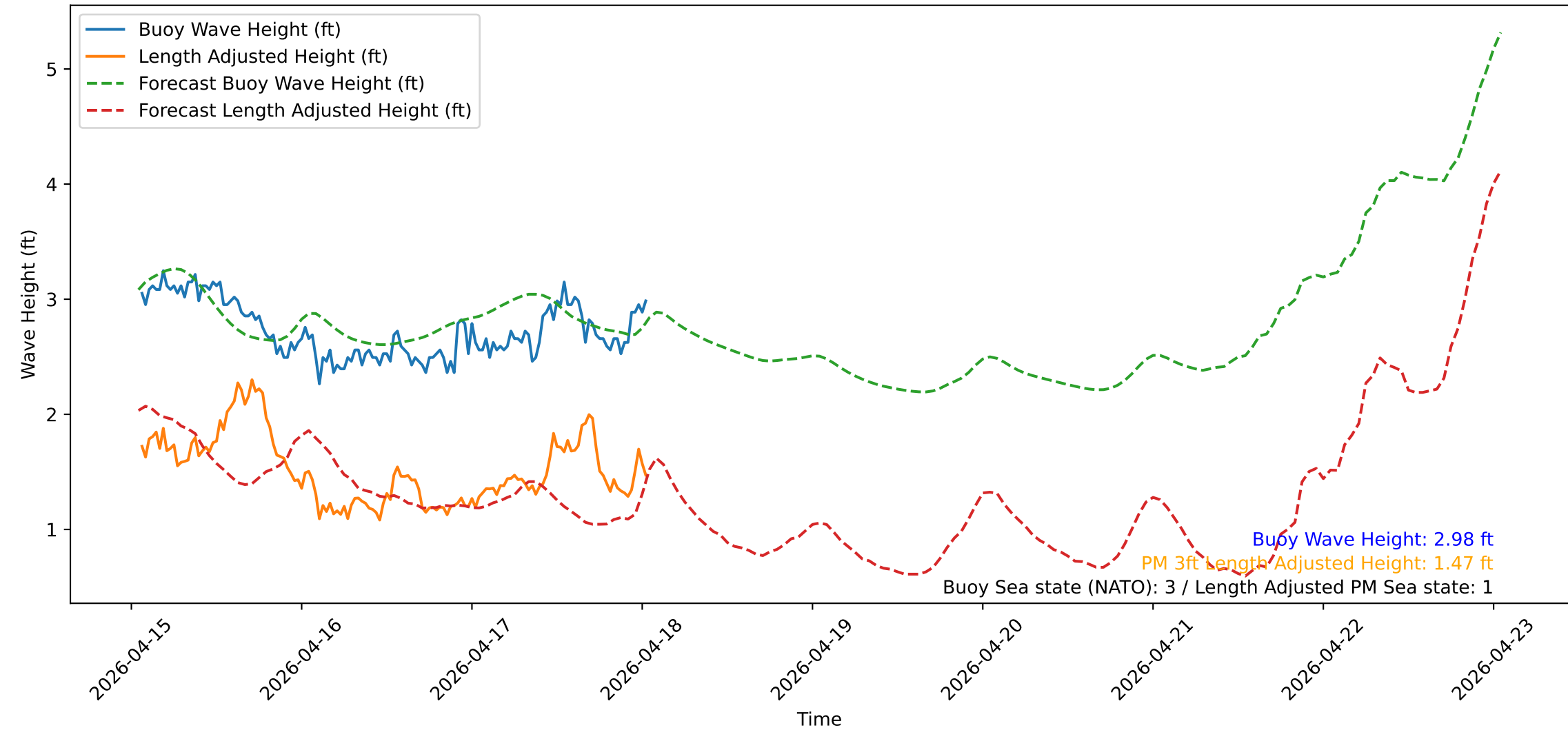
Wave Heights over Time for Red Beach at 2026-04-18 01:20:51
