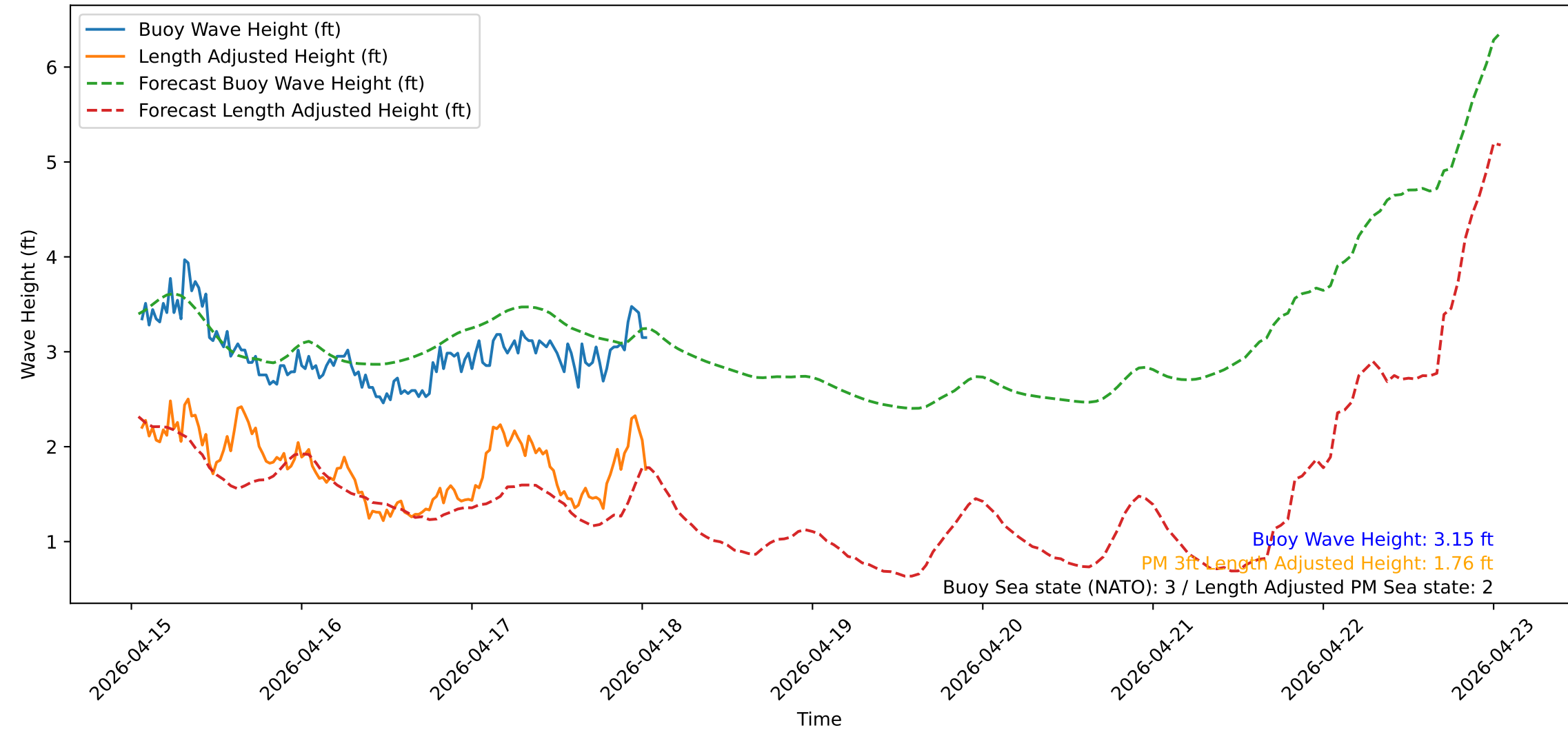
Wave Heights over Time for Green Beach at 2026-04-18 01:21:13
