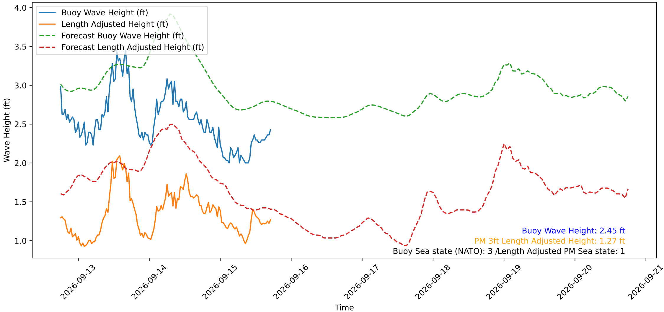
Wave Heights over Time for Red Beach at 2026-09-15 17:40:49
