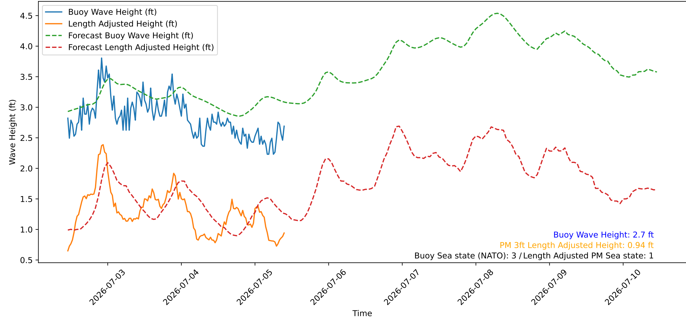
Wave Heights over Time for Red Beach at 2026-07-05 10:30:50
