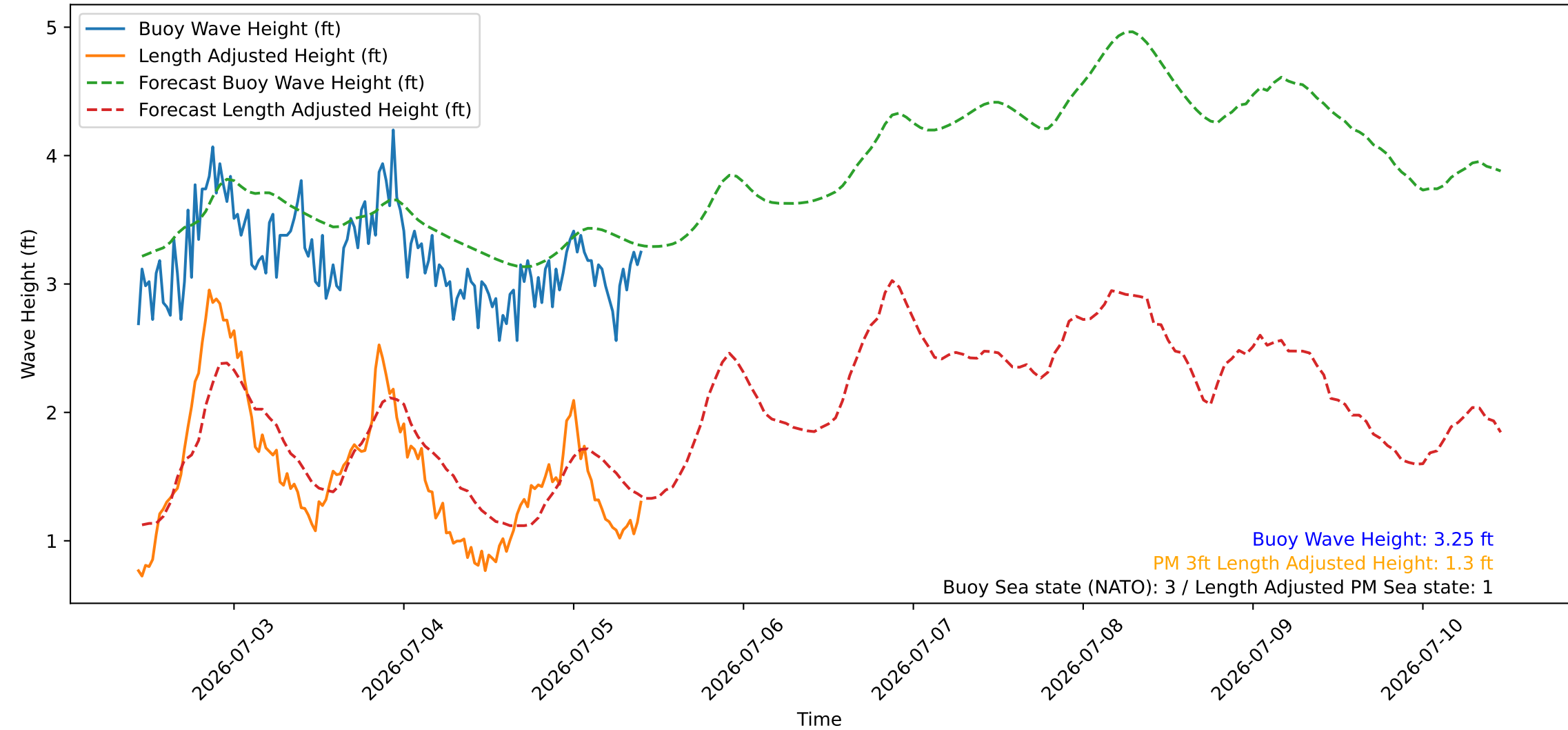
Wave Heights over Time for Green Beach at 2026-07-05 10:31:14
