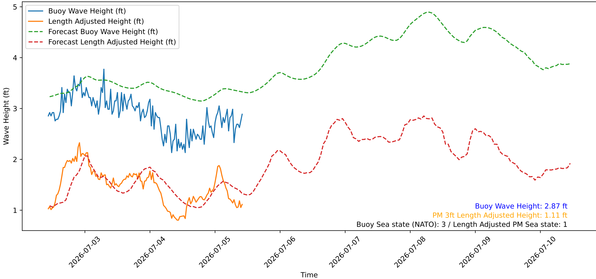
Wave Heights over Time for Oceanside Harbor at 2026-07-05 10:30:28
