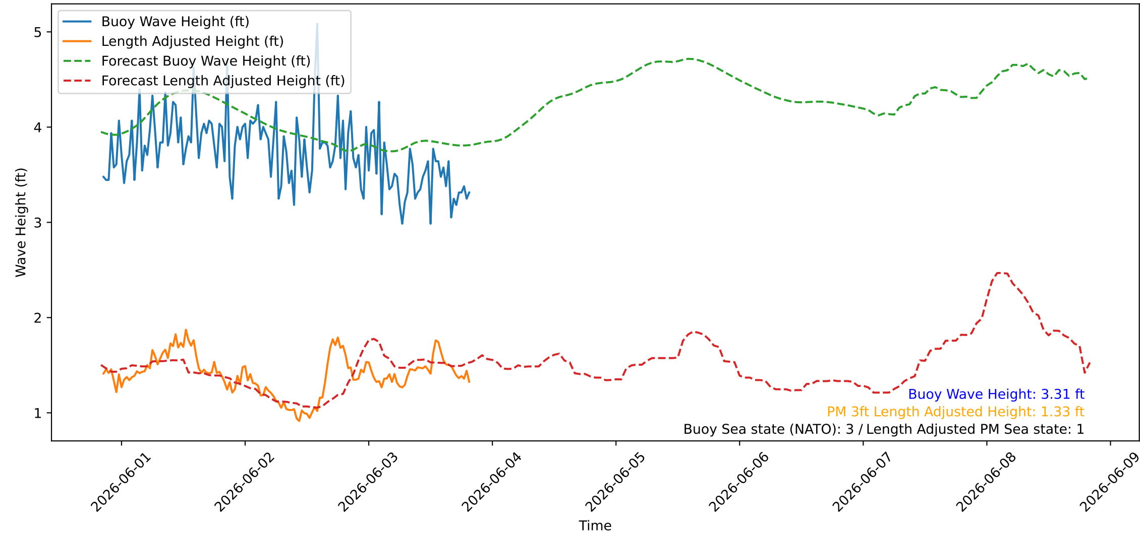
Wave Heights over Time for Oceanside Harbor at 2026-06-03 20:20:26
