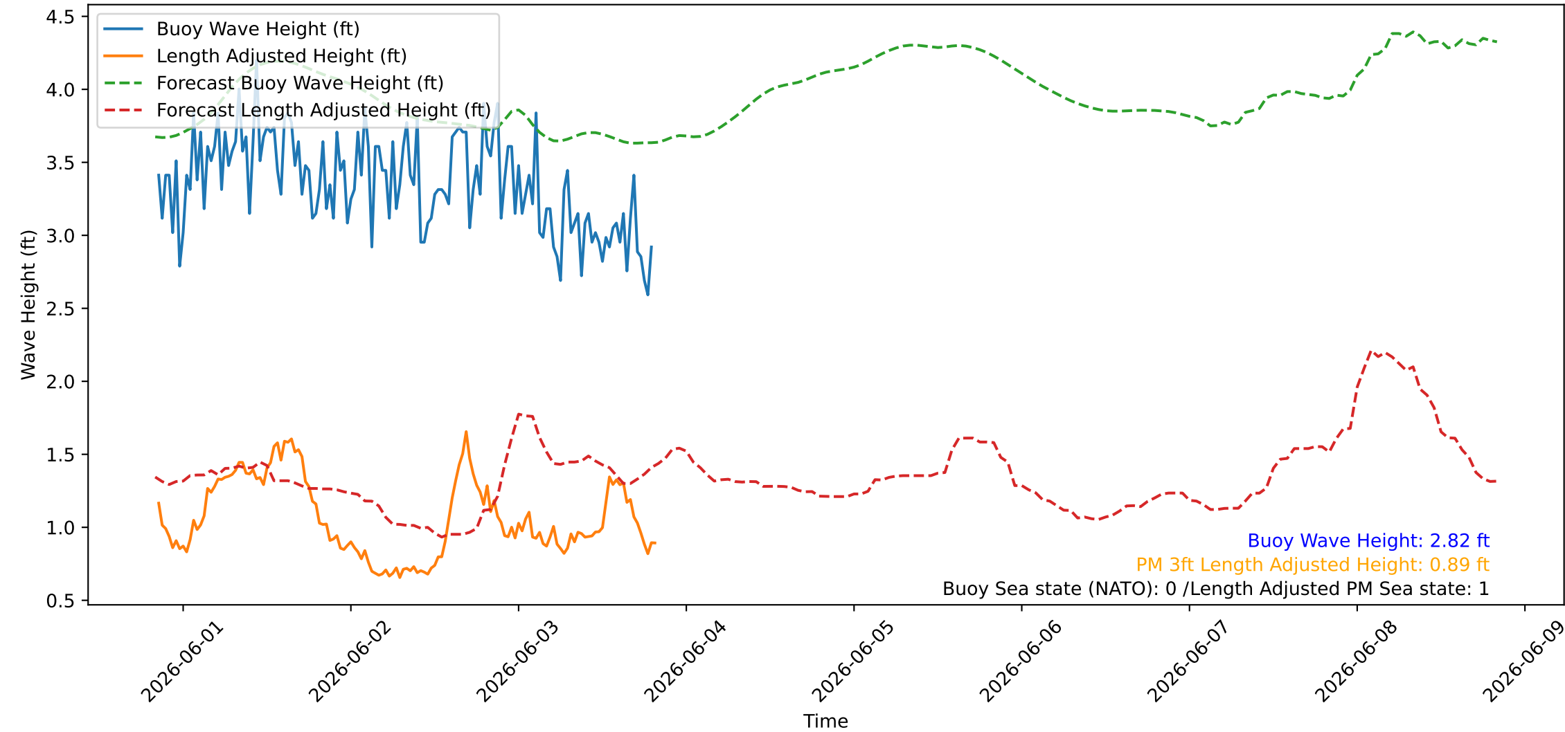
Wave Heights over Time for Red Beach at 2026-06-03 20:20:47
