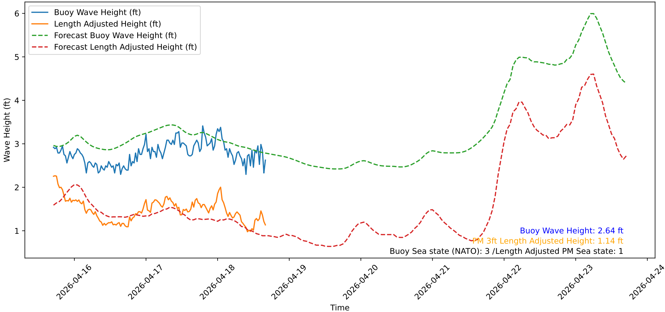
Wave Heights over Time for Oceanside Harbor at 2026-04-18 17:00:31
