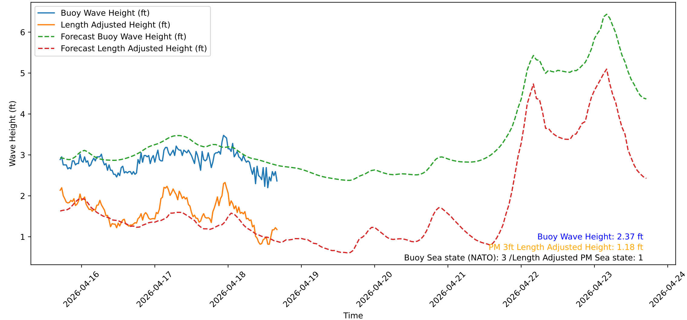
Wave Heights over Time for Green Beach at 2026-04-18 17:01:13
