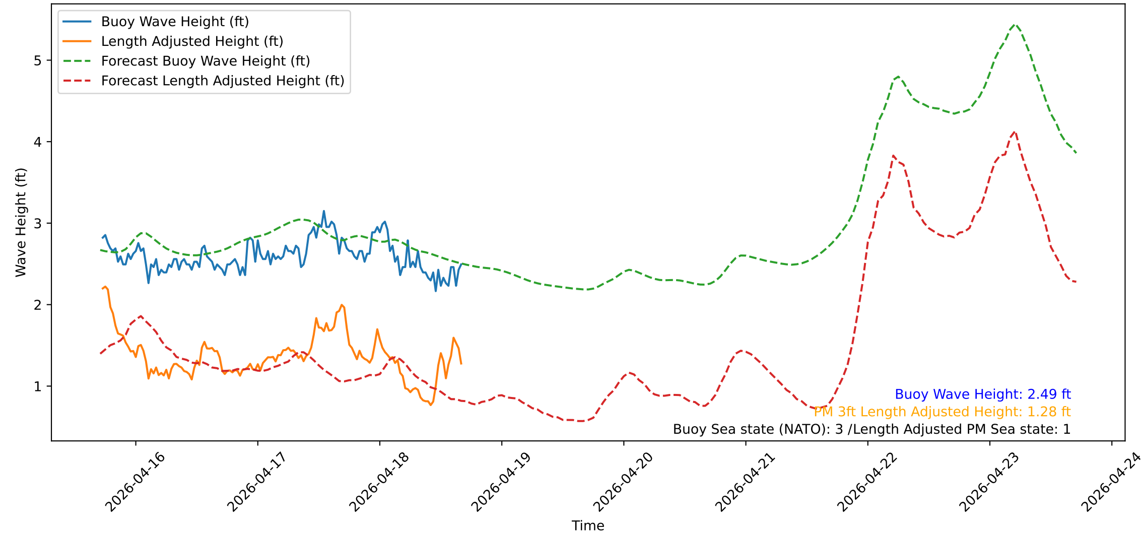
Wave Heights over Time for Red Beach at 2026-04-18 17:00:51
