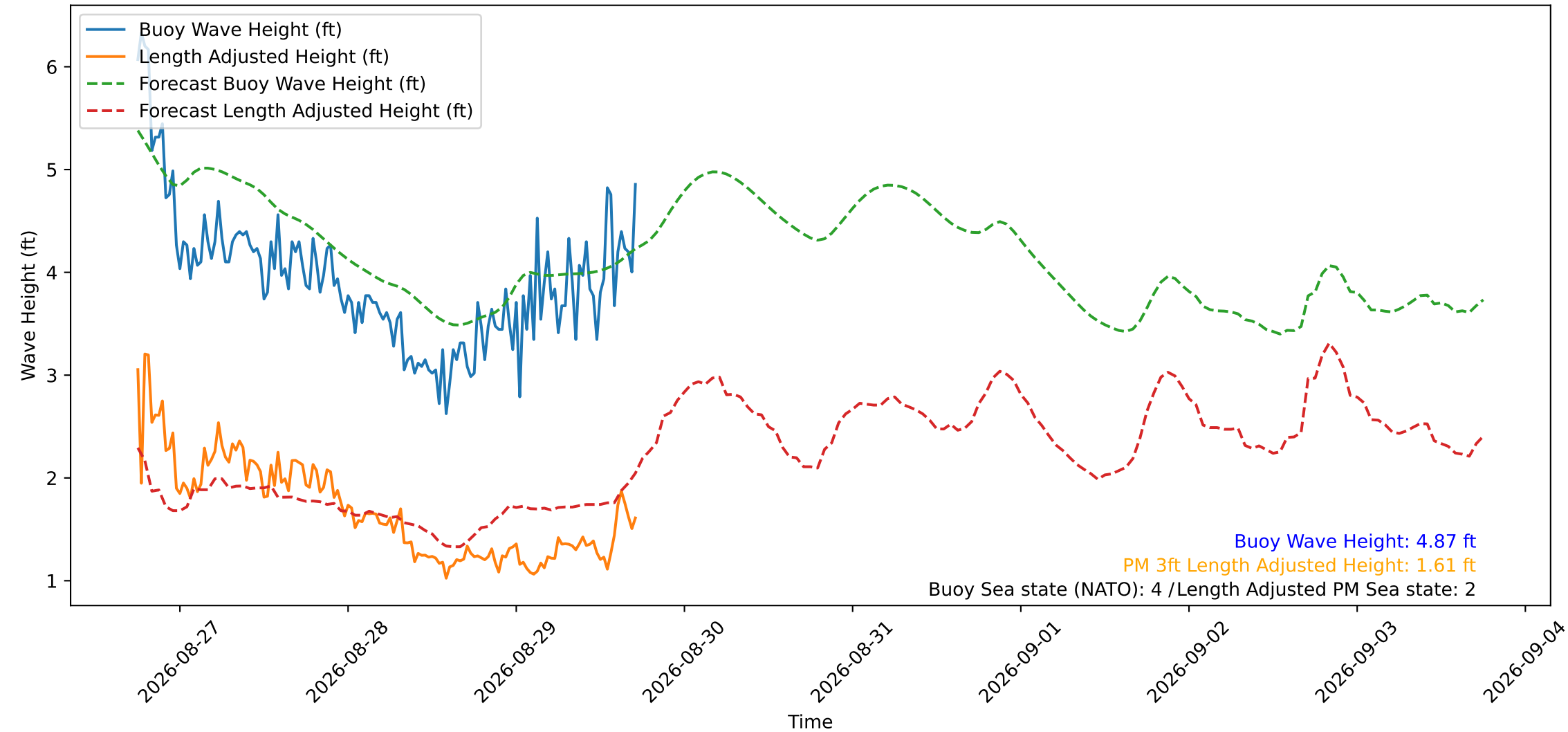
Wave Heights over Time for Green Beach at 2026-08-29 17:41:12
