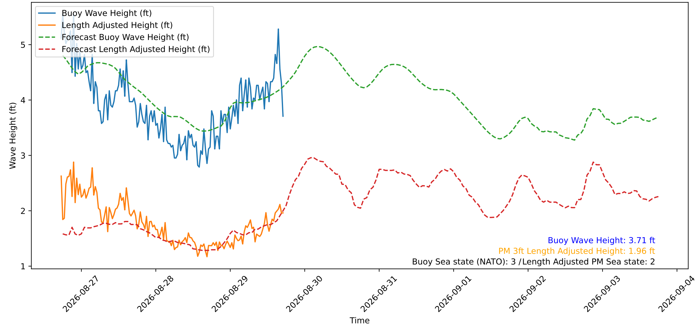
Wave Heights over Time for Oceanside Harbor at 2026-08-29 17:40:29
