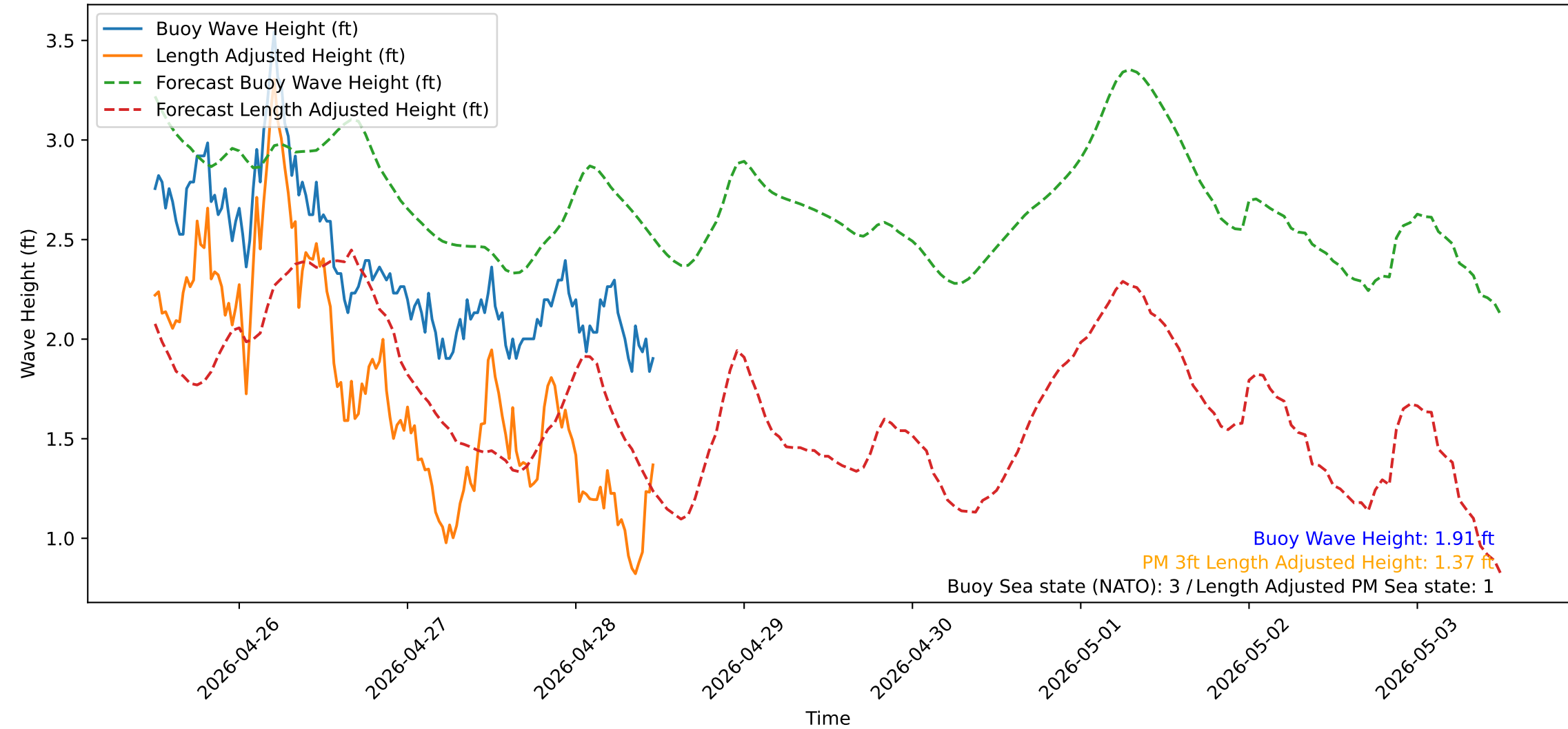
Wave Heights over Time for Red Beach at 2026-04-28 11:40:50
