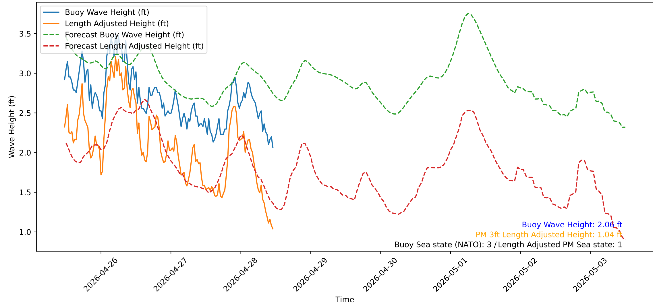
Wave Heights over Time for Green Beach at 2026-04-28 11:41:13
