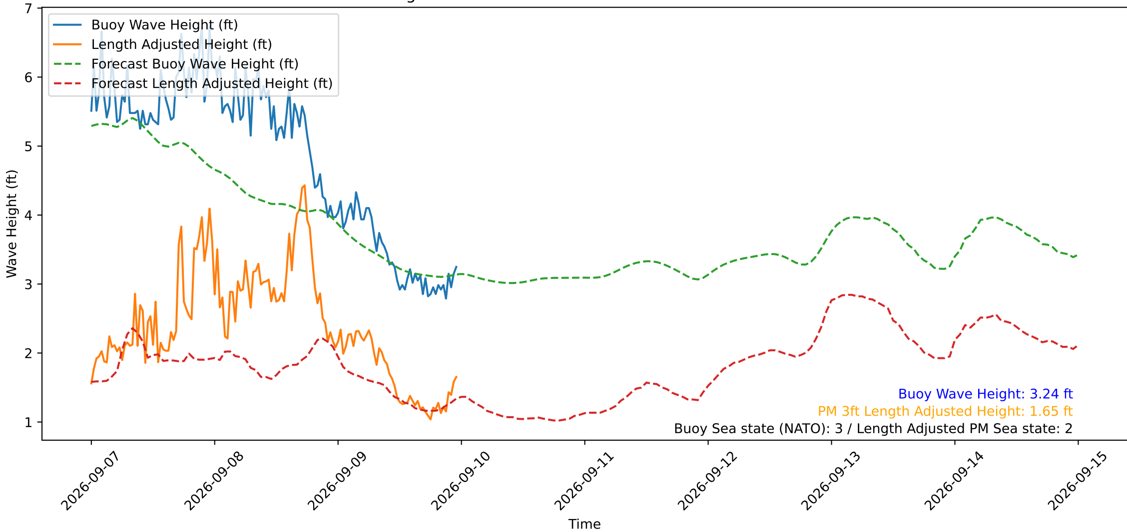
Wave Heights over Time for Red Beach at 2026-09-09 23:40:49
