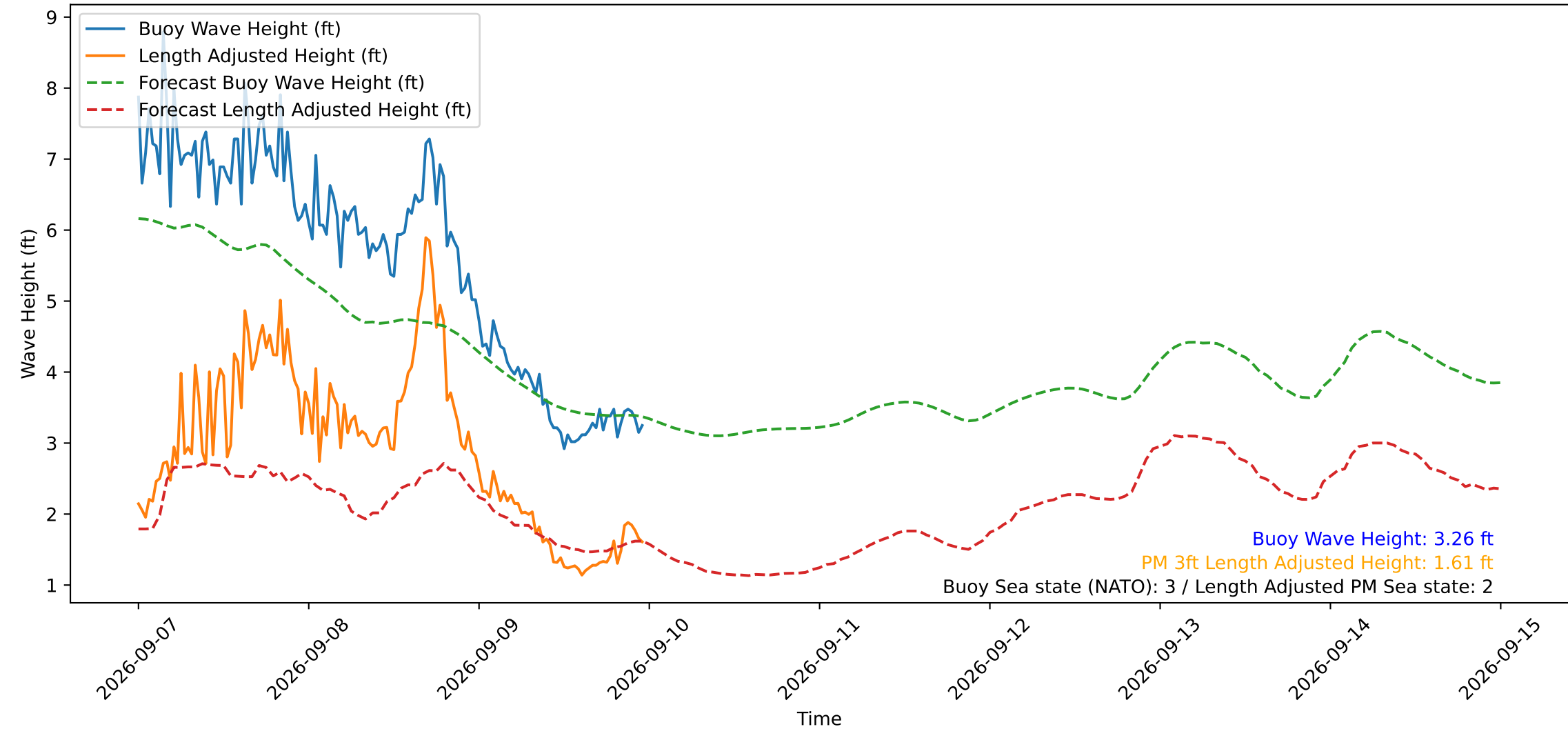
Wave Heights over Time for Green Beach at 2026-09-09 23:41:11
