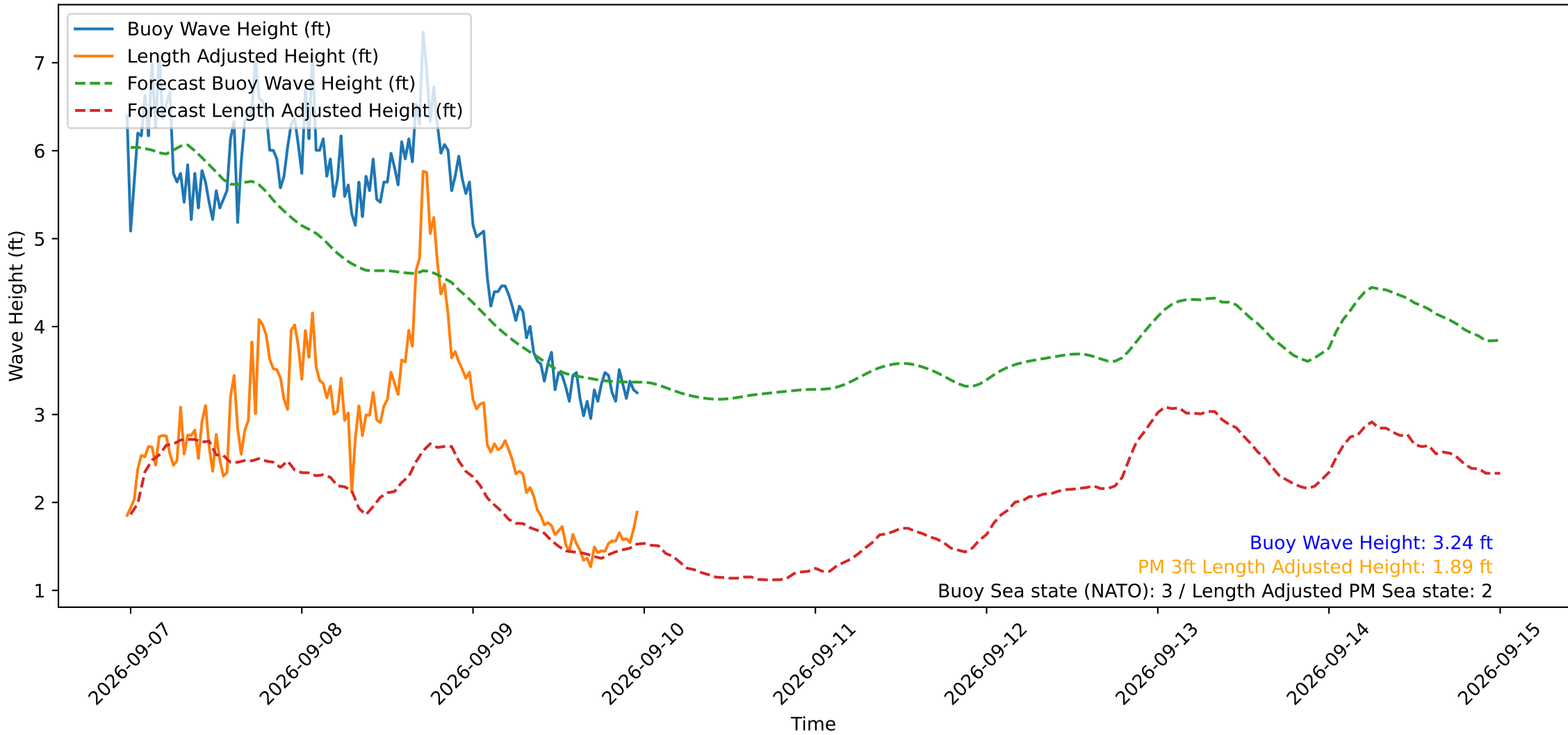
Wave Heights over Time for Oceanside Harbor at 2026-09-09 23:40:29
