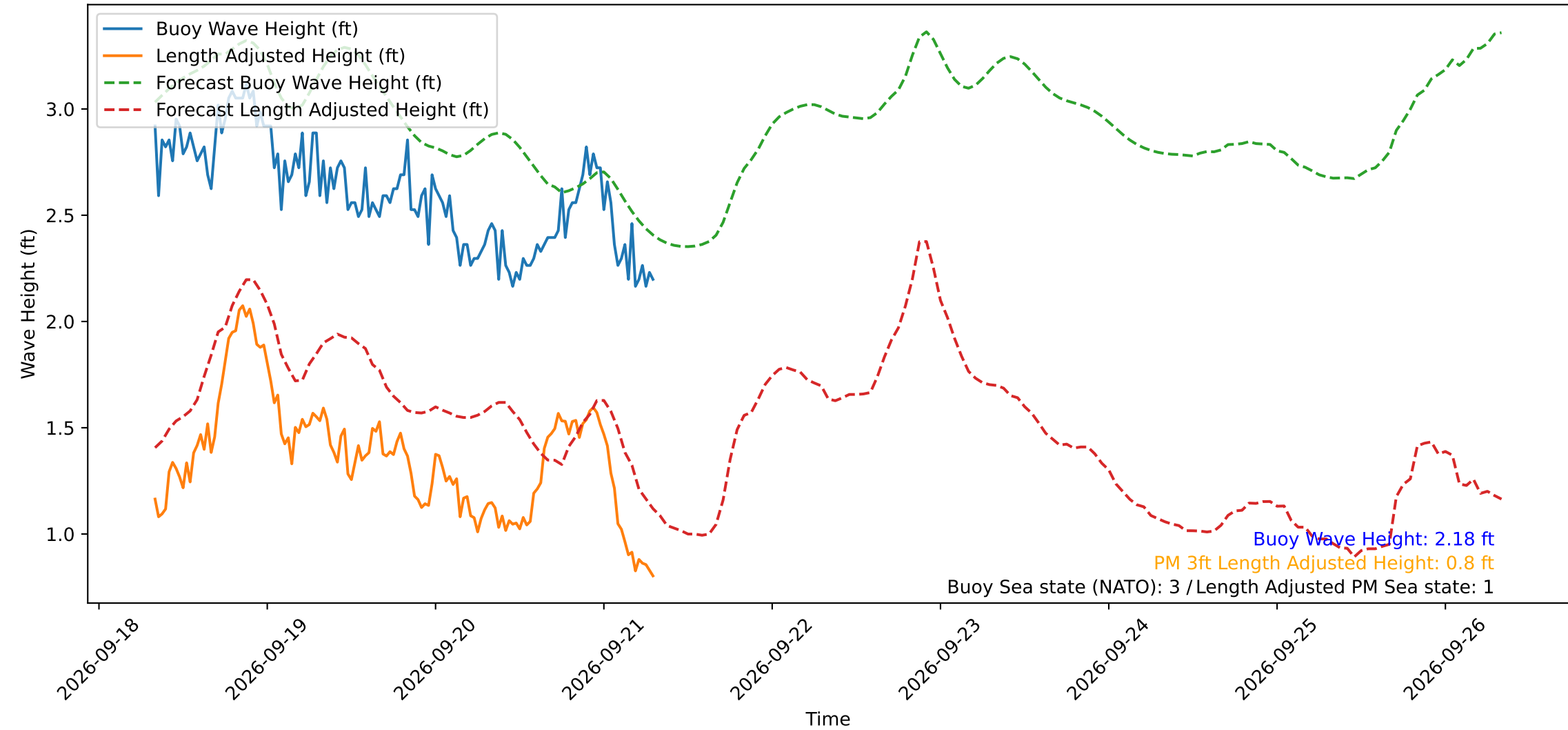
Wave Heights over Time for Green Beach at 2026-09-21 07:41:11
