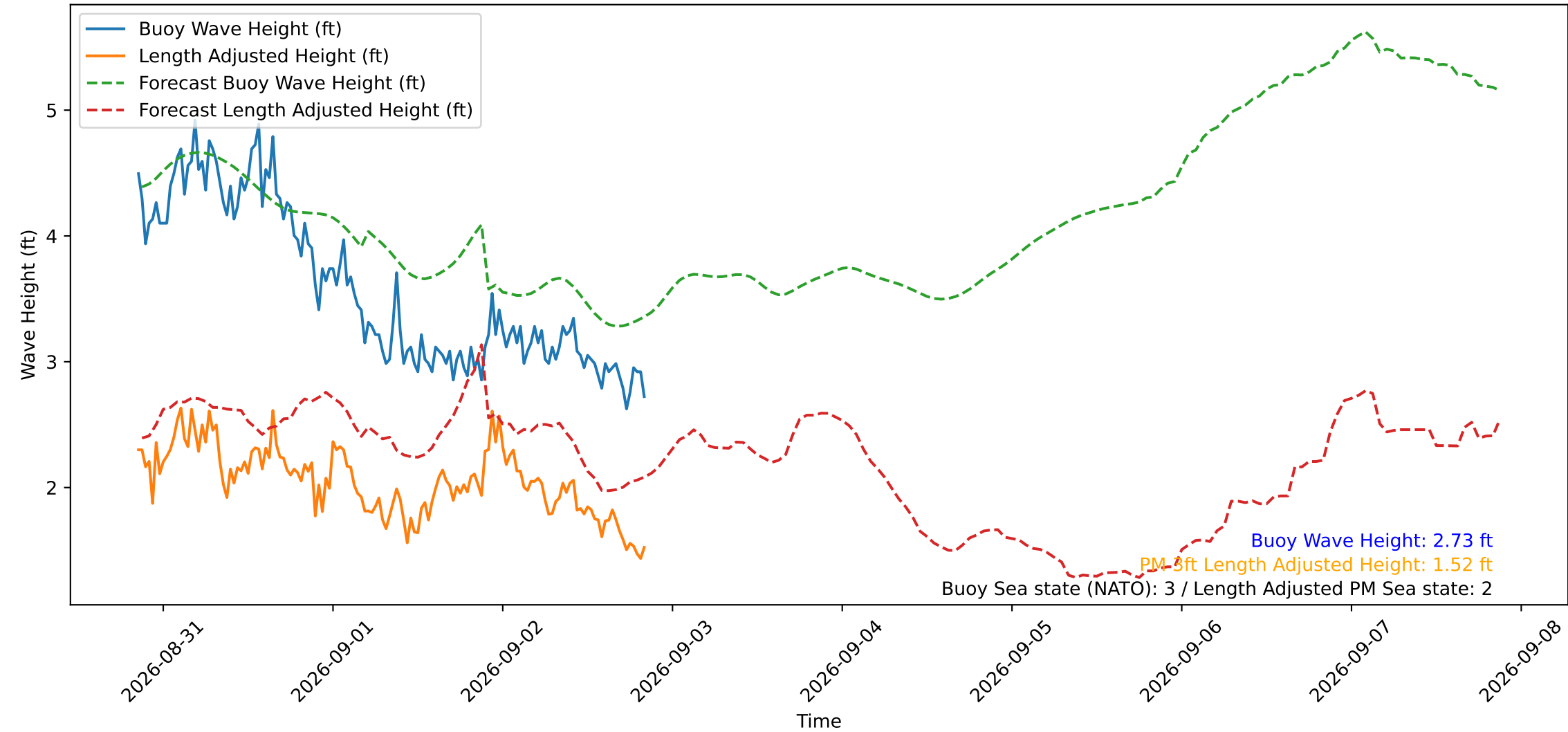
Wave Heights over Time for Oceanside Harbor at 2026-09-02 20:30:30
