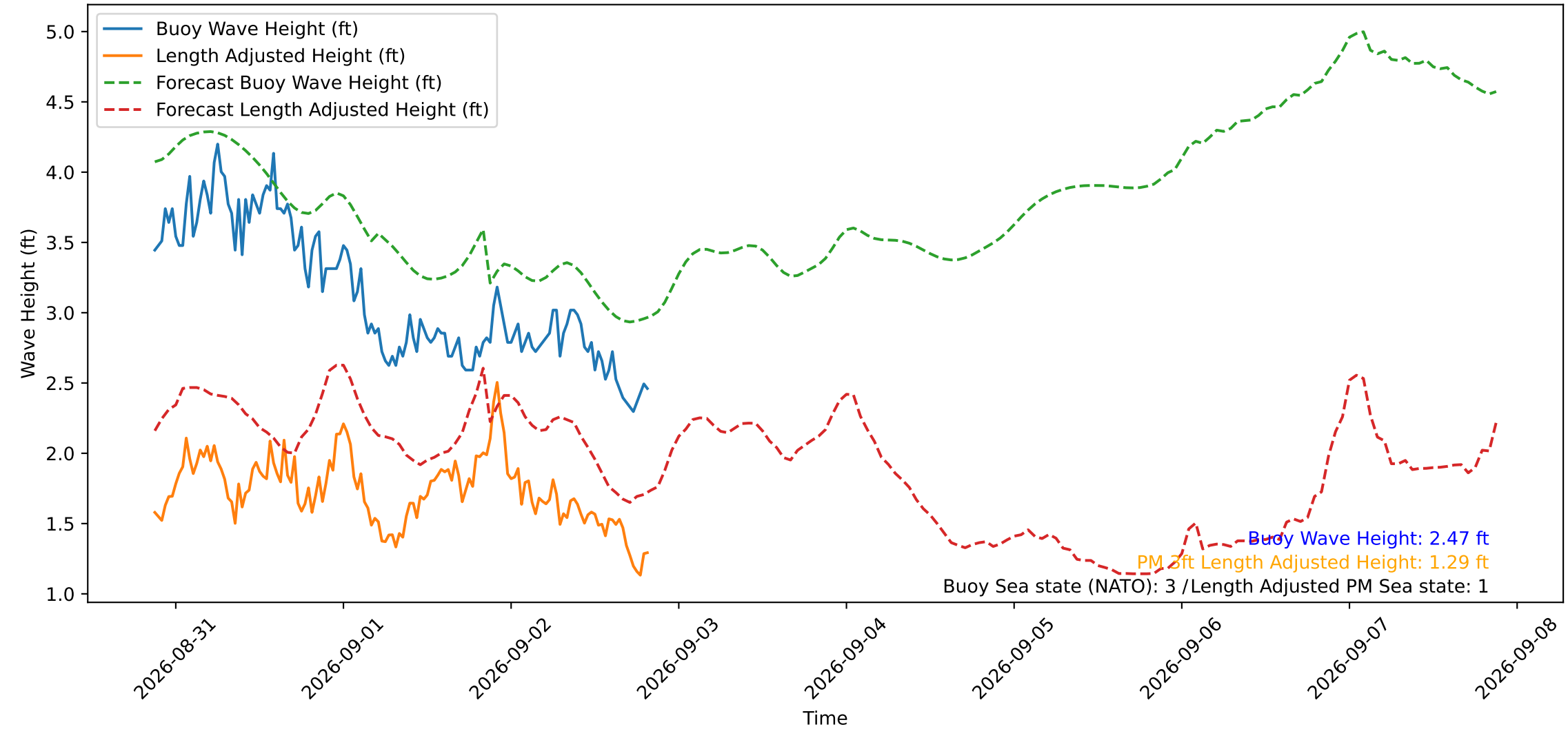
Wave Heights over Time for Red Beach at 2026-09-02 20:30:50
