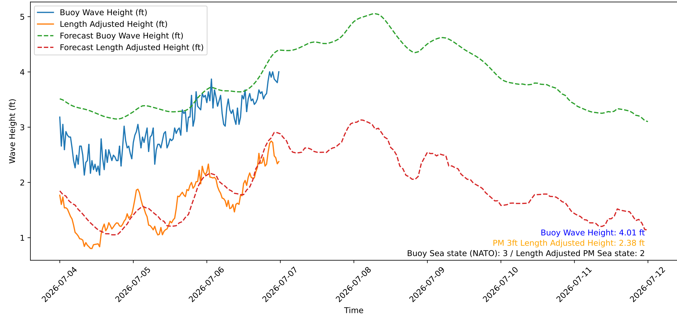
Wave Heights over Time for Oceanside Harbor at 2026-07-07 00:00:26
