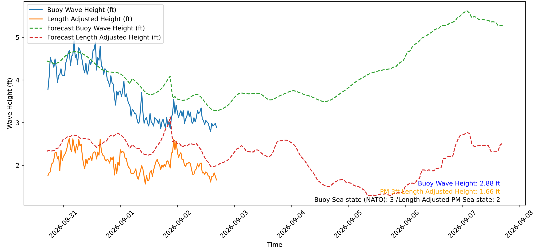
Wave Heights over Time for Oceanside Harbor at 2026-09-02 17:20:30
