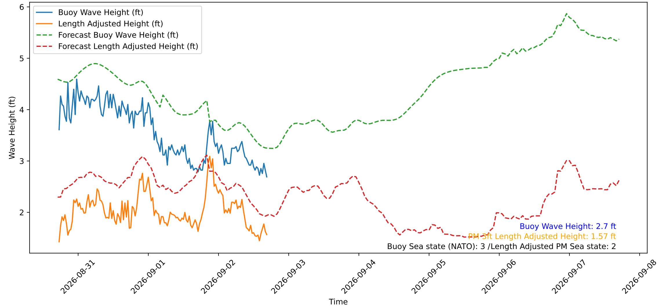
Wave Heights over Time for Green Beach at 2026-09-02 17:21:15
