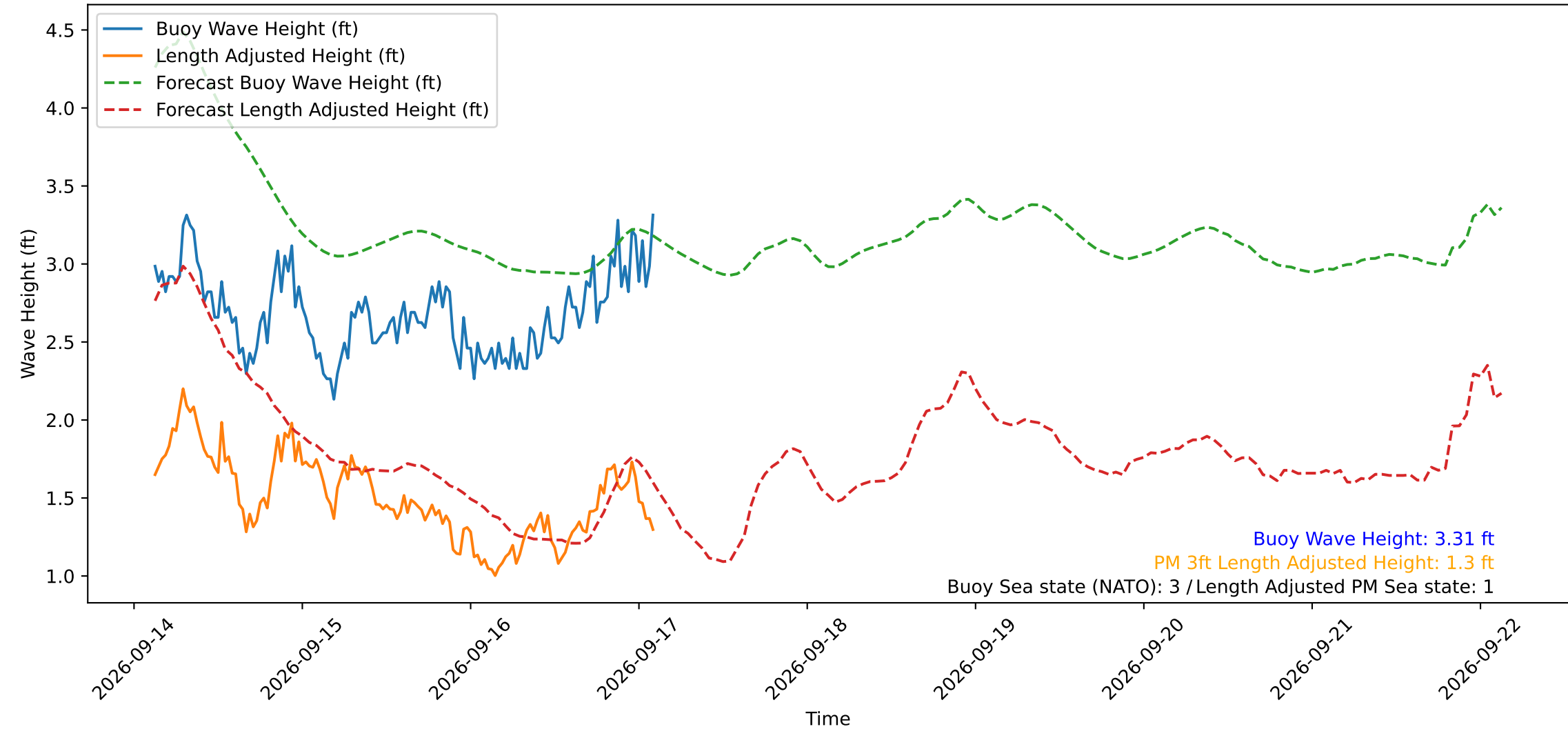
Wave Heights over Time for Green Beach at 2026-09-17 02:41:11
